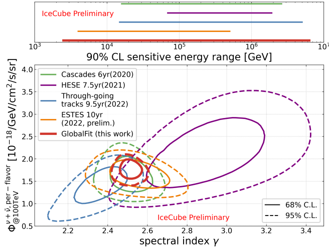
Figure 1: Result of the combined fit of tracks and cascades (in red) under the assumption of an astrophysical SPL neutrino flux. Previous results from measurements using single event channels are shown for comparison. Note that the sensitive neutrino energy ranges (as indicated in the upper panel) and neutrino flavor probed are different amongst the different samples.
