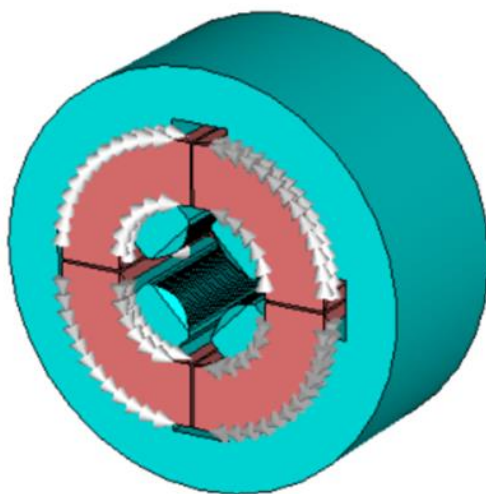
Figure 1: 3D diagram of the quadrupole magnet type A.
