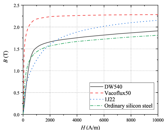
Figure 2: Comparison of the BH curves for soft magnetic alloy and ordinary silicon steel.
