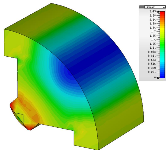
Figure 4: B field in the yoke of type A magnet.
