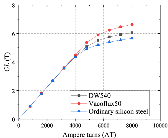
Figure 3: Quadrupole saturation of type A magnet with different yoke materials.
