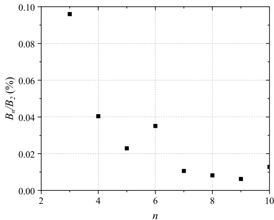
Figure 6: Values of the various multipole normalized with quadrupole strength.
