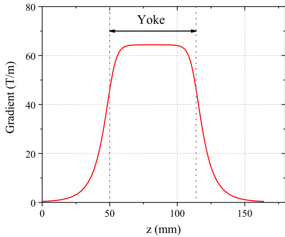
Figure 5: Gradient along the beam axis of type A magnet with the excitation current of 4450 AT.
