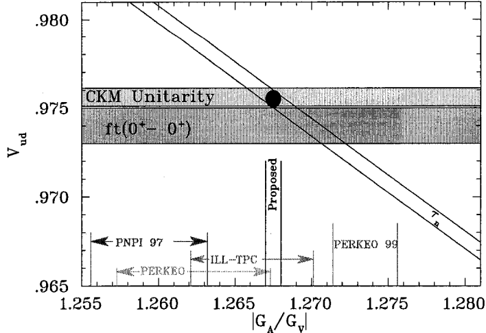
FIG. 6: Projected accuracy of neutron lifetime (diagonal band labeled \tau_n ) and beta asymmetry measurements in future LANSCE experiments (horizontal band labeled “Proposed”). Together, these measurements will provide a measurement of V_{ud} . Also shown are the experimental uncertainties on other measurements of |G_A/G_V| .
