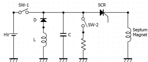
Figure 10: Circuit architecture of the septum magnet.
