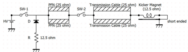
Figure 9: Equivalent circuit of the kicker magnet power supply.
