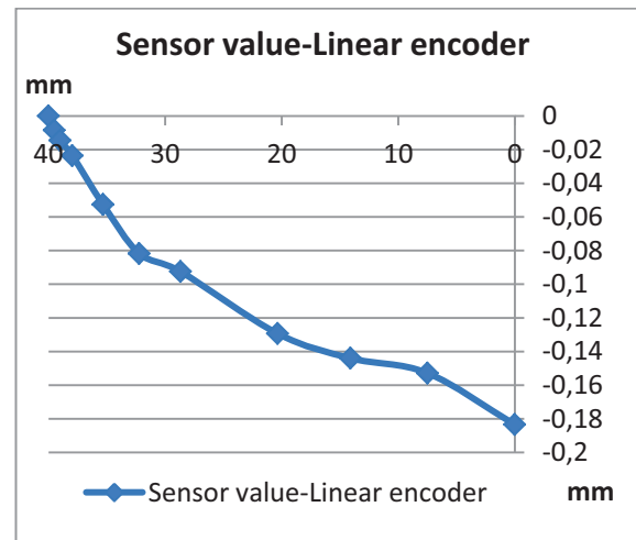
Figure 6: Receiver sensor compensated value.
