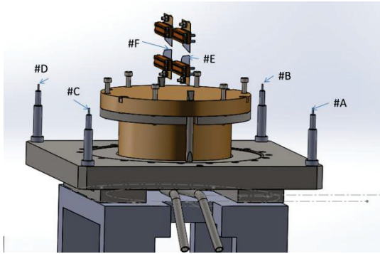
Figure 7: Measurement data locations.
