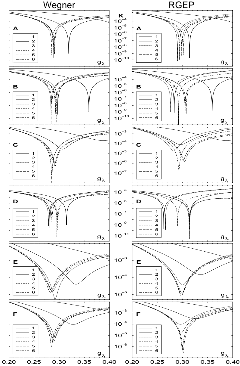
Fig. 6. The functions K(g_\lambda) from Eqs. (16) to (21) plotted for Wegner and RGEP cases, \lambda = 2 GeV. In all cases a preferred value of g_\lambda is clearly identified. These are given in Table I.
