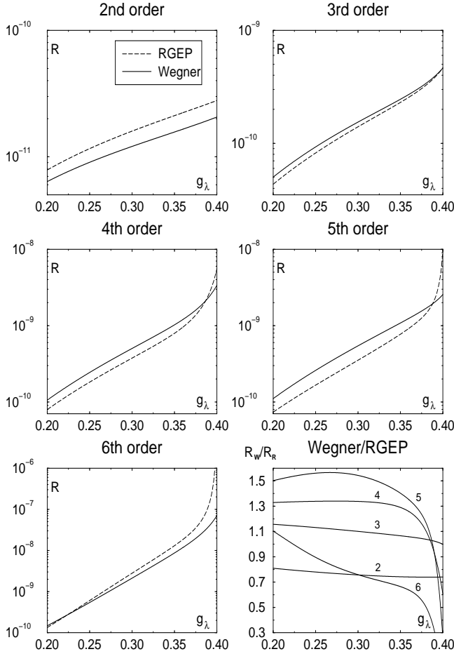
Fig. 5. Plots of the renormalizability measure R(g_\lambda) from Eq. (22) for the RGE procedure (dashed lines) and the altered Wegner equation (solid line). The last diagram displays the ratios R_W/R_R (with R_W standing for the benchmark R , and R_R for the R in the RGE procedure), and the integer labels indicate the corresponding orders of the weak-coupling expansion.
