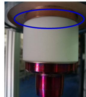
Figure 2: Vacuum leakage of cold ceramic window caused by argon plasma.
