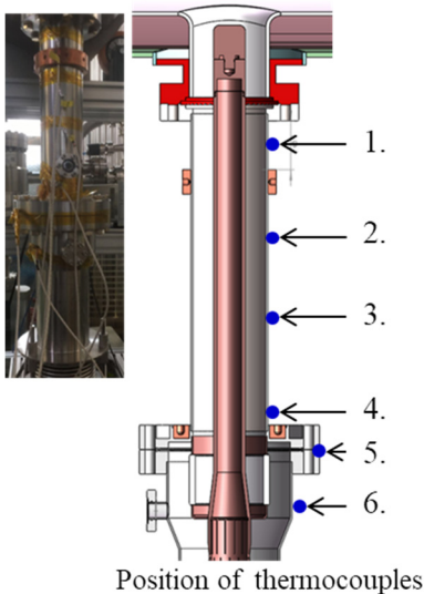
Figure 3: Schematic diagram of thermocouples on the coupler.
