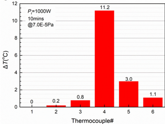
Figure 4: Temperature variation of coupler surface after the argon plasma discharge.
