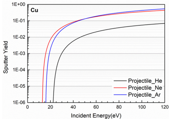
Figure 6: Sputter yield of copper by He/Ne/Ar ions as the function of incident energy.
