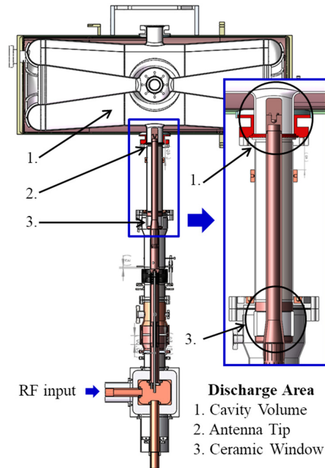
Figure 1: HWR015 assembled with coupler for plasma online ignition.
