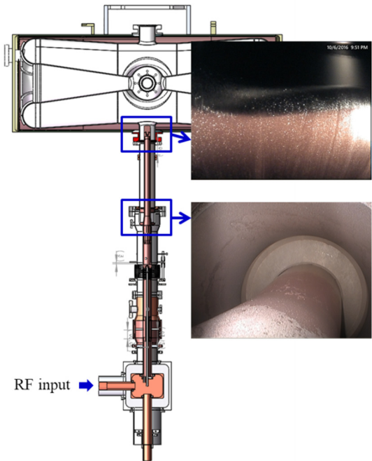
Figure 5: Visual inspection by optical camera.
