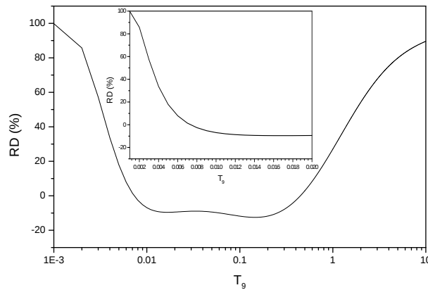
Fig. 6. {}^2\text{H}(d,p){}^3\text{H} : The variation of the relative difference RD between the new and the old REACLIB rates with respect to temperature ( n = 5\% ).
