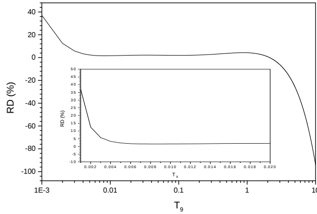
Fig. 10. {}^3\text{He}(\alpha, \gamma){}^7\text{Be} : The variation of the RD between the old and the new REACLIB rates with respect to temperature ( n = 6\% ).
