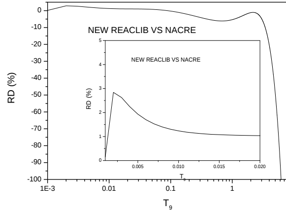
Fig. 12. {}^6\text{Li}(p, \gamma){}^7\text{Be} : The variation of the RD between the new REACLIB rate and the NACRE one with respect to temperature ( n = 7\% ).
