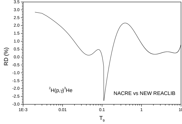
Fig. 3. {}^2\text{H}(p, \gamma){}^3\text{He} : The variation of the relative difference RD between the new REACLIB rates and the NACRE ones with respect to temperature ( n = 3\% ).
