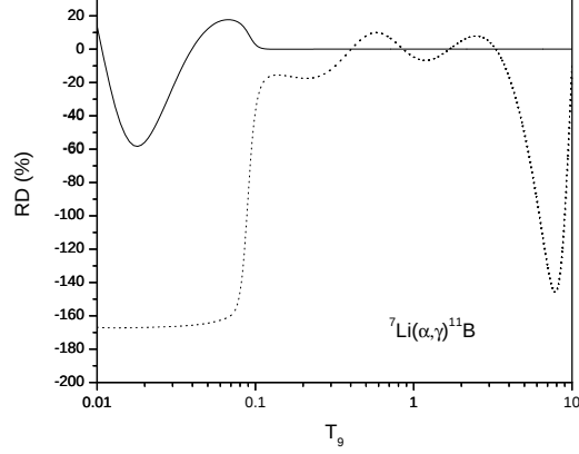
Fig. 16. {}^7\text{Li}(\alpha, \gamma){}^{11}\text{B} : The variation of the RD between the old (solid curve)/new (dotted curve) REACLIB rates and the NACRE one with respect to temperature ( n = 17\% ).
