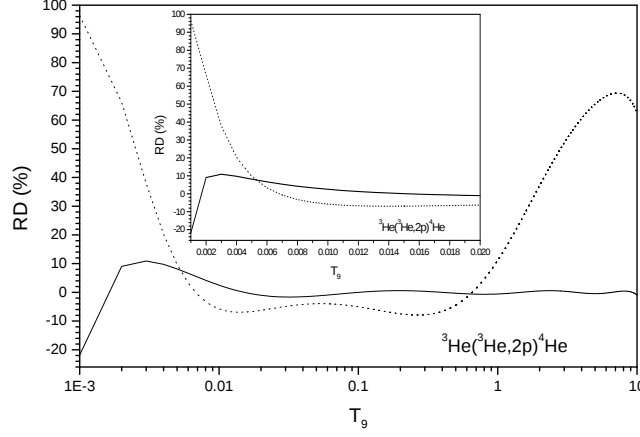
Fig. 7. {}^3\text{He}({}^3\text{He}, 2p){}^4\text{He} : The variation of the relative difference RD between the (old/new) REACLIB rates and that obtained by using the LUNA data with respect to temperature. The solid (dotted) curve represents the RD between the new (old) REACLIB rate and the LUNA one.
