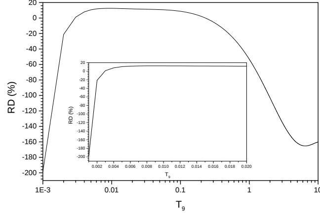
Fig. 4. {}^2\text{H}(d, \gamma){}^4\text{He} : The variation of the relative difference RD between the new and old REACLIB rates with respect to temperature ( n = 3\% ).
