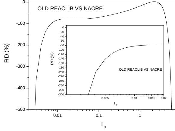
Fig. 11. {}^6\text{Li}(p, \gamma){}^7\text{Be} : The variation of the RD between the old REACLIB rate and the NACRE one with respect to temperature ( n = 7\% ).
