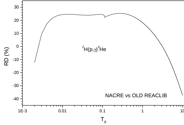
Fig. 2. {}^2\text{H}(p, \gamma){}^3\text{He} : The variation of the relative difference RD between the old REACLIB rates and the NACRE ones with respect to temperature ( n = 3\% ).
