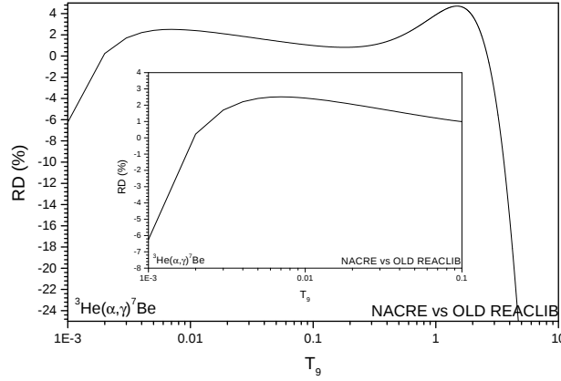
Fig. 9. {}^3\text{He}(\alpha, \gamma){}^7\text{Be} : The variation of the RD between the old REACLIB rate and the NACRE one with respect to temperature ( n = 6\% ).
