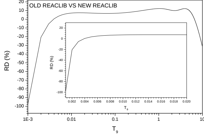
Fig. 13. {}^6\text{Li}(p, \alpha){}^3\text{He} : The variation of the RD between the old REACLIB rate and the new one with respect to temperature (2%).
