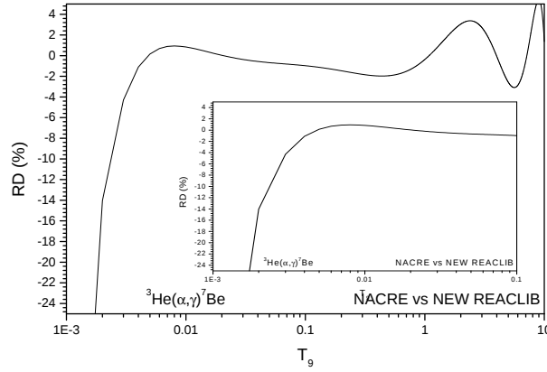
Fig. 8. {}^3\text{He}(\alpha, \gamma){}^7\text{Be} : The variation of the RD between the new REACLIB rate and the NACRE one with respect to temperature ( n = 6\% ).
