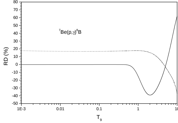
Fig. 18. {}^7\text{Be}(p, \gamma){}^8\text{B} : The variation of the RD between the new REACLIB rate and the NACRE one (solid curve) and the variation of the RD between the old and the new REACLIB rates (dotted curve) ( n = 3\% ).
