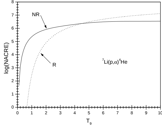
Fig. 14. {}^7\text{Li}(p, \alpha){}^4\text{He} : The logarithms of the NACRE rates (resonant and non-resonant) with respect to temperature (6%).
