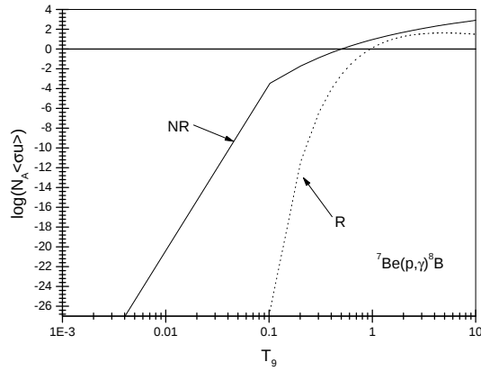
Fig. 17. {}^7\text{Be}(p, \gamma){}^8\text{B} : The logarithms of the NACRE rates (resonant, non-resonant and multiresonant) with respect to temperature ( n = 3\% ).
