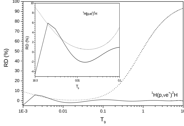
Fig. 1. {}^1\text{H}(p, \nu e^+){}^2\text{H} : The variation RD(%) of the relative difference between the REACLIB rates and the values obtained by numerical integration of Eq. (2) using the NACRE data. The solid curve represents the RD between the new REACLIB rate and the NACRE one while the dotted one represents the RD between the old REACLIB rate and the NACRE one ( n = 3\% ).
