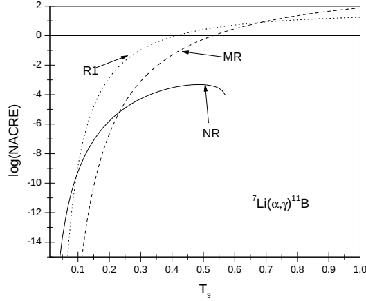
Fig. 15. {}^7\text{Li}(\alpha, \gamma){}^{11}\text{B} : The logarithms of the NACRE rates (resonant, non-resonant and multiresonant) with respect to temperature ( n = 17\% ).
