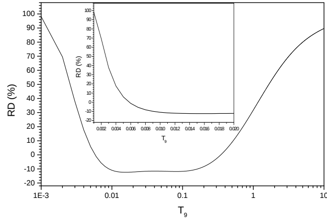
Fig. 5. {}^2\text{H}(d, n){}^3\text{He} : The variation of the relative difference RD between the new and old REACLIB rates with respect to temperature ( n = 4\% ).
