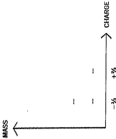
FIG. 4. Hypothetical Quarks.
