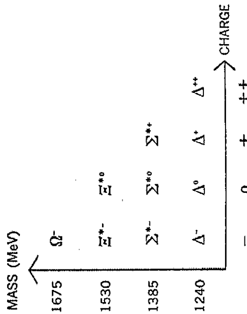
FIG. 2. Baryon Decimet ( J=3/2^+ ).
