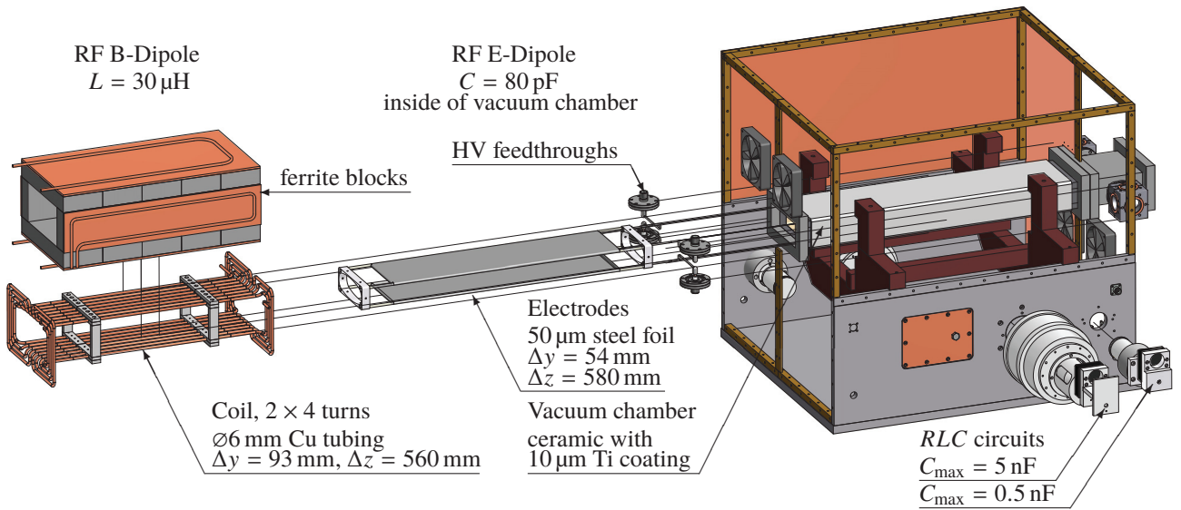
Figure 1: An explosion drawing showing the main components of the RF ExB-Dipole.
