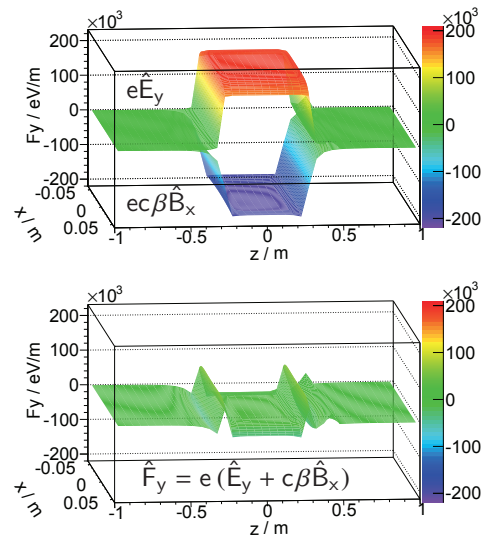
Figure 2: Simulation of the Lorentz-Force on a particle entering the RF ExB-Dipole on axis across a horizontal cut through the center of the beam pipe. The results have been normalized to a coil current amplitude of \hat{I} = 1 A.
