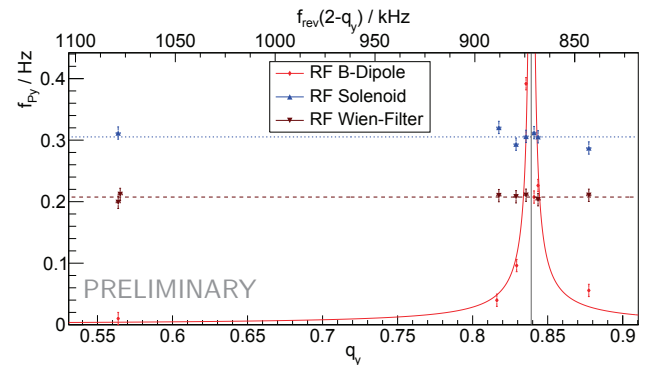
Figure 5: Results of the resonance scans at the nominal tune of COSY at Q_y = 3.56 and for a set of vertical betatron tunes with sideband frequencies around the spin resonance, depicted by the vertical line at 871 428.00 Hz.
