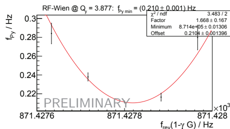
Figure 4: Polarization oscillation frequencies from a series of runs with varying excitation frequencies. The points form the tip of the spin resonance curve.
