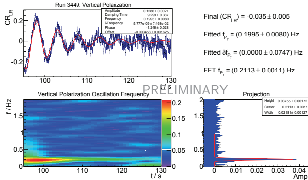
Figure 3: The top panel shows the driven oscillation of the vertical polarization component in case of excitation close to the spin resonance. The bottom panels show the frequency content of the signal determined by FFT analysis, resolved over time to detect fluctuations on the left and integrally over the whole run on the right.
