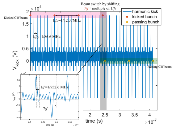
Figure 5: The alternating operation of two CW beams. The harmonic kick profile is with base frequency of 86.6 MHz using five odd harmonics. The profile has 10 zero kick locations spaced by 1/f .
