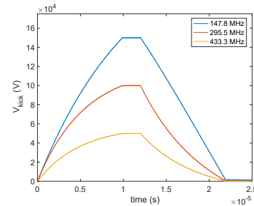
(a) The kick voltage within the kicker cavity with the optimized \beta 's.
