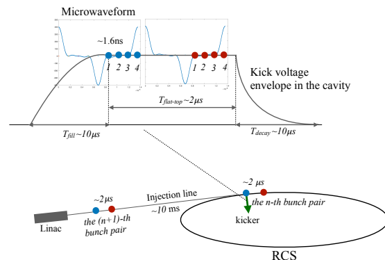
Figure 1: The schematics of the RCS illustrating the injection scheme. The microwaveforms are near zero on passing (1,2,3) pairs while peaked on the injected pair (4).
