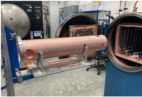
Figure 4: The harmonic kicker prototype in fabrication.
