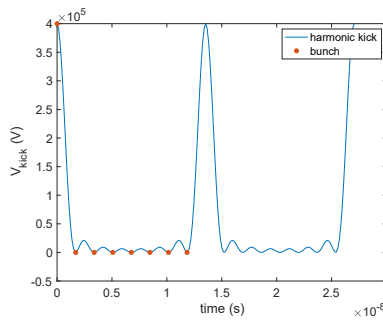
(b) The 8 bunch train scheme.
