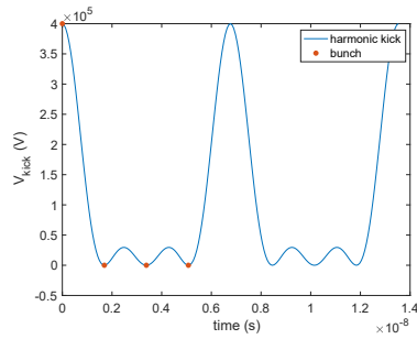
(a) The 4 bunch train scheme.
