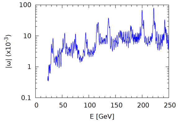
Figure 4: Coherent part of the ST-resonance strength in RHIC as a function of energy.
