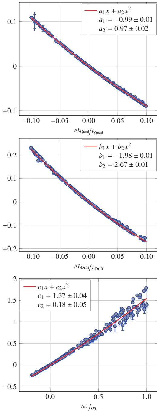
Figure 2: Dependency of emittance errors on measurement errors. From top to bottom: Influence of relative errors of the quadrupole strength, the drift length and the measured beam size.
