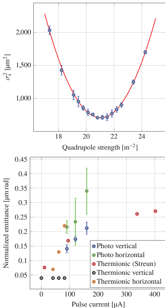
Figure 3: Top: Quadrupole scan of a continuous 20 nA beam at 3.5 MeV. The results show statistical errors of the beam size measurement in the order of a few \mu\text{m} . The normalized emittance of the displayed data set is (40.0 \pm 2.4) \text{ nm rad} . Bottom: Collection of measured emittances at the MAMI accelerator using a pulsed beam. The graph displays the results of the experiment and compares them to an old data set taken by A. Streun in the year 1986 at 100 keV using a continuous beam [6].
