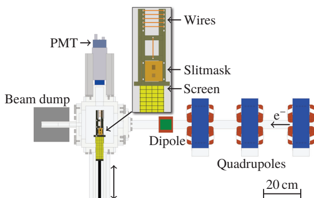
Figure 1: Schematic view of the set-up. The experiment lies behind the 3.5 MeV pre-accelerator of MAMI. The detail view is a close-up of the scanner as seen from the beam direction.
