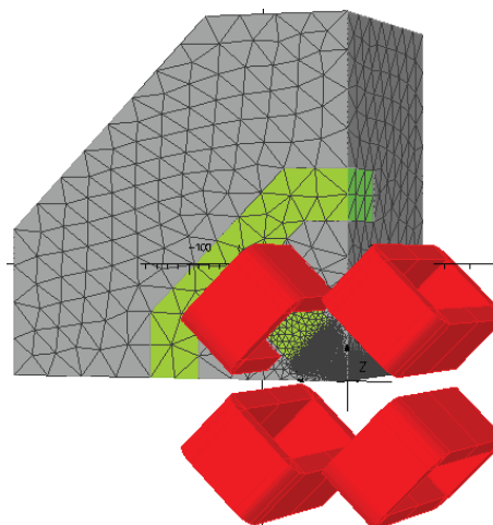
Figure 6: 3D design of the booster quadrupole magnet created in OPERA.
