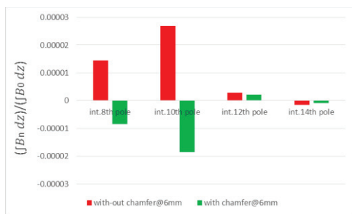
Figure 4: Normalized integrated multipole errors at 6 mm in dipole sections.
