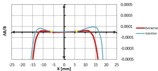
Figure 3: Field quality of the BR dipole sections within \pm 6 mm GFR at injection and extraction.
