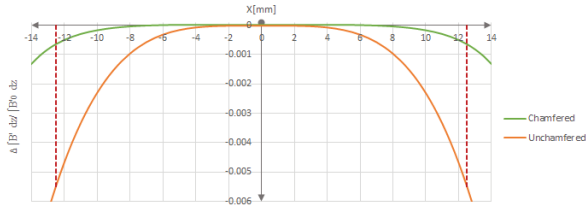
Figure 8: Integrated field quality of the booster quadrupole magnet in the y=0 plane with and without chamfer.
