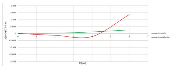
Figure 5: Integrated field quality of the booster dipole magnet in the y=0 plane with and without chamfer.
