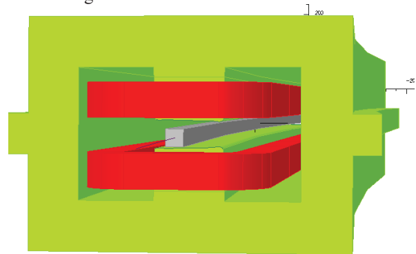
Figure 2: 3D design of the booster dipole magnet created in OPERA simulation code.
