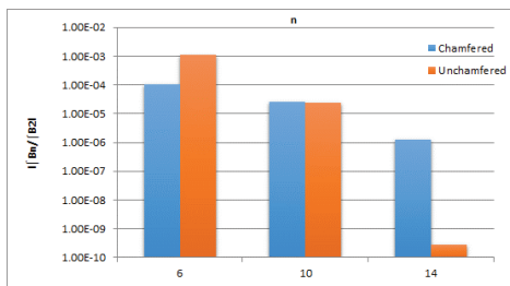
Figure 9: Absolute normalized integrated multipoles' errors at 12.5 mm GFR with (blue) and without (orange) chamfer.
