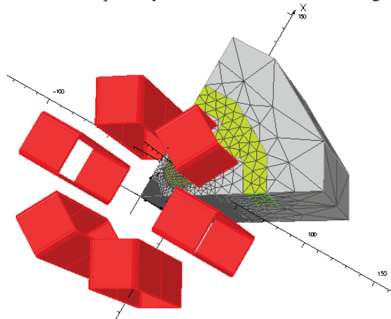
Figure 10: 3D design of the booster sextupole with meshed regions.
