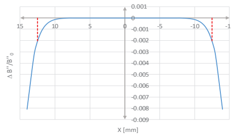
Figure 11: Field quality of the booster sextupole within \pm 12.5 mm GFR.
