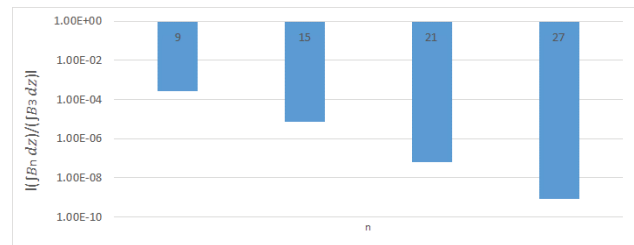
Figure 12: Absolute normalized integrated multipoles' errors at 12.5 mm GFR.
