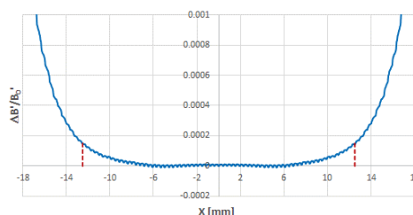
Figure 7: Field quality of the booster quadrupole within \pm 12.5 mm GFR.
