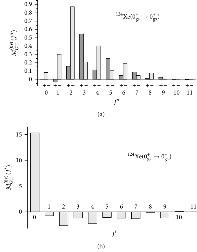
FIGURE 12: Decompositions of (37) in J^\pi (a) and J' (b) for the ground-state Gamow-Teller NME M_{GT}^{(0v)}(0_{gs}^+) of ^{124}\text{Xe} . Results for the Jastrow short-range correlations are shown with g_A = 1.25 .
