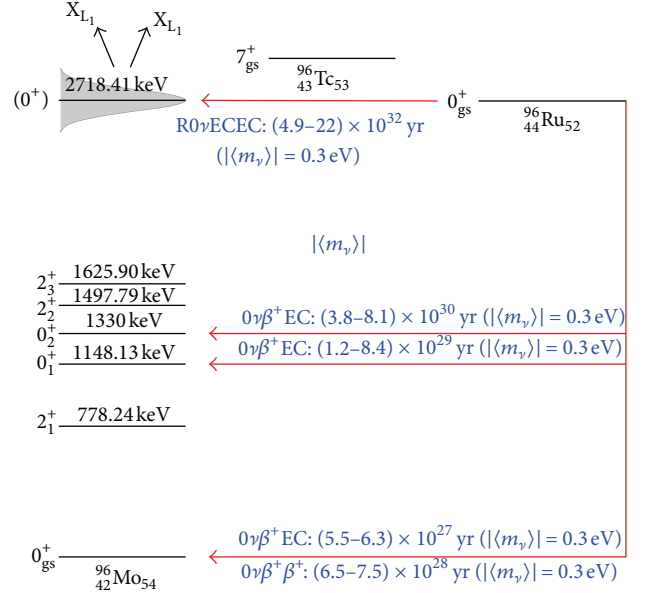
FIGURE 6: Computed partial 0\nu\beta^+/\text{EC} decay half-lives of the various decay transitions from ^{96}\text{Ru} . The value m_{\text{eff}} = 0.3 \text{ eV} is adopted for the effective neutrino mass and the UCOM short-range correlations have been assumed. The half-lives are given in units of years.
