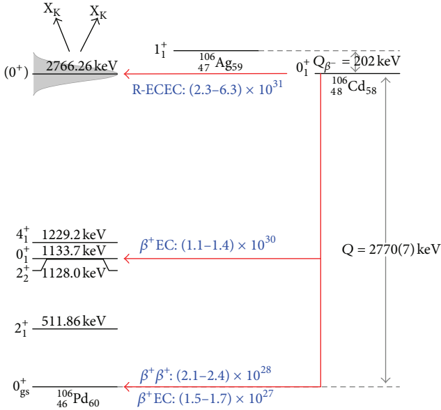
FIGURE 5: Computed partial 0\nu\beta^+/\text{EC} decay half-lives of the various decay transitions from ^{106}\text{Cd} . The value m_{\text{eff}} = 0.3 \text{ eV} is adopted for the effective neutrino mass and the UCOM short-range correlations have been assumed. The half-lives are given in units of years.
