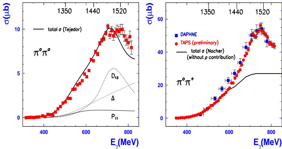
Fig. 1. Total cross section as a function of incident photon energy for \pi^0\pi^0 (left) and \pi^0\pi^+ production (right) off the proton. The lines correspond to models (see text). On the upper horizontal axis center-of-momentum energies are indicated. The figures are taken from Wolf et al. [9] and Langgärtner et al. [10].
