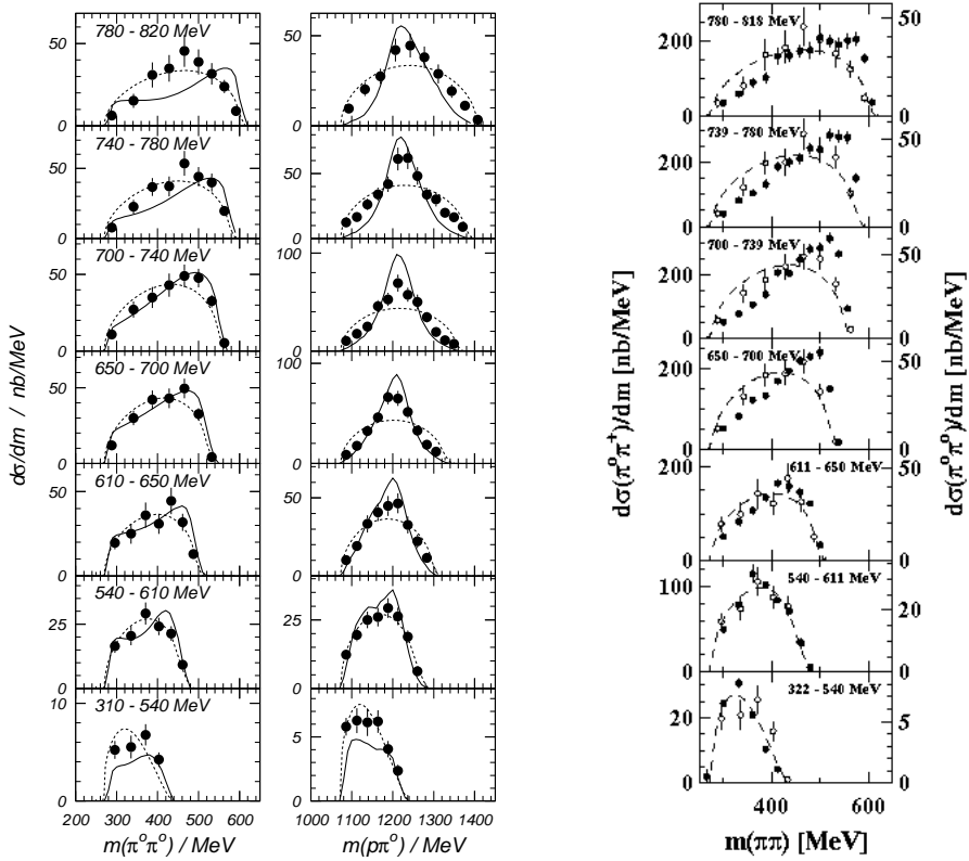
Fig. 2. Left: comparison of \pi^0\pi^0 and p\pi^0 mass distributions to pure phase space (dashed line) and model calculations [14]; right: comparison of \pi^0\pi^0 and \pi^0\pi^+ invariant mass distributions (dashed line: phase space).
