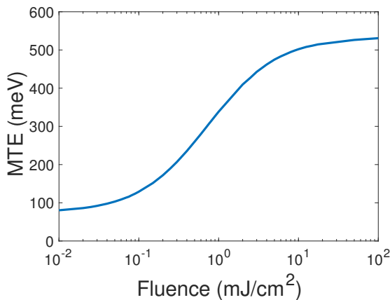
Figure 3: MTE calculated from Eq. (2) for a wide range of laser fluences for 265 nm. The MTE increases by a factor of 3 to 4 in the fluence regime ( 10^{-1} mJ/cm 2 to 10^2 mJ/cm 2 ) typically used in photoinjectors. This dramatic increase can be attributed to nonlinear effects.
