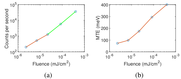
Figure 2: (a) The electron counts per seconds as a function of fluence for 280 nm. The shift from the red slope to the green slope at 2.18 \times 10^{-5} \text{ mJ/cm}^2 is due to the transition between linear and nonlinear emission. (b) MTE as a function of fluence for 280 nm. We see that the MTE increases as the emission transitions from linear to nonlinear.
