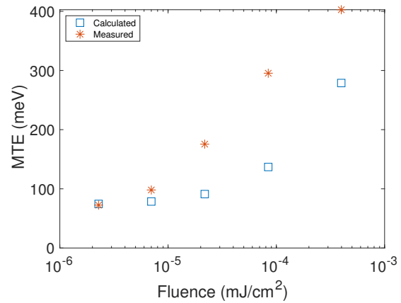
Figure 4: Comparison of the measured MTE for 280 nm (red stars) and the MTE calculated (blue squares) using Eq. (2) to determine the accuracy of this extrapolation. We see that it provides a lower limit and becomes less accurate with increasing fluence.
