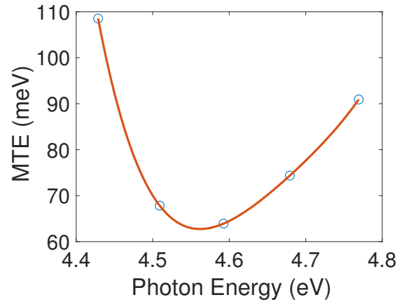
Figure 1: MTE measured for several wavelengths around the photoemission threshold for a laser fluence of 10^{-7} \text{ mJ/cm}^2 . From the fitted curve we see the minimum value of the MTE occurs at approximately the same energy as the measured work function. MTE increases below threshold due to effects of nonlinear photoemission.
