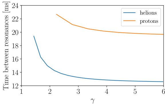
Figure 1: Imperfection resonance spacing for protons and helions.
