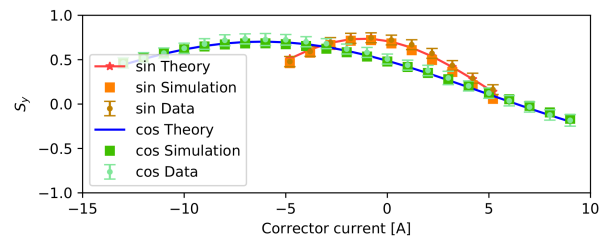
Figure 3: Harmonic scan of protons crossing |G\gamma| = 3 with a comparison between theory, simulations, and experimental data.
