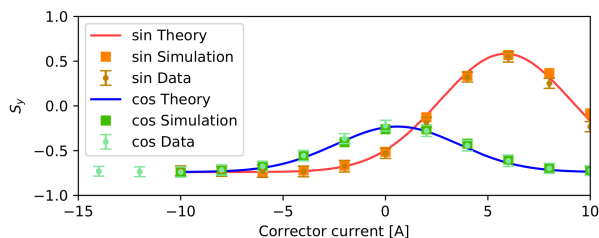
Figure 4: Harmonic scan of protons crossing |G\gamma| = 4 with a comparison between theory, simulations, and experimental data.
