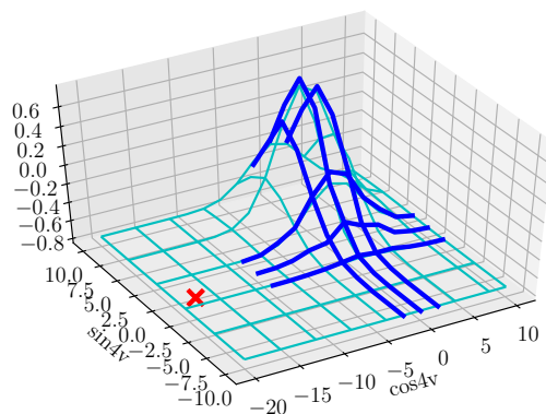
Figure 5: Harmonic scan of protons crossing the |G\gamma| = 4 resonance with initial currents at [-2, 0, 2] for the sine and cosine components. Dark blue lines are resulting simulation data. The light blue surface grid is reconstructed by fitting to the experimental data and extrapolating it to a larger range. The red 'X' marks corrector currents used in Run17, [\sin 4v, \cos 4v] = [0, -18] .
