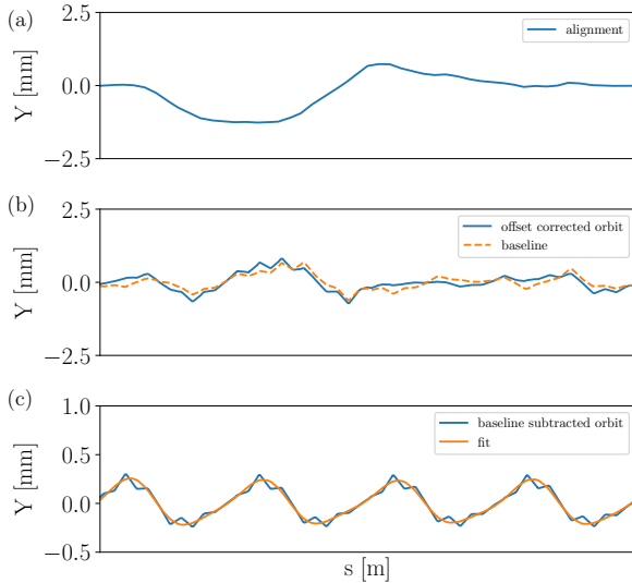
Figure 2: a) Vertical quadrupole misalignments in the Booster are scaled to 65% to match h=4 data, Fig. 4; b) Orbit after incorporating misalignments; c) Baseline subtracted orbit for helions crossing the |G\gamma| = 8 resonance where harmonic correction is the same except the baseline orbit has \sin 4v=6.97 A and the other has \sin 4v=5.22 A. This example has a corrector current with respect to h=8 of \cos 8v=5 A, \sin 8v=13 A. The components of the fit results are: [\sin 4, \cos 4, \sin 5, \cos 5, \sin 8, \cos 8]=[0.1997 mm, 0.07796 mm, 0.01137 mm, 0.00031849 mm, -0.01263 mm, -0.04177 mm].
