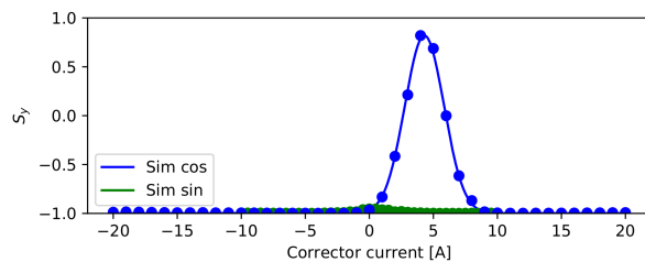
Figure 6: Helions crossing the |G\gamma| = 5 resonance. Correction of harmonic is insufficient and needs to be enhanced to spin-flip. To correct the orbit harmonic h=4 , [\sin 4, \cos 4] = [2.797, 0.669] and to spin-flip: h=5 currents are [\sin 5, \cos 5] = [10.0, -18.0] and I_{\max} = 23.086 .
