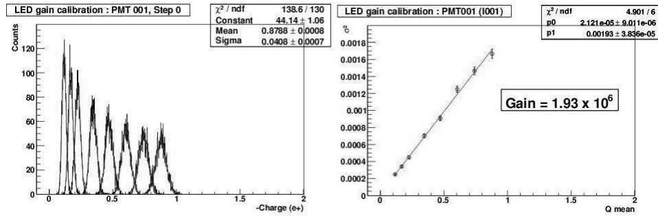
Figure 4. Example of a gain fit for a photomultiplier
