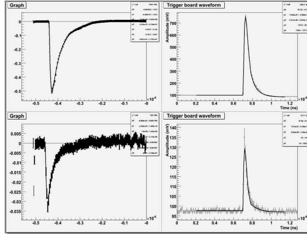
Figure 3. Alpha and \gamma waveform for DRS (negative) and trigger (positive) digitizer
