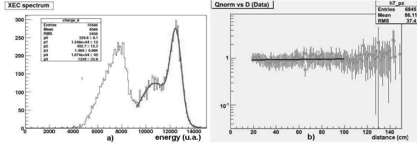
Figure 5. a) Lithium peak. b) A distribution of the ratio of simulated and real photoelectrons number versus the distance of each photomultiplier to evaluate Xe purity
