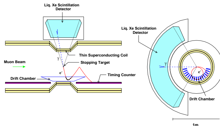
Figure 1. The set-up of the MEG experiment. The C-shaped liquid xenon calorimeter is visible on both views
