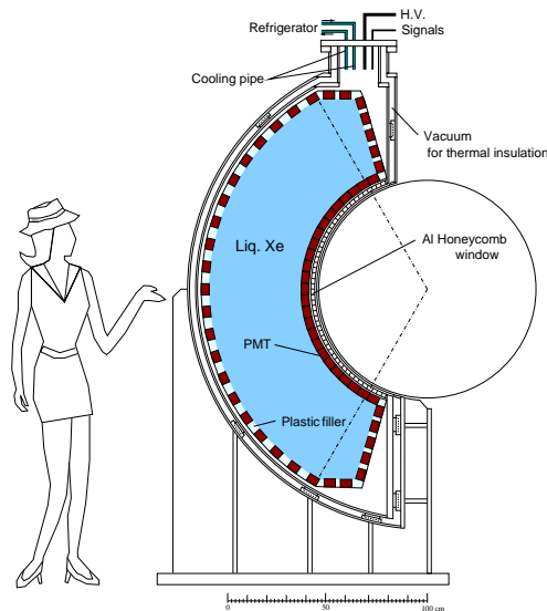
Figure 2. View of liquid xenon calorimeter
