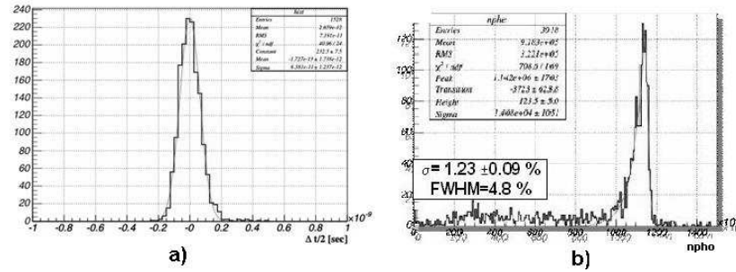
Figure 6. Time (a) and energy (b) resolution on 52.9 MeV photons
