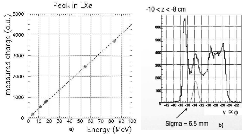
Figure 7. a) Checked charge at different photon energies in the calorimeter. b) Spatial resolution obtained by 52.9 MeV photons using a lead collimator
