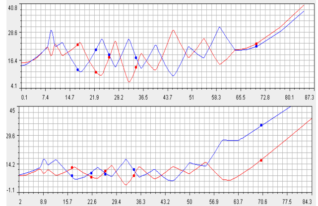
Figure 4: Beam envelope fitting when beam extracted at different time: upper: 5 ms, lower: 20 ms Solid dots: measurement result (red: horizontal, blue: vertical). Solid line: beam envelope fitted.
