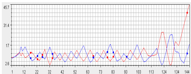
Figure 5: Beam envelope in RTBT. Solid dots measurement result (red: horizontal, blue: vertical). Solid line: beam envelope fitted.
