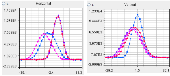
Figure 3: Measured results by wire scanners in RTBT. Left: horizontal profiles, Right: vertical profiles.
