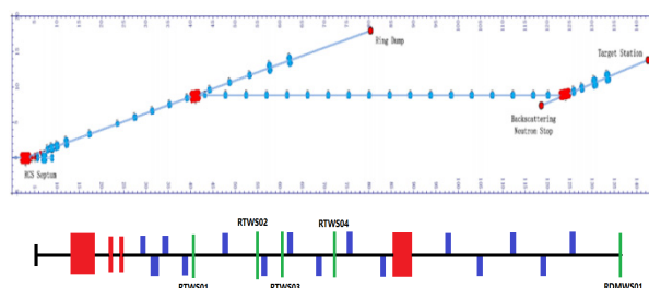
Figure 2: Layout of RTBT and RDBT beam transport line.
