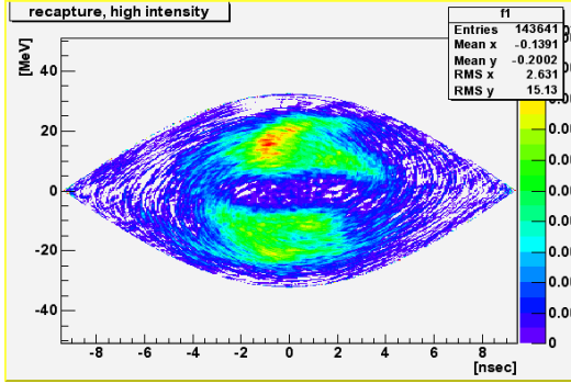
Figure 7: Longitudinal phase space tomography at recapture.
