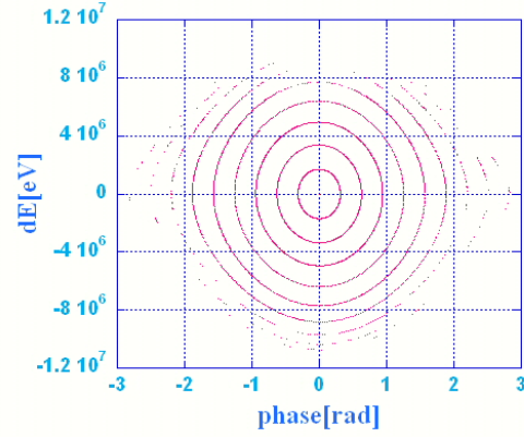
Figure 5: Injection distribution of the particles which could stay around synchronus phase after 12000 turns.
