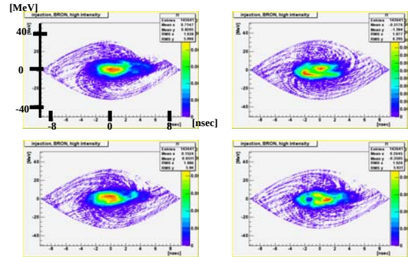
Figure 6: Longitudinal phase space tomography at injection.
