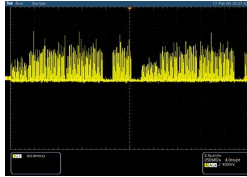
Figure 13: WCM signal at 120 GeV.
