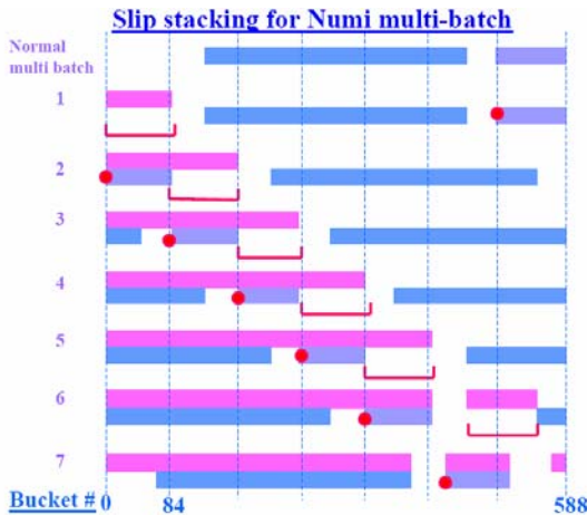
Figure 11: The scheme of 11 pulses slip stacking.
