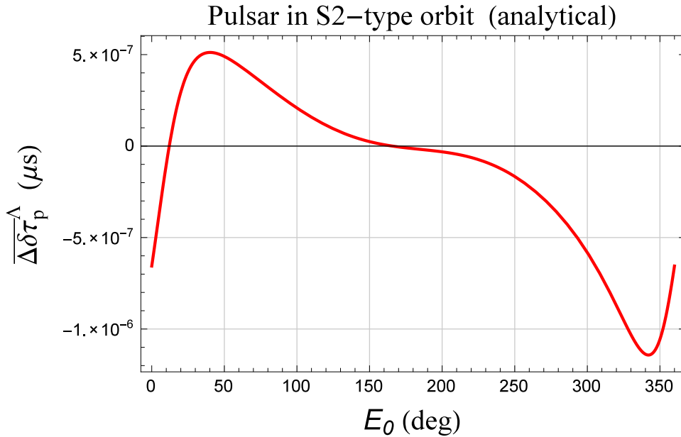
Figure A1. Average orbital time shift per orbit \overline{\Delta\delta\tau_p^\Lambda} , in \mu\text{s} , of a hypothetical pulsar in Sgr A* obtained analytically from Equation (27) along with the value of Equation (1) for \Lambda as a function of the initial phase E_0 . The orbital configuration of the S2 star, quoted in Table A1, was adopted. It can be noted that \overline{\Delta\delta\tau_p^\Lambda} vanishes for two given values of E_0 ; the largest absolute value occurs for E_0 = 342.08 deg. By assuming a pulsar timing accuracy of \sigma_{\tau_p} = 1 \mu\text{s} , it translates to an upper bound on \Lambda of the order of |\Lambda| \leq 9 \times 10^{-47} \text{ m}^{-2} ( \lesssim 10^{-116} in Planck units).
