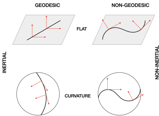
Fig. 5 This figure shows how tetrads behave in terms of inertial and gravitational effects. When no gravity is present, and we consider inertial effects only (i.e., we move along geodesics), we obtain trivial (holonomic) tetrads, whereas when non-inertial contributions take place (i.e., following non-geodesic orbits) the tetrads become anholonomic. The situation is analogue when gravitation is switched on. Along geodesic we obtain inertial frames, whereas along non-geodesic trajectories we have the most general anholonomic frames
