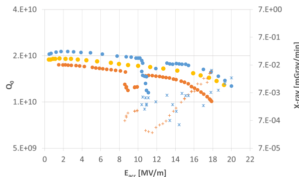
Figure 6: M006 tests: naked cavity (orange), after integration (blue) and after HPR retreatment (yellow)
