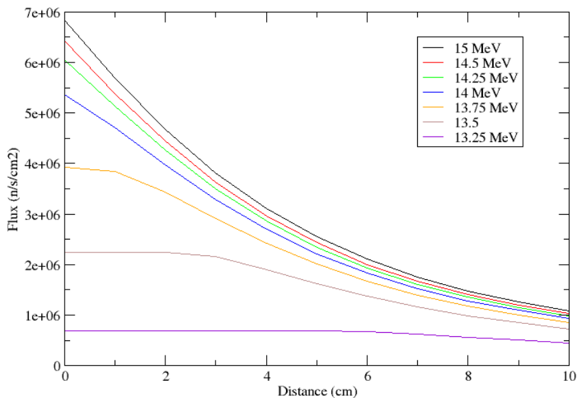
Fig. 4 Available neutron fluxes at zero degrees as a function of the distance of the gas cell
