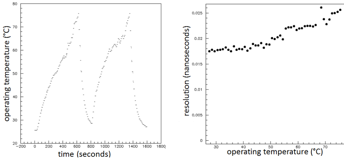
Figure 5.23: Thermal cycles. Left: Operating temperature as function of the elapsed time. Right: Carry chain delay line TDC resolution as a function of the operating temperature.
