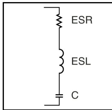
Figure 4.5: Parasitic model of a real capacitor.
