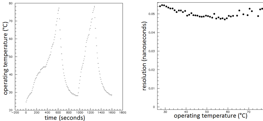
Figure 5.29: Thermal cycles. Left: Operating temperature as function of the elapsed time. Right: Vernier delay line TDC resolution as a function of the operating temperature.
