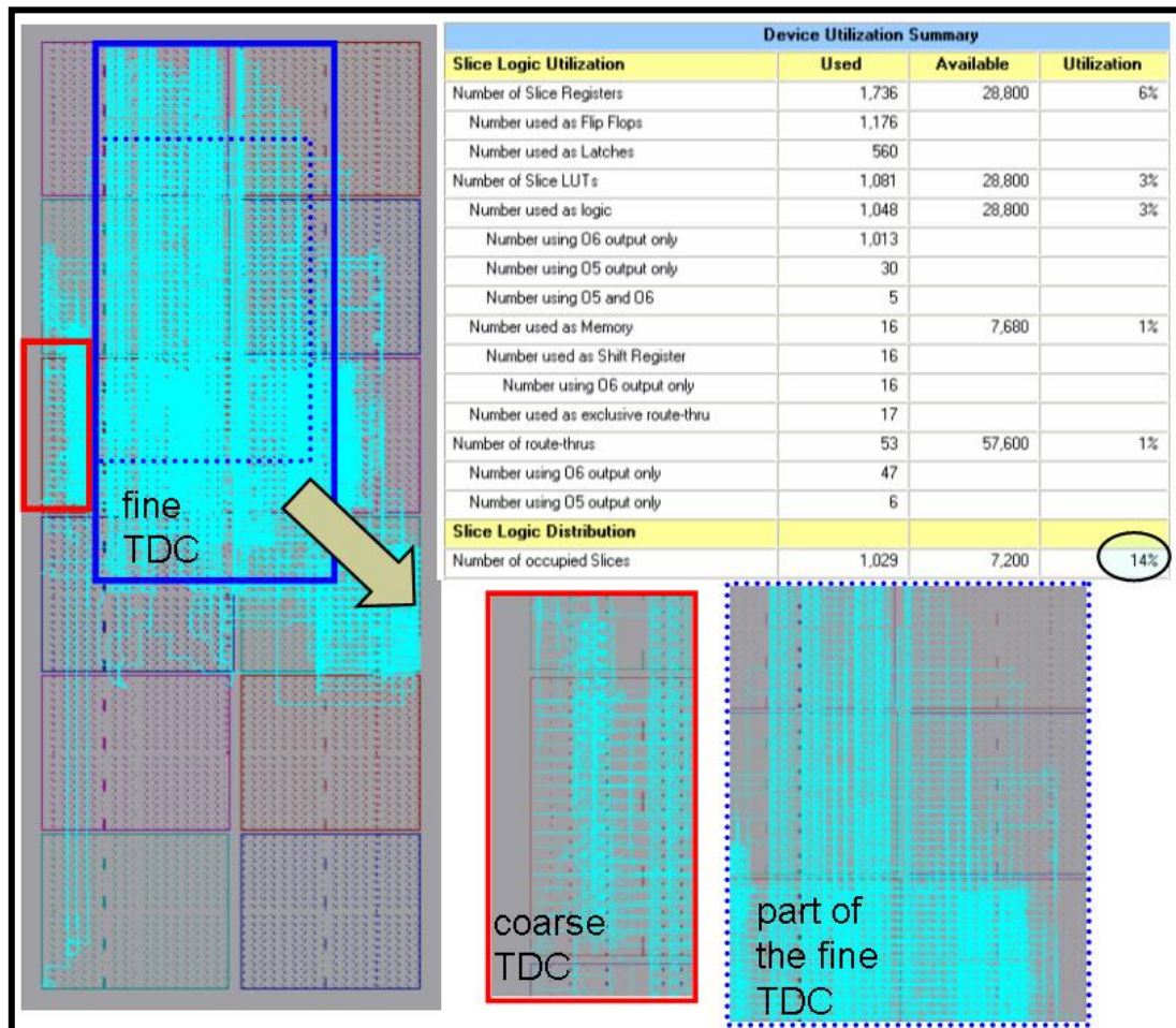
Figure 3.20: Vernier delay line TDC implementation.
