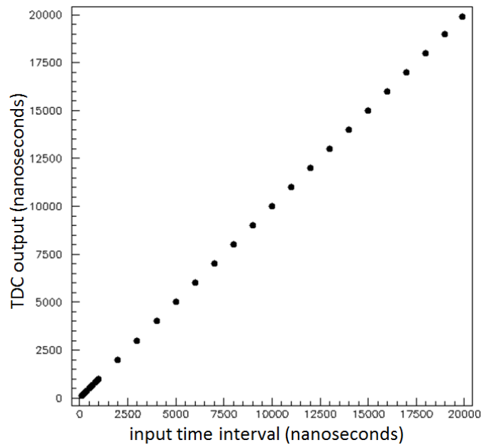
Figure 5.27: Vernier delay line TDC output as function of the input time interval.
