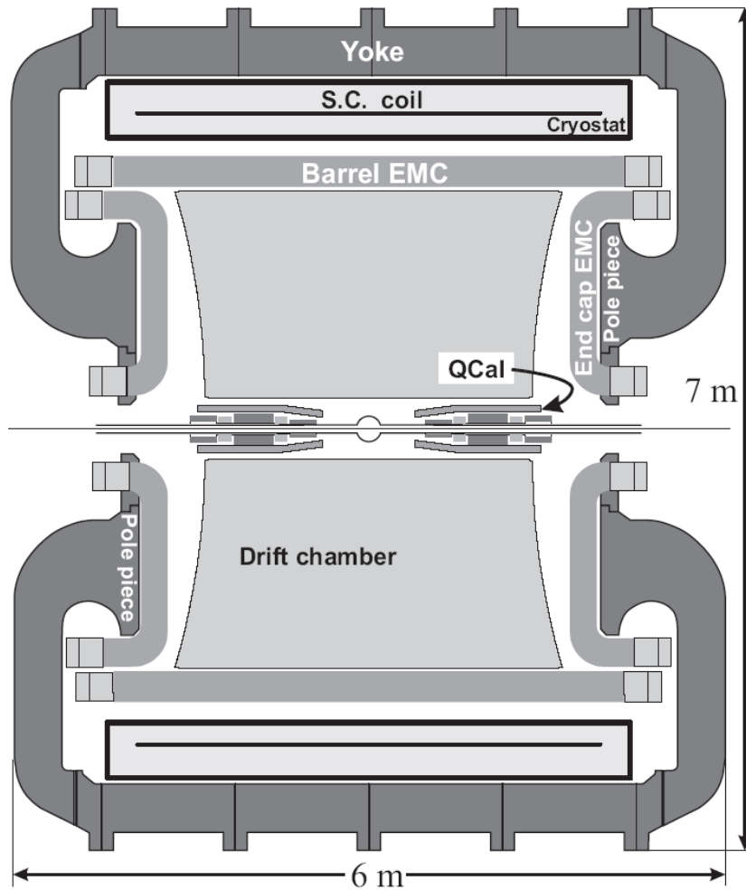
Figure 1.2: Cross-sectional view of the KLOE experiment, showing the interaction region, the DC, the EMC, the superconducting coil, and the return yoke of the magnet, the beam pipe with the spherical insertion, the low- \beta quadrupoles for the beam final focus and the two QCAL calorimeters around them.
