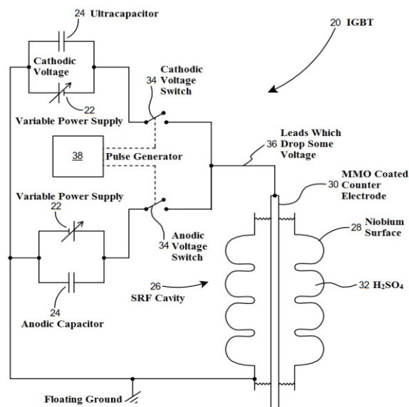
Figure 1: Schematic of the JLab BPEP equipment. [8]
