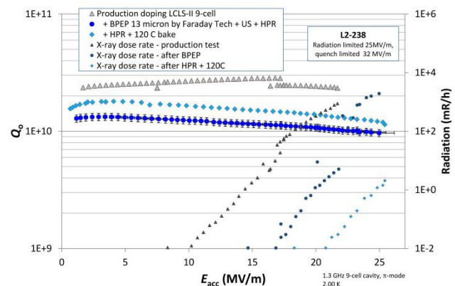
Figure 7: RF test of 9-cell cavity BPEP processed by Faraday.
