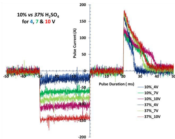
Figure 5: BPEP current with single cell cavity.
