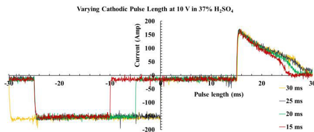
Figure 6: BPEP current with variation of cathodic pulse length.
