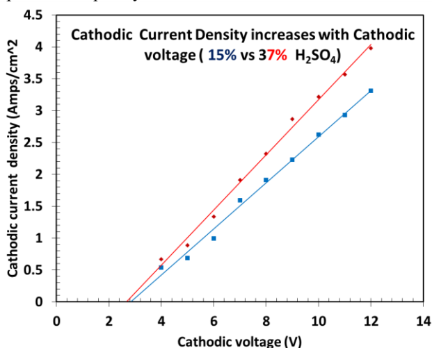
Figure 2: The cathodic current density increases with cathodic voltage for 15% and 37% H 2 SO 4 .
