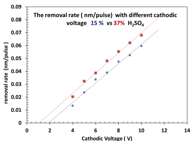
Figure 3: The average removal per pulse increases with cathodic voltage for 15% and 37% H 2 SO 4 .
