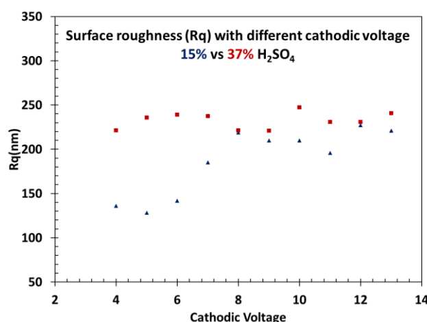
Figure 4: The surface roughness of samples processed by different cathodic voltage for 15% and 37% H 2 SO 4 .
