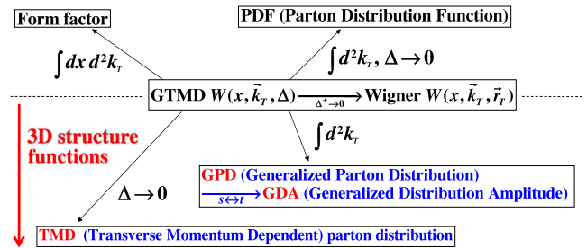
FIG. 1. Three-dimensional structure functions (TMD, GPD, GDA) from the generalized transverse-momentum-dependent parton distribution (GTMD) and the Wigner function, together with the form factor and parton distribution function.
