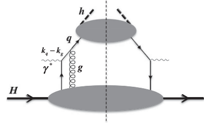
FIG. 3. A typical semi-inclusive DIS process \gamma^* + H \rightarrow h + X ( \ell \rightarrow \gamma^* \ell' , \ell' = e or \mu ) with a gluon interaction in the final state.
