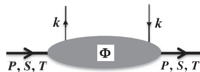
FIG. 2. Quark correlation function \Phi with the quark (hadron) momentum k ( P ) and the hadron vector and tensor polarizations S and T , respectively.
