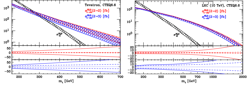
Figure 6.6: Cross sections (fb) at the Tevatron Run II (left) and LHC 10 GeV (right) for the sum of top and anti-top quark production in the t channel, as a function of the top mass obtained with the CTEQ6.6 PDF set and V_{tb} = 1 in the 2 \rightarrow 2 and 2 \rightarrow 3 schemes. Bands are the total uncertainty (scale+PDF). In the lower plots, dashed is scale uncertainty, solid is scale + PDF. Taken from Ref. [230].
