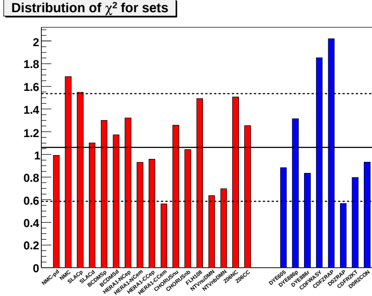
Figure 3.12: Values of the \chi^2 for the datasets included in the NNPDF2.0 reference fit [71], listed in Table 3.7. The horizontal line corresponds to the unweighted average of \chi^2 over datasets and the black dashed line to the 1\sigma interval about it: \langle\chi^2\rangle_{\text{sets}} = 1.06 , \sigma_{\chi^2} = 0.40 ; DIS and hadronic datasets are grouped respectively to the left and right of the histogram and distinguished by different colors.
