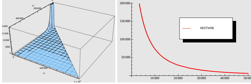
Figure 6.13: Partonic cross section multiplied by the parton luminosity plotted as a function of t_1 and s_1 (left) and parton luminosity as a function of s_1 (right) at the LHC S = (10\text{TeV})^2 . Input PDFs: MSTW08 [43].
