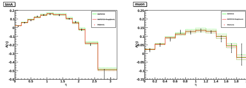
Figure 5.27: W electron asymmetry computed on the NNPDF2.0 set before and after the reweighting of the D0 W electron asymmetry (left) and D0 muon asymmetry (right).
