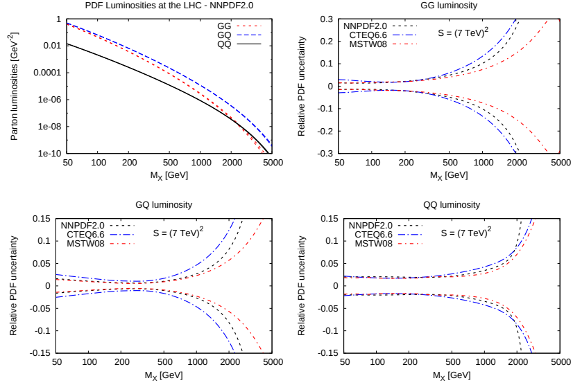
Figure 5.16: Parton-parton luminosities Eq. (5.29) in the various partonic channels, computed from the NNPDF2.0 set at the LHC for \sqrt{s} = 7 (top left). Relative PDF uncertainties on parton-parton luminosities Eq. (5.29) for the NNPDF2.0, CTEQ6.6 and MSTW2008 PDF sets, as function of the mass of the produced heavy object M_X at the LHC for 7 TeV. In a clockwise sense, the gluon-gluon luminosity, the gluon-quark luminosity and the quark-quark luminosity are shown.
