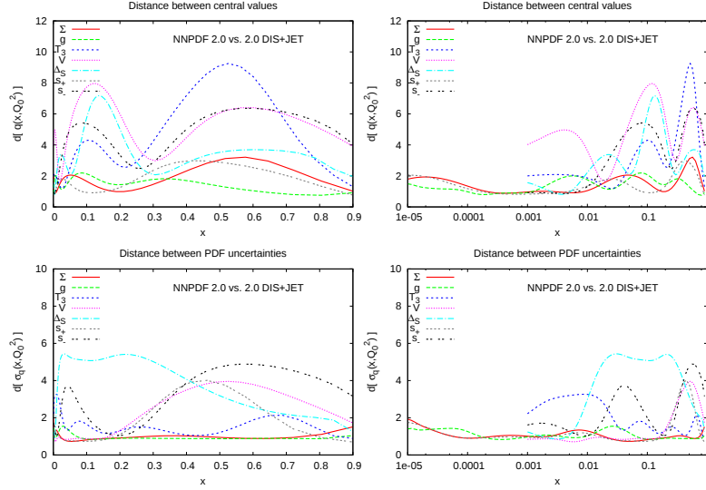
Figure 3.23: Distances between the PDFs obtained from the NNPDF2.0 DIS+JET fit of Fig. 3.21 and the reference NNPDF2.0 fit (Drell-Yan data also included). The distances are shown in linear (left) and logarithmic (right) scales for the central values (top) and the 1\sigma uncertainties.
