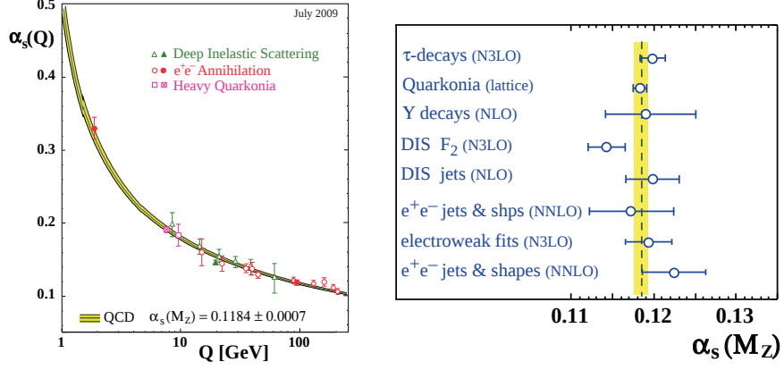
Figure 1: Experimental measurements of the universal QCD running coupling constant \alpha_s(Q) : (a) as a function of the scale Q ; (b) summary of the measurements converted to an equivalent \alpha_s(M_Z^2) . The vertical line and shaded band mark indicate the final world average value from these measurements [12].
