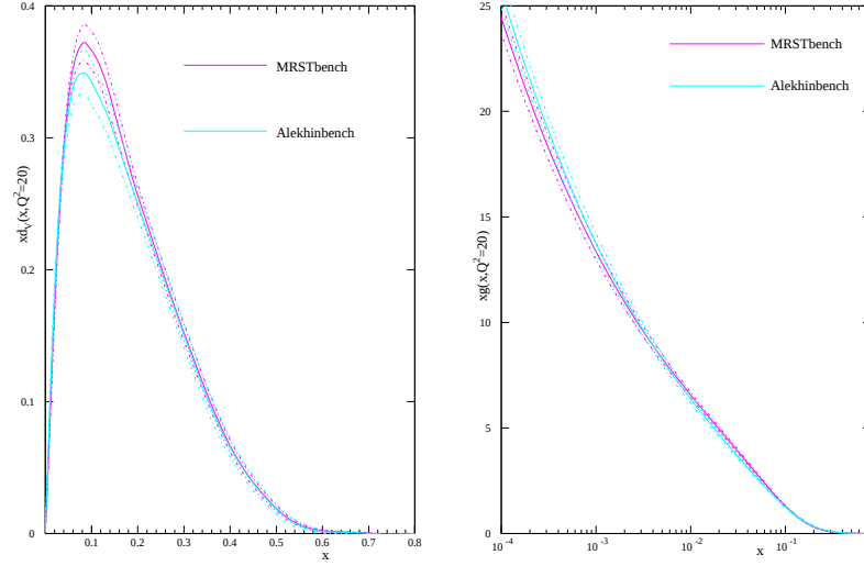
Figure 2.4: Left plot: x d_V(x) at Q^2 = 20 \text{ GeV}^2 from the MRST benchmark partons compared to the one from the Alekhin benchmark partons. Right plot: x g(x) at Q^2 = 20 \text{ GeV}^2 from the MRST benchmark partons compared to the one from the Alekhin benchmark partons. Taken from Ref. [101].
