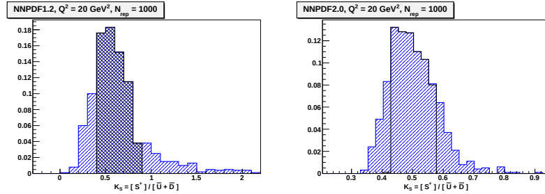
Figure 5.7: Distribution of K_S at Q^2 = 20 \text{ GeV}^2 computed from the reference set of N_{\text{rep}} = 1000 NNPDF1.2 (left) and NNPDF2.0 (right) PDF replicas. The central region corresponds to the 68% confidence interval.
