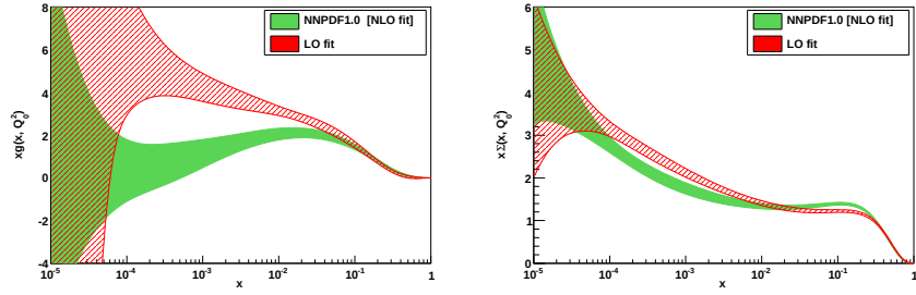
Figure 3.25: Comparison of the NLO NNPDF1.0 fit [68] and LO fit results for the gluon (left) and quark singlet PDFs (right).
