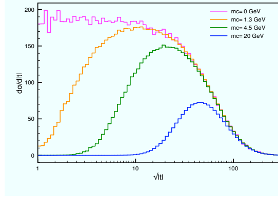
Figure 6.19: \log(t) distribution for \sqrt{S} = 1.96 TeV, M_W = 80.398 GeV and various values of m_c . The distribution is not normalised
