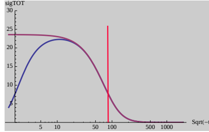
Figure 6.18: Plot of d\sigma/dt as a function of \sqrt{|t|}/m_c for l=2 , \sqrt{S} = 10 TeV, M_W = 80.398 GeV for m_c = 1.3 GeV (pink) and m_c = 0 (blue).
