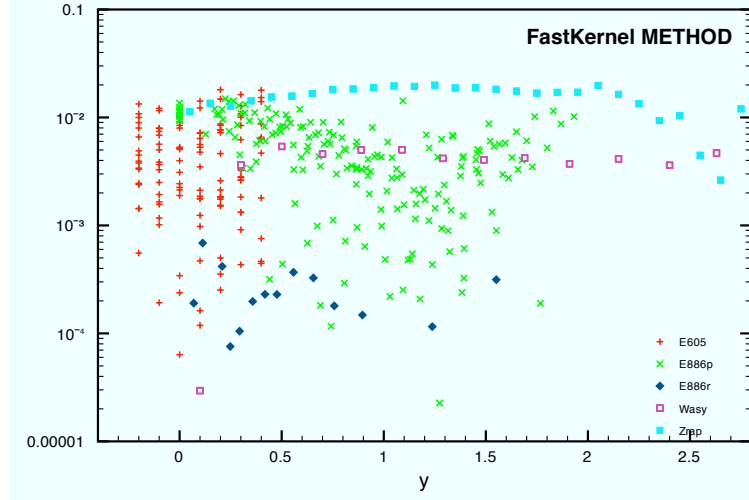
Figure 4.4: Relative accuracy for NLO Drell–Yan rapidity distributions using the FastKernel method, compared to the code of [166], as a function of rapidity y . Each point corresponds to the kinematics of a data point included in the NNPDF2.0 fit. The accuracy refers to a grid of 100 points distributed as the squared root of the logarithm from x_{\min} to 1.
