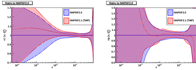
Figure 3.26: The ratio of the preliminary NNPDF2.1 Singlet (left plot) and gluon PDFs (right plot) to the respective NNPDF2.0 ones, at the initial evolution scale Q_0^2 = 2 \text{ GeV}^2 . Error bands are normalised to the NNPDF2.0 central value.
