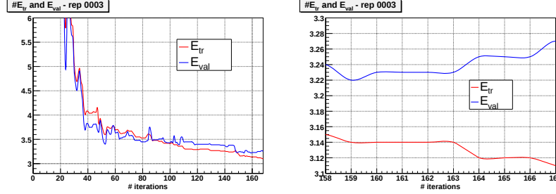
Figure 3.6: Training and validation error functions as a function of the number of iterations for one of the replicas in the reference fit. The stopping region is zoomed on the right-hand side plot.
