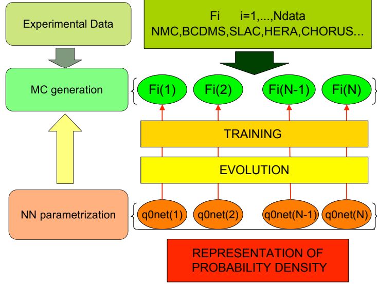
Figure 3.1: Schematic representation of the NNPDF approach.
