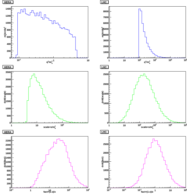
Figure 6.8: Q^2/m_b^2 (top), s/m_b^2 (middle) and (1-z)/z (bottom) logarithmic distributions for b\bar{b} production in the HERA (left – 2 < Q^2 < 100 , 0.1 < y < 0.9 , E_p = 920 \text{ GeV} , E_e = 27.5 \text{ GeV} ) and LHC-like (right – 2 \cdot 10^3 < Q^2 < 10^6 , 0.001 < y < 0.8 , E_p = 7 \text{ TeV} , E_e = 1.05 \text{ TeV} ) kinematics. Input PDF: CTEQ66 [42].
