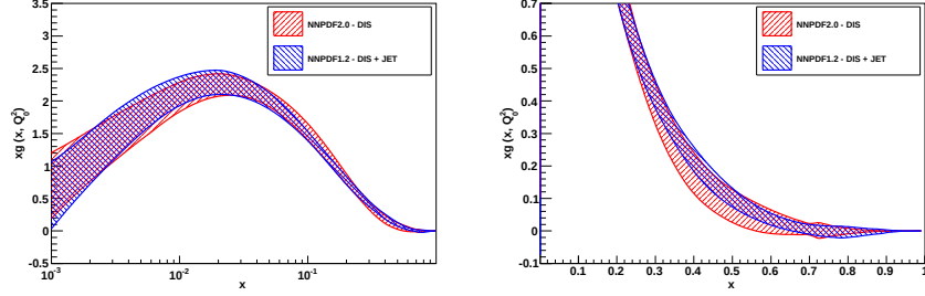
Figure 3.22: Comparison between the gluon density at the initial scale Q_0^2 = 2 \text{ GeV}^2 at small (left) and large (right) x obtained from NNPDF2.0 DIS fit of Fig. 3.20 and a fit in which jet data are also included (NNPDF2.0 DIS+JET) (the distances are shown in Fig. 3.21).
