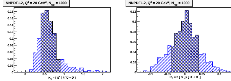
Figure 5.6: Probability distribution of K_S (left) and R_S (right) at Q^2 = 20 \text{ GeV}^2 computed from the reference set of N_{\text{rep}} = 1000 NNPDF1.2 PDF replicas. The region filled in black corresponds to the central 68% confidence interval, K_S(Q^2 = 20 \text{ GeV}^2) = 0.71^{+0.19}_{-0.31}{}^{\text{stat}} and R_S(Q^2 = 20 \text{ GeV}^2) = 0.006 \pm 0.045^{\text{stat}} .
