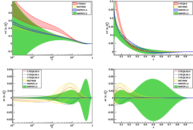
Figure 5.1: From top to bottom, the strange C-even and C-odd combinations s^+(x, Q_0^2) , s^-(x, Q_0^2) PDFs, plotted at the initial scale Q_0^2 = 2 \text{ GeV}^2 versus x on a log (left) or linear (right) scale, computed from the NNPDF1.2 set of N_{\text{rep}} = 1000 replicas. The NNPDF1.2 result is compared to the MSTW08 [43] and CTEQ6.6 [42] global fits. For s^- some of the results from obtained the CTEQ6.5s strangeness series [62] are also shown.
