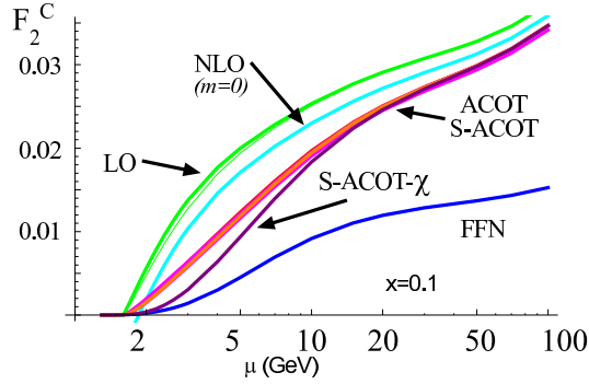
Figure 1.5: Calculation of DIS heavy quark production for a variety of schemes: LO represents QV \rightarrow Q process. NLO includes the \mathcal{O}(\alpha_s^1) processes in the massless approximation. In the FFNS the heavy quark PDF is set to zero and it only receives contributions from gV \rightarrow Q\bar{Q} . ACOT and S-ACOT are described in the text. Taken from Ref. [50].
