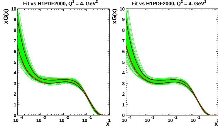
Figure 2.8: Comparison between errors on PDFs obtained via standard error calculation (black) where Gauss assumption is used, and errors obtained via Monte Carlo method (red) where luminosity uncertainty is allowed to fluctuate according to log-normal distributions and all the other uncertainties follow the Gaussian distribution (left), and where all the systematic uncertainties are allowed to fluctuate according to lognormal distributions (right). Only the gluon PDF is shown, where the errors are larger. The green lines show the spread of the N individual fits. Taken from Ref. [101]
