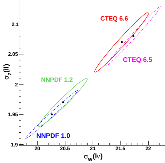
Figure 5.8: Comparison of the W and Z one sigma correlation ellipses at the LHC obtained from different fits: NNPDF 1.2 (green), NNPDF 1.0 (blue), CTEQ 6.6 (red) and CTEQ 6.5 (purple).
