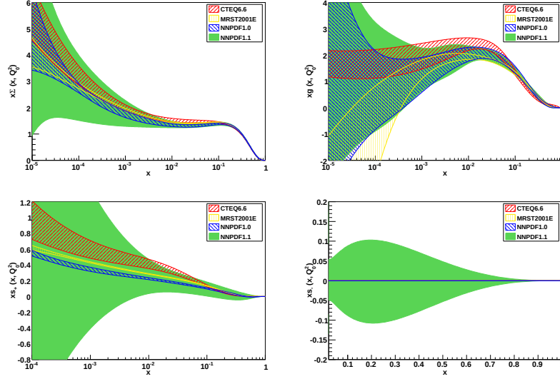
Figure 3.18: The NNPDF1.1 [69] singlet (top left), gluon (top right), total strangeness (bottom left) and strange valence (bottom right) compared to the NNPDF1.0, CTEQ66 and MRST01 sets.
