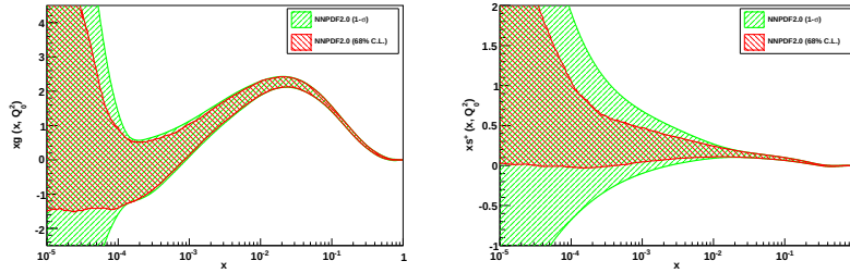
Figure 3.15: Comparison of 68% confidence level and 1\sigma intervals for the gluon (left) and the total strangeness (right). The PDFs have been determined in the NNPDF2.0 analysis [71] at the initial scale Q_0^2 = 2 \text{ GeV}^2 .
