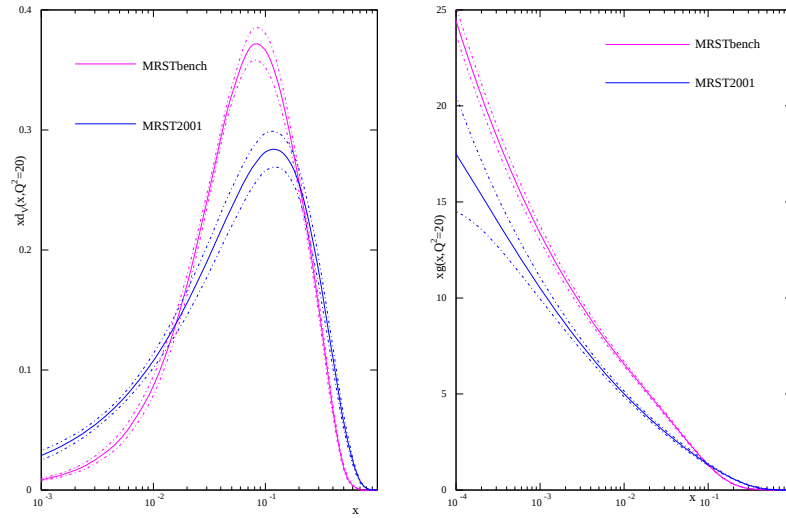
Figure 2.5: Left plot: x d_V(x) at Q^2 = 20 \text{ GeV}^2 from the MRST benchmark partons compared to that from the MRST01 partons. Right plot: x g(x) at Q^2 = 20 \text{ GeV}^2 from the MRST benchmark partons compared to that from the MRST01 partons. Taken from Ref. [101].
