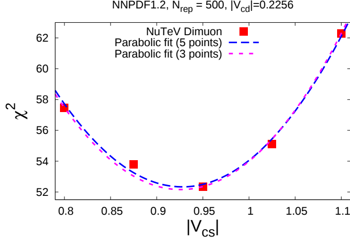
Figure 5.11: The \chi^2 of the NuTeV dimuon data as a function of |V_{cs}| when |V_{cd}| is kept fixed at its best unitarity fit value. The solid line is the parabolic fit from which the central value and 1\sigma uncertainty Eq. (5.21); the dashed curve is a parabolic fit to the central and two outer points only.
