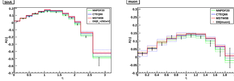
Figure 5.23: Prediction for the D0 W electron and muon asymmetries [146, 145] (left, electron binA: E_T > 25 GeV; ; right, muon E_T > 20 GeV) obtained with DNNLO at next-to-leading order, using the NNPDF20_1000 [71], CTEQ6.6 [41] and MSTW08 [43] parton sets. The uncertainty are the PDFs uncertainty, evaluated according to the HEPDATA recipe for MSTW08 and CTEQ6.6 and with the Monte Carlo prescription for the NNPDF2.0 set reported in Appendix C.
