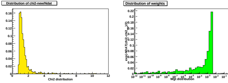
Figure 5.22: Distribution of the \chi_{\text{new}}^{2,(k)} and the weights in the reweighting of the jets inclusive cross-sections on the NNPDF20_DIS+DYP_1000 PDF set.
