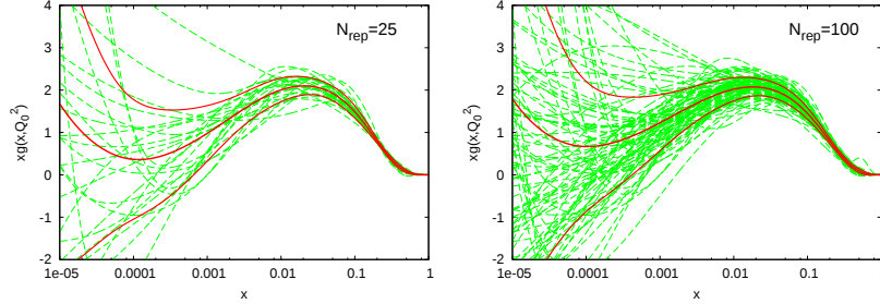
Figure 3.2: Sets of 25 replicas (left) and 100 replicas (right) of the gluon distribution at the initial scale Q_0^2 = 2 \text{ GeV}^2 from Ref. [68]. The solid red (dark) lines show the average and 1\sigma intervals computed from the given sets.
