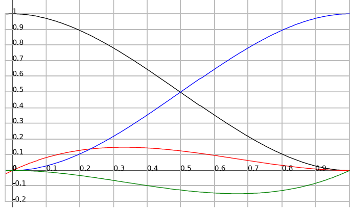
Figure 4.3: Set of interpolating Hermite cubic functions in the [0,1] interval.
