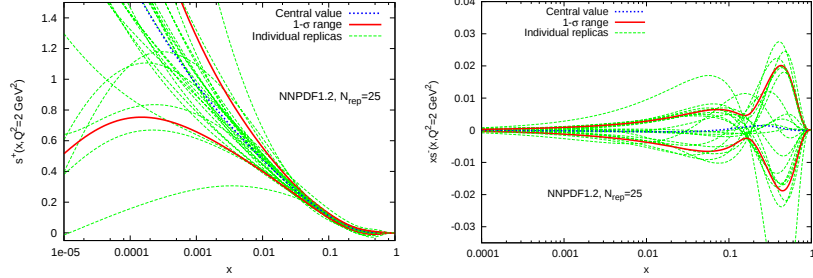
Figure 5.3: A set of randomly chosen N_{\text{rep}} = 25 replicas of the strange PDFs s^+(x, Q_0^2) (left), s^-(x, Q_0^2) (right) out of the full set of Fig. 5.1, and the PDFs computed from them.
