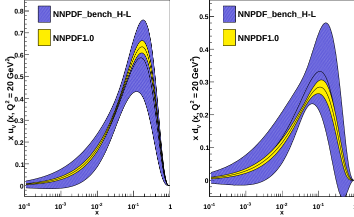
Figure 2.6: Comparison of the NNPDF benchmark and NNPDF1.0 reference fits for the u -valence (left) and d -valence (right) at Q^2 = 20 \text{ GeV}^2 .
