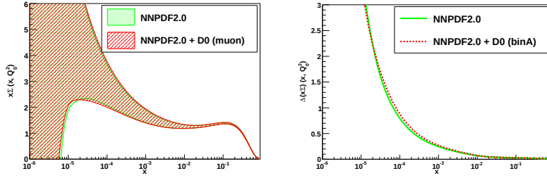
Figure 5.25: Singlet PDF and its absolute error at Q^2 = Q_0^2 for NNPDF2.0 and NNPDF2.0 + D0 muon data added by reweighting
