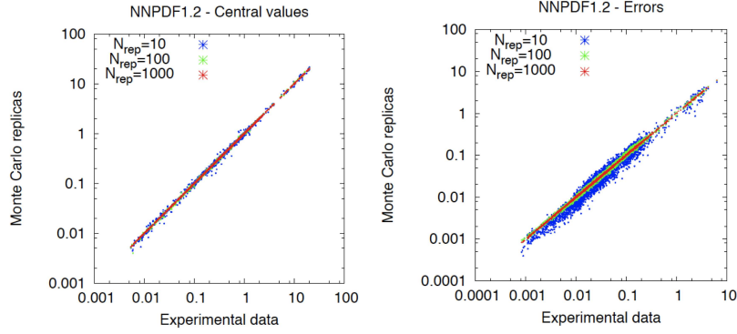
Figure 3.3: Scatter plot for mean values and errors evaluated and averaged over all the ensemble of MC replicas of the data according to the statistical estimators defined in Appendix B. Results are shown for a sample of 10, 100 and 1000 replicas in the NNPDF1.2 analysis.
