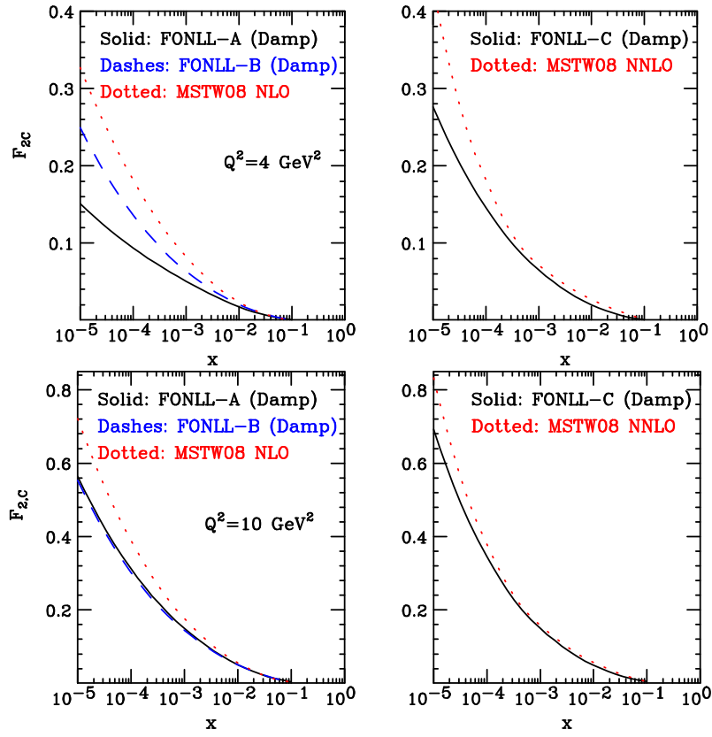
Figure 1.8: The F_{2c} structure function for Q^2 = 4 (top) and 10 (bottom) \text{GeV}^2 in FONLL and in TR', both for the NLO schemes (left plots) and for the NNLO schemes (right plots). In both cases the default threshold prescriptions are used: \chi -scaling for TR' and a damping factor for FONLL. Taken from Ref. [54].
