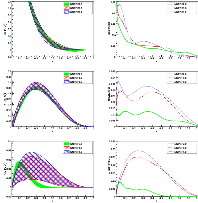
Figure 3.13: The gluon xg(x) (top), the triplet xT_3(x) (middle) and the sea asymmetry x\Delta_S(x) (bottom) at the initial scale Q_0^2 = 2 \text{ GeV}^2 from the NNPDF2.0 analysis. Both the PDFs (left) and their absolute uncertainties (right) are shown, compared to the previous NNPDF releases NNPDF1.0 [68] and NNPDF 1.2 [71].
