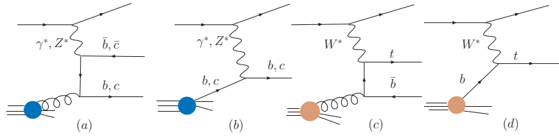
Figure 6.1: Leading-order diagrams for heavy quark production in the massive (a) and massless (b) scheme. Leading order diagrams for single top production in massive (c) and massless (d) schemes.
