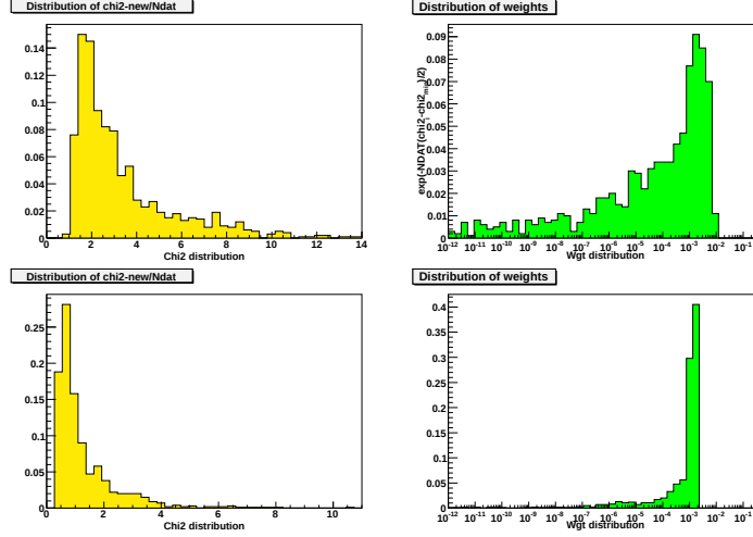
Figure 5.26: Distribution of the \chi_{\text{new}}^{2,(k)} and the weights in the reweighting of the D0 W electron asymmetry (top) and of the D0 muon (bottom) using the NNPDF20_1000 set as a initial probability distribution.
