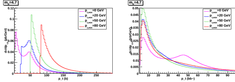
Figure 6.10: Comparison of normalised LO transverse momentum differential cross sections for bottom productions in the LHC kinematic. PDF input set: CTEQ66 [42]. Cut on the transverse momentum of the outgoing b quark.
