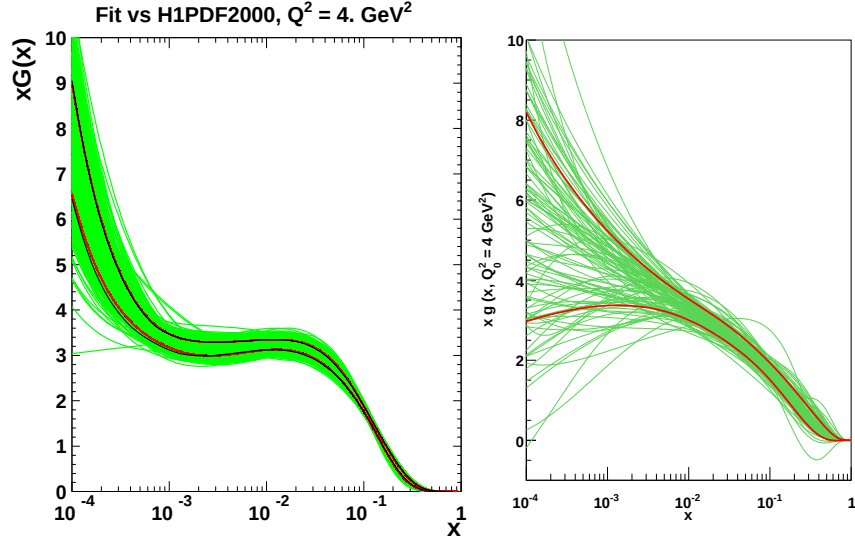
Figure 2.9: Left: The Monte Carlo set of gluon PDFs for the H1 benchmark. The comparison between the standard error calculations and the Gaussian error distribution for the gluon PDF shows a good agreement. Green lines represent the spread of Monte Carlo generated allowances for the errors, and the red lines are the RMS of this spread. The black lines correspond to the standard error calculations of the PDF errors. Right: The Monte Carlo set of gluon PDFs for the NNPDF benchmark. The red lines show the 1\sigma contour calculated from the Monte Carlo set. Taken from Ref. [122]
