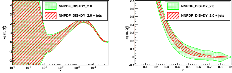
Figure 5.21: Small- x (left) and large- x gluon distribution at the initial scale Q_0^2 = 2 \text{ GeV}^2 . The gluon is evaluated before and after the inclusion of the jet data by reweighting.
