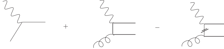
Figure 1.4: Schematic representation of the ACOT scheme implementation at NLO in the heavy quark production process.
