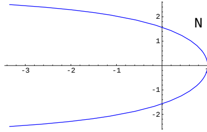
Figure 4.1: The path in the complex N -space followed by the Talbot integration path, Eq. (4.8) for r = 1 .
