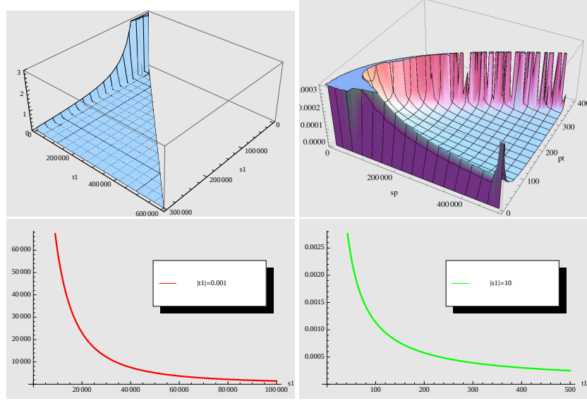
Figure 6.12: Partonic cross section plotted as a function of (|t_1|, s_1) (top left) and (p_T, s_1) (top right). Transverse sections of the top left 3D plot for a fixed value of t_1 (bottom left) and s_1 (bottom right).
