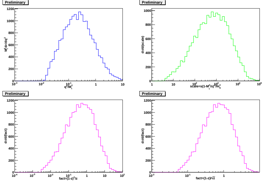
Figure 6.11: Distribution of q^2/M_t^2 (top left), the scale of the collinear logarithm (top right), the (1-z)^2/z factor (bottom left) and its squared root (bottom right). Here the energies of the proton beams are at 7 TeV. M_t = 174.3 GeV, m_b = 4.7 GeV. Input PDF: CTEQ6L1 [59].
