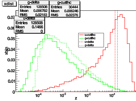
Figure 6.7: Solid lines: distribution of the fraction of momentum carried by the initial up quark and the gluon in the process ug \rightarrow ub\bar{b} , s = (14 \text{ TeV})^2 . Dashed lines: distribution of the fraction of momentum carried by the gluon in the process ug \rightarrow ub\bar{b} , if E_g = 7 \text{ TeV} and z_{up} = 0.15 , E_u = 1.05 \text{ TeV} .
