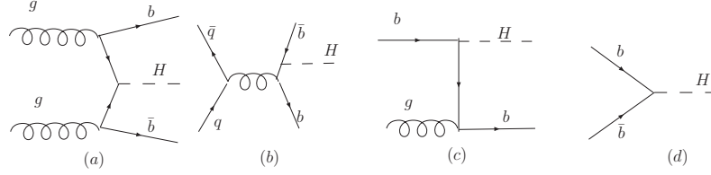
Figure 6.3: Leading-order diagrams for: (a),(b) inclusive Higgs production in the four-flavor scheme, (c) inclusive Higgs plus 1 b -jet production in the five-flavor scheme, (d) inclusive Higgs production in the five-flavor scheme.
