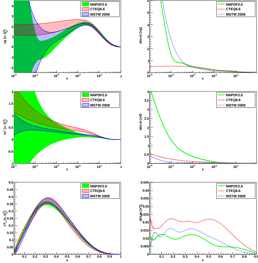
Figure 3.14: The gluon xg(x) (top), the total strangeness xS^+(x) (middle) and the triplet T_3(x) (bottom) at the initial scale Q_0^2 = 2 \text{ GeV}^2 from the NNPDF2.0 analysis. Both the PDFs (left) and their absolute uncertainties (right) are shown, compared to MSTW08 [43] and CTEQ6.6 [42] PDFs.
