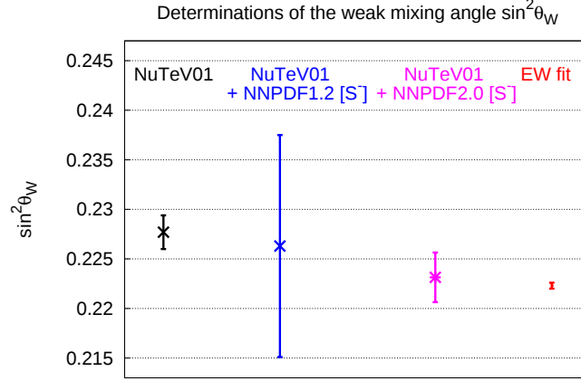
Figure 5.10: Determination of the Weinberg angle from the uncorrected NuTeV data [171], with [S^-] correction using NNPDF1.2 (Eq. (5.9)) and NNPDF2.0 (Eq. (5.9)) results, and from a global electroweak fit [182]. Note that only statistical uncertainties are included in the NNPDF2.0 correction.
