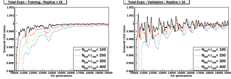
Figure 3.7: The training (left) and validation (right) ratios (defined in Eqs.(3.25, 3.26)) for a particular replica, as a function of the number of genetic algorithms generations, for various choices of the smearing parameter N_{\text{smear}} = \Delta_{\text{smear}} . The value N_{\text{smear}} = \Delta_{\text{smear}} = 200 is used in the reference fit (see Table 3.5).
