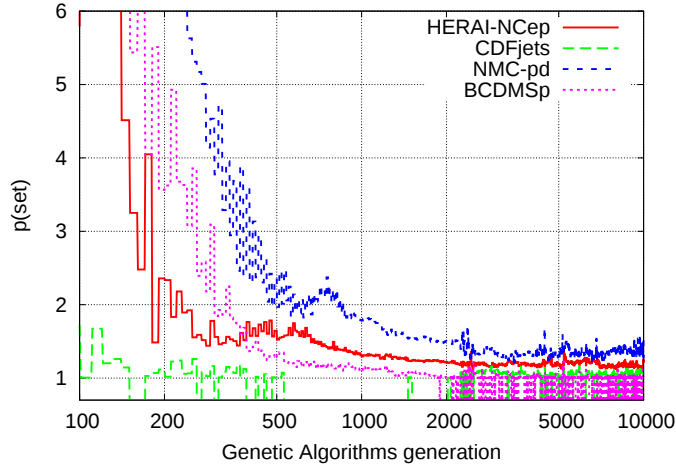
Figure 3.5: Illustration of the weighted training in one particular replica. Individual weights for each dataset converge to a value of p_i which is close to 1 as the training progresses. Only the behaviour of representative datasets is shown here.
