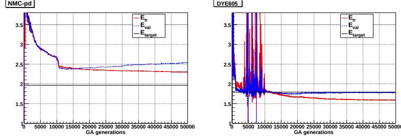
Figure 3.8: Two typical examples of overlearning behaviour, extracted from a fit with the same settings as the final reference fit of the NNPDF2.0 analysis [71] but with no stopping and a large maximum number of genetic algorithm generations N_{\text{gen}}^{\text{max}} = 50000 . The right plot shows the overlearning of the E605 experiment observed in one particular replica, and the left plot corresponds to the NMC-pd experiment. Note that in these fits weighted training is switched off at N_{\text{gen}}^{\text{wt}} = 10000 .
