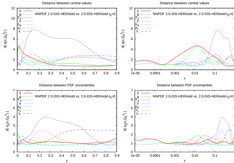
Figure 3.19: Distances between the PDFs obtained in a fit with improved genetic algorithm (IGA) and a fit with IGA + improved treatment of normalisation uncertainties (IGA+ t_0 ). The distances are shown in linear (left) and logarithmic (right) scales for the central values (top) and the 1\sigma uncertainties.
