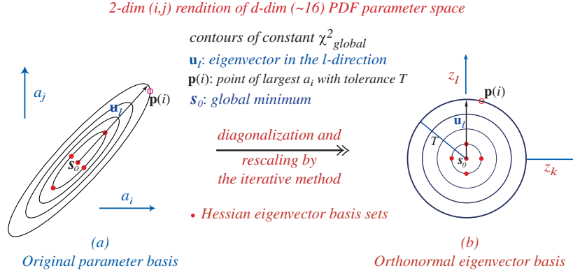
Figure 2.2: A schematic representation of the transformation from the PDFs parameter basis to the orthonormal eigenvector basis defined in Eq. (2.9). Taken from Ref. [113]
