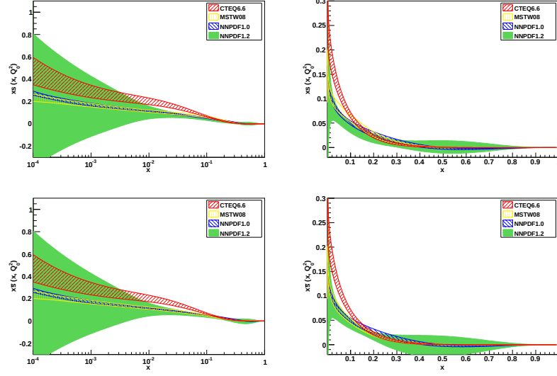
Figure 5.2: Same as Fig. 5.1 with strange s(x, Q_0^2) (top) and anti-strange \bar{s}(x, Q_0^2) (bottom) PDFs plotted at the initial scale Q_0^2 = 2 \text{ GeV}^2 .
