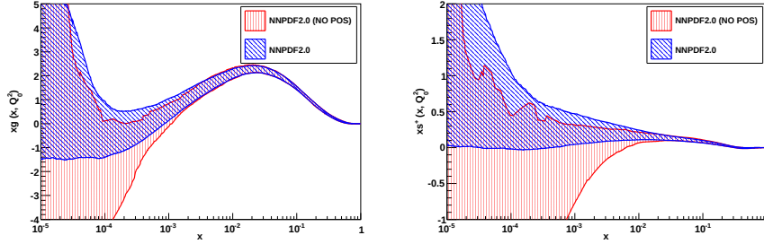
Figure 3.16: Gluon (left) and total strangeness (right) PDFs determined in the NNPDF2.0 analysis [71] at the initial scale Q_0^2 = 2 \text{ GeV}^2 with and without positivity constraints. All uncertainty bands are determined as 68% confidence levels. PDFs not shown here are not affected by the positivity constraints.
