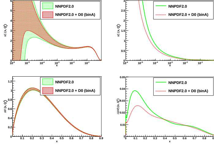
Figure 5.24: Singlet (top) and Valence (bottom) PDFs and their absolute errors at Q^2 = Q_0^2 for NNPDF2.0 and NNPDF2.0 + D0 electron data (bin A) added by reweighting.
