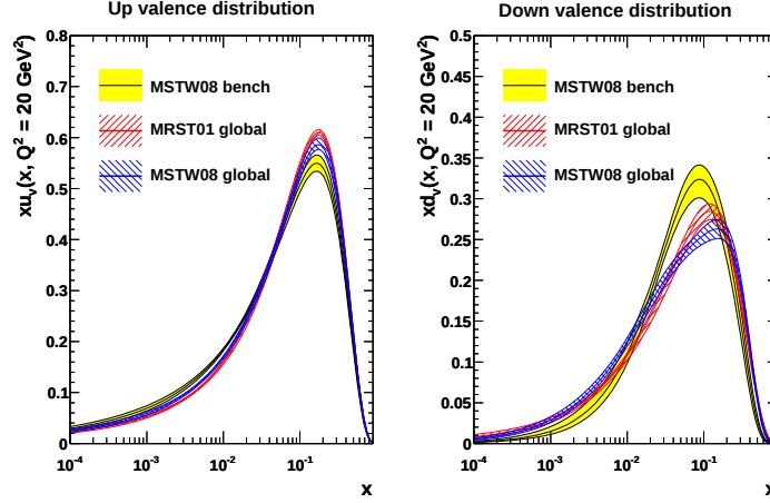
Figure 2.7: Comparison of the MSTW benchmark and MRST/MSTW global fits for the u -valence and d -valence at Q^2 = 20 \text{ GeV}^2 . All uncertainties shown correspond to 1\sigma bands.
