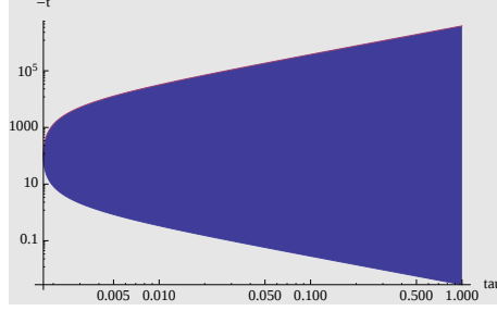
Figure 6.17: Region of integration of Eq. (6.43) in the plane (\tau, |t|) .
