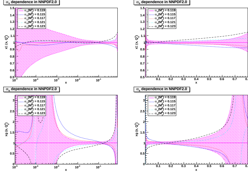
Figure 5.17: Ratios of PDFs with \alpha_s varied in the range 0.115 \leq \alpha_s \leq 0.123 to the central NNPDF2.0 determination, compared to the PDF uncertainty band: the singlet at small- and large- x , the gluon at small- and large- x (from top to bottom and from left to right).
