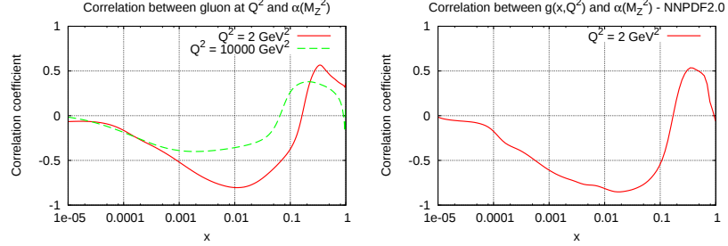
Figure 5.19: Correlation coefficient between the gluon PDF in the NNPDF1.2 (left) and NNPDF2.0 (right) analyses. The correlations is computed according to Eqs. (5.33, 5.34)
