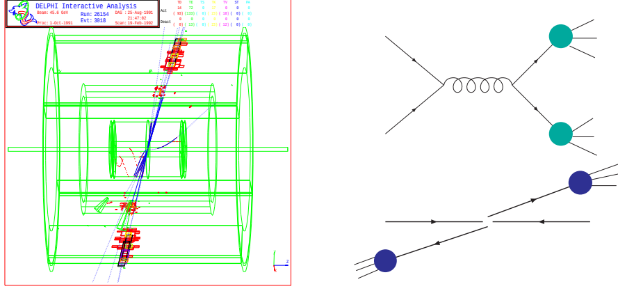
Figure 1.1: Typical event in e^+e^- \rightarrow \text{hadrons} with 2-jets in final state at LEP. Clear evidence for q\bar{q} creation.
