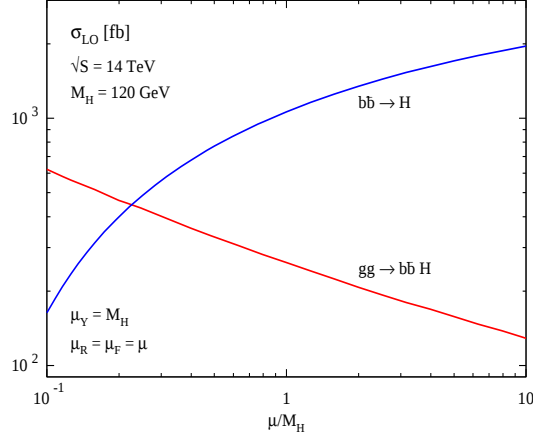
Figure 6.4: Scale variation of the LO inclusive Higgs production cross section prediction for pp \rightarrow b\bar{b}H + X at the LHC in the four- and five flavour schemes. Taken from Ref. [213].
