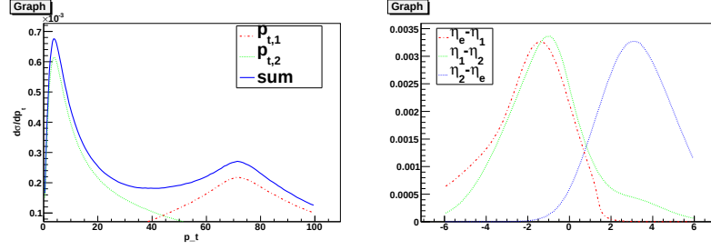
Figure 6.9: LO differential cross sections in p_T (left) and pseudo-rapidity \eta (right) for b\bar{b} production in LHC kinematics, Q_{min}^2 = 2000 GeV. The two dashed histograms represent the distributions relative to the most energetic quark ( b_1 ) and for the less energetic one ( b_2 ). PDF input set: CTEQ66 [42].
