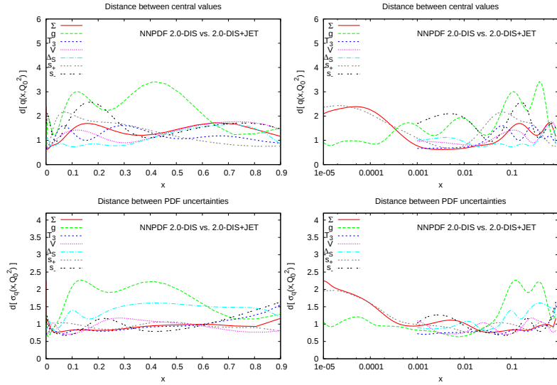
Figure 3.21: Distances between the PDFs obtained from a NNPDF2.0 DIS fit of Fig. 3.20 and those obtained from a fit in which jet data are also included (NNPDF2.0 DIS+JET). The distances are shown in linear (left) and logarithmic (right) scales for the central values (top) and the 1\sigma uncertainties.
