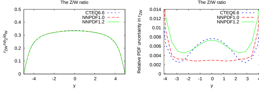
Figure 5.9: Left: the differential rapidity distribution of the ZW ratio, defined in Eq. 5.11. The very small PDF uncertainties are not shown. Right: the relative PDF uncertainties in r_{ZW} , as a function of the rapidity y .
