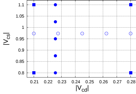
Figure 5.13: The grid of points used in the determination of the CKM matrix elements |V_{cs}| and |V_{cd}| . Open circles denotes points used for the determination of |V_{cd}| Eq. (5.22), and full circles points used for the determination of |V_{cs}| Eq. (5.21). All points are used in the joint determination Eq. (5.24).
