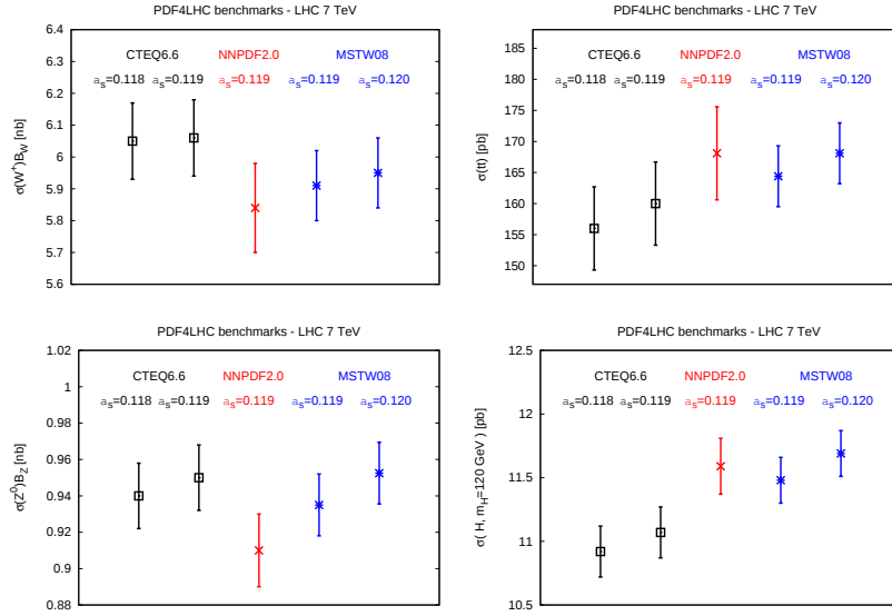
Figure 5.15: Comparison of predictions for LHC observables for NNPDF2.0, MSTW08 and CTEQ6.6 sets for the LHC at centre of mass energy of 7 TeV.
