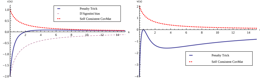
Figure 2.3: The “bias” functions c(x) for the central value (left plot) and v(x) for the variance (right plot), corresponding to the results obtained when the d’Agostini bias is present, using the penalty trick, and using the self-consistent covariance matrix method. The unbiased result corresponds to c = v = 0 .
