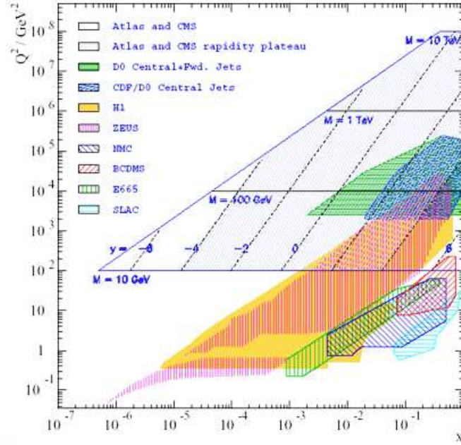
Figure 2: This plot shows the kinematical coverage of the LHC when the centre-of-mass energy will reach 14 TeV in the plane (x, Q^2) compared to the kinematical coverage of previous colliders.
