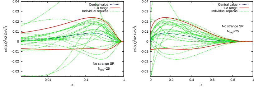
Figure 5.4: A set of randomly chosen N_{\text{rep}} = 25 replicas of the strange valence s^-(x, Q_0^2) out of the full set of Fig. 5.1, and the PDFs computed from them. Here sum rule Eq. (3.31) is not imposed during the fitting procedure. Both small- x (left) and large- x (right) regions are shown.
