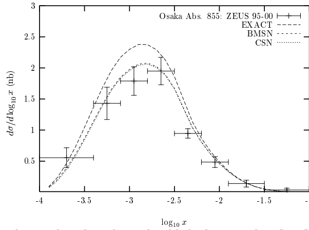
Figure 6.2: The combined Osaka and published ZEUS-data [210] for d\sigma/d\log_{10} x (nb) for DIS production of D^{*,\pm} -mesons. The dashed line is the NLO fixed flavor number scheme result F_{2,c}^{\text{EXACT}} , from the program HVQDIS [207]. The dotted line (BMSN-scheme [205]) and dashed-dotted line (CSN-scheme [211]) are based on a variable flavor number scheme computation F_{2,c}^{\text{VFNS}} . Taken from Ref. [209].
