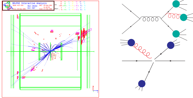
Figure 1.2: Typical event in e^+e^- \rightarrow \text{hadrons} with 3-jets in final state at LEP. Clear evidence for q\bar{q}g creation.
