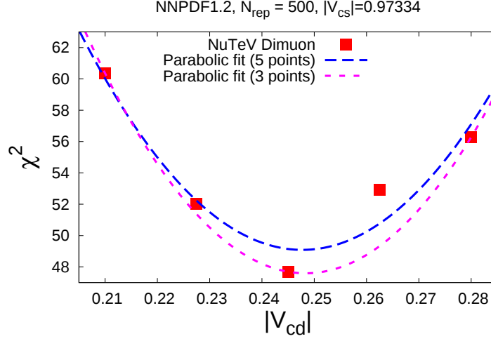
Figure 5.12: The \chi^2 of the NuTeV dimuon data as a function of |V_{cd}| when |V_{cs}| is kept fixed at its best unitarity fit value. The solid line is the parabolic fit from which the central value and 1\sigma uncertainty Eq. (5.22); the dashed curve is a parabolic fit to the central and two outer points only.
