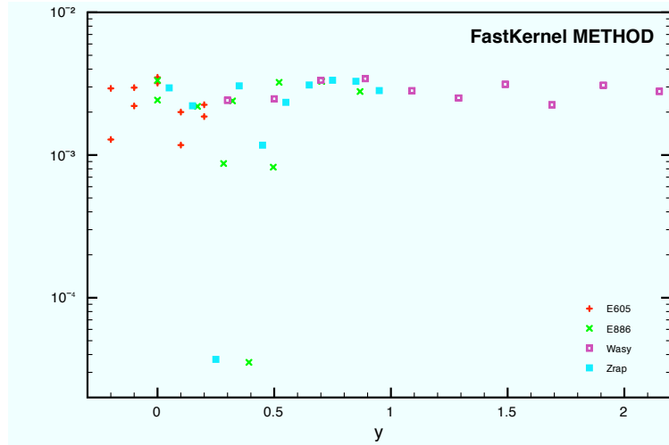
Figure 4.5: Same as Fig. 4.4, for 40 points in the kinematical range covered by the data points included in the NNPDF2.0 fit, using a grid of 500 points distributed as the squared root of the logarithm from x_{\min} to 1.
