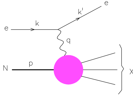
Figure 1.3: Schematic representation of deep–inelastic charged lepton–nucleon scattering.
