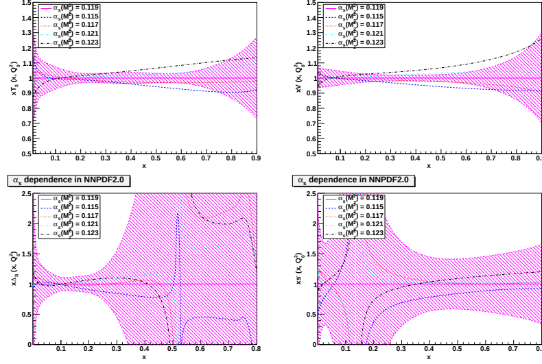
Figure 5.18: Ratios of PDFs with \alpha_s varied in the range 0.115 \leq \alpha_s \leq 0.123 to the central NNPDF2.0 determination, compared to the PDF uncertainty band: triplet, valence, sea asymmetry and strange valence (from top to bottom and from left to right).
