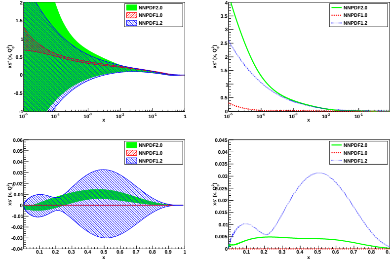
Figure 5.5: xs^+(x, Q_0^2) (top), xs^-(x, Q_0^2) (bottom) PDFs combinations (left) and their absolute uncertainties (right), plotted at the input scale Q_0^2 = 2 \text{ GeV}^2 versus x , computed from the NNPDF1.2 set of N_{\text{rep}} = 1000 replicas. The NNPDF2.0 [71], NNPDF1.2 [70] and NNPDF1.0 [68] distributions and their absolute errors are compared.
