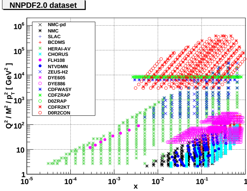
Figure 3.10: Experimental data which enter the NNPDF2.0 analysis. For hadronic data, the values of x_1 and x_2 determined by leading order partonic kinematics (Eqs. (3.40), (3.41) and (3.48)) are plotted.
