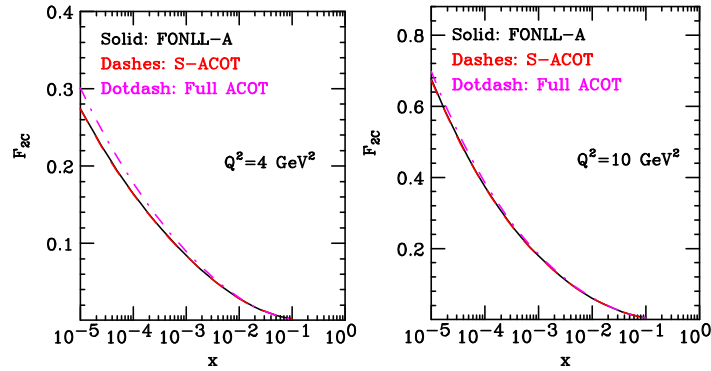
Figure 1.7: The F_{2c} structure function for Q^2 = 4 (left) and 10 (right) \text{GeV}^2 in the FONLL scheme A (plain) compared to the Simplified ACOT (S-ACOT) and full ACOT schemes. Taken from Ref. [54].
