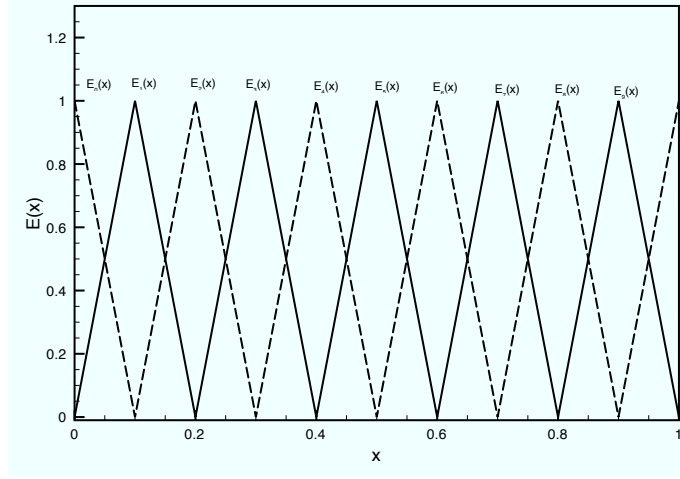
Figure 4.2: Set of interpolating triangular basis functions. The corresponding analytical form is given in Eq. (4.45).
