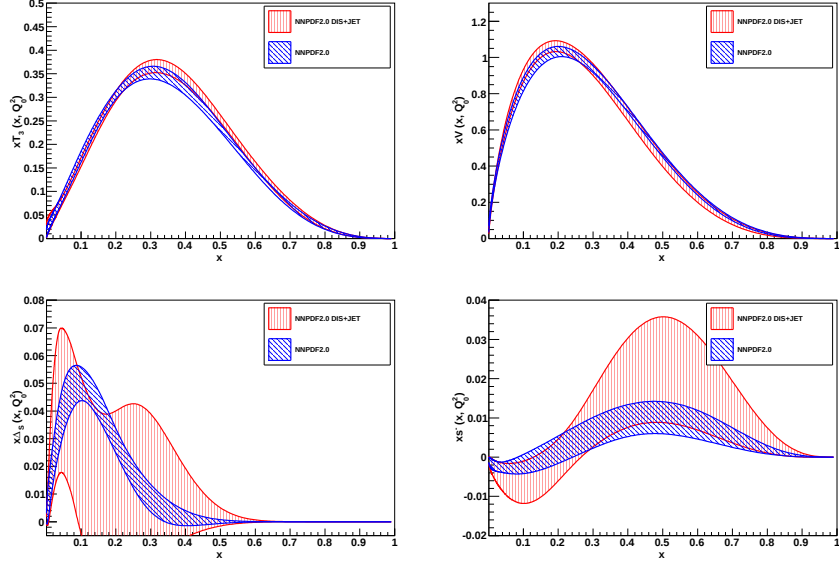
Figure 3.24: Comparison between PDFs at the initial scale Q_0^2 = 2 \text{ GeV}^2 from the NNPDF2.0 DIS+JET fit of Fig. 3.21 and the reference NNPDF2.0 fit which included also Drell–Yan data (the distances are shown in Fig. 3.23). From left to right and from top to bottom the following distributions are shown: triplet, valence, sea asymmetry and strange valence.
