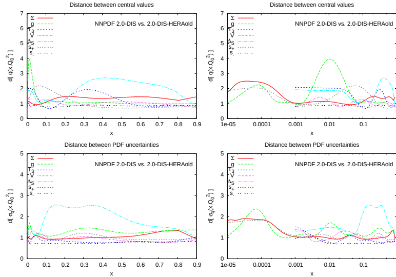
Figure 3.20: Distances between the PDFs obtained with a IGA+ t_0 fit of Fig. 3.19 and a fit in which the separate H1 and ZEUS data are replaced by the combined HERA-I DIS data (NNPDF2.0 DIS). The distances are shown in linear (left) and logarithmic (right) scales for the central values (top) and the 1\sigma uncertainties.
