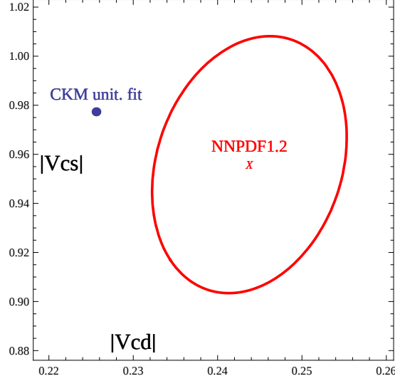
Figure 5.14: Location of the best-fit point and 1\sigma (statistical \Delta\chi^2 = 1 uncertainty) ellipse in the (|V_{cd}|, |V_{cs}|) plane for the best-fit \chi^2 paraboloid obtained from the \chi^2 computed at the points displayed in Fig. 5.13. The best unitarity fit result [189] is also shown for comparison.
