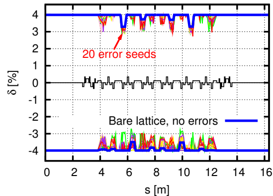
Figure 3: Overall MA (shown for one achromat) from 6D tracking including alignment, field, and multipole errors (20 seeds), and assuming RF acceptance set at 4%.
