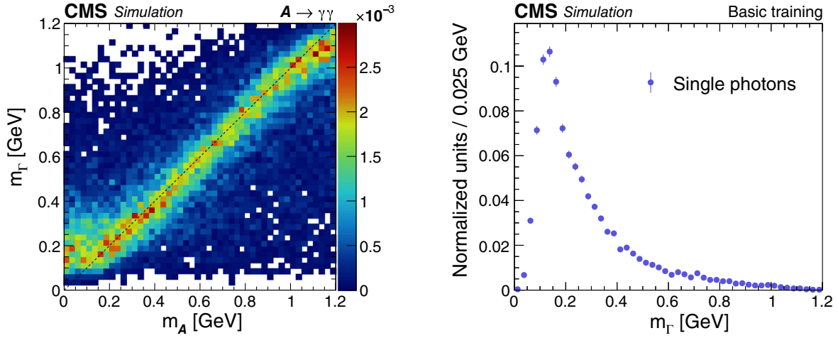
FIG. 2. Left: the regressed mass m_T vs the generated m_A value for simulated \mathcal{A} \rightarrow \gamma\gamma decays generated uniformly in (p_T, m_A) before domain continuation is implemented. The regressed m_T is normalized in 0.025 GeV vertical slices of the generated m_A . The color scale to the right of the plot gives the normalized number of events per vertical slice in 0.025 GeV bins of m_T . Right: the regressed m_T distribution for simulated single-photon samples only, before domain continuation, resulting in a distinct peak in the low- m_T region. The distribution is normalized to unity with the vertical bars on the points indicating the statistical uncertainty.
