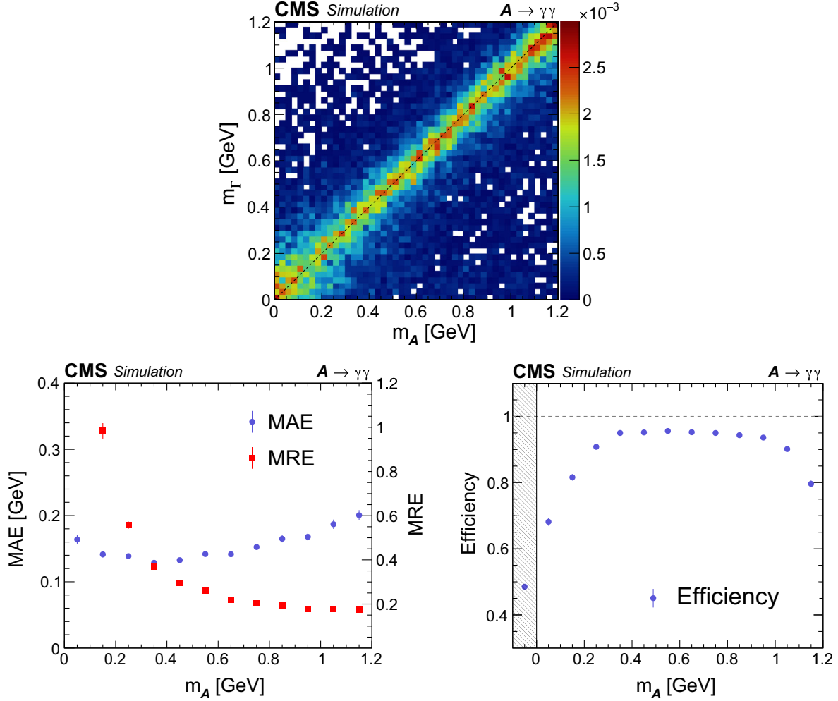
FIG. 4. Mass regression performance for simulated \mathcal{A} \rightarrow \gamma\gamma samples generated uniformly in (p_T, m_{\mathcal{A}}) , corresponding to mean boosts in the range \langle \gamma_L \rangle = 600\text{--}50 for m_{\mathcal{A}} = 0.1\text{--}1.2 GeV. Upper: regressed m_T vs generated m_{\mathcal{A}} . The regressed m_T is normalized in 0.025 GeV vertical slices of the generated m_{\mathcal{A}} . The color scale to the right of the plot gives the normalized number of events per vertical slice in 0.025 GeV bins of m_T . Lower left: the MAE (blue circles, use left scale) and MRE (red squares, use right scale) vs the generated m_{\mathcal{A}} . For clarity, the MRE for m_{\mathcal{A}} < 0.1 GeV is not shown since its value diverges as m_{\mathcal{A}} \rightarrow 0 . Lower right: the m_{\mathcal{A}} regression efficiency as a function of the generated m_{\mathcal{A}} . The hatched region shows the efficiency for single photons. The vertical bars on the points show the statistical uncertainty in the simulated sample.
