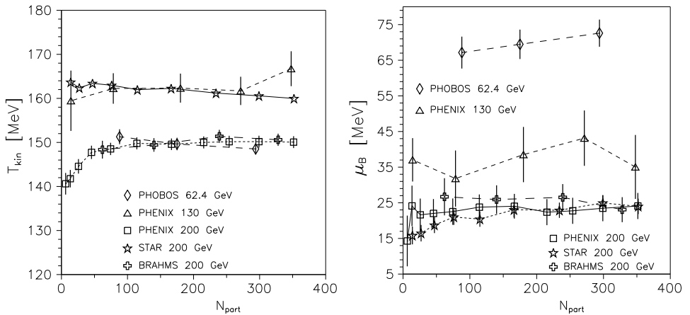
Fig. 4. Centrality dependence of the kinetic freeze-out temperature (left) and of the baryon number chemical potential (right), for the RHIC measurements at \sqrt{s_{\text{NN}}} = 62.4, 130 and 200 GeV. The lines connect the results and are a guide.
