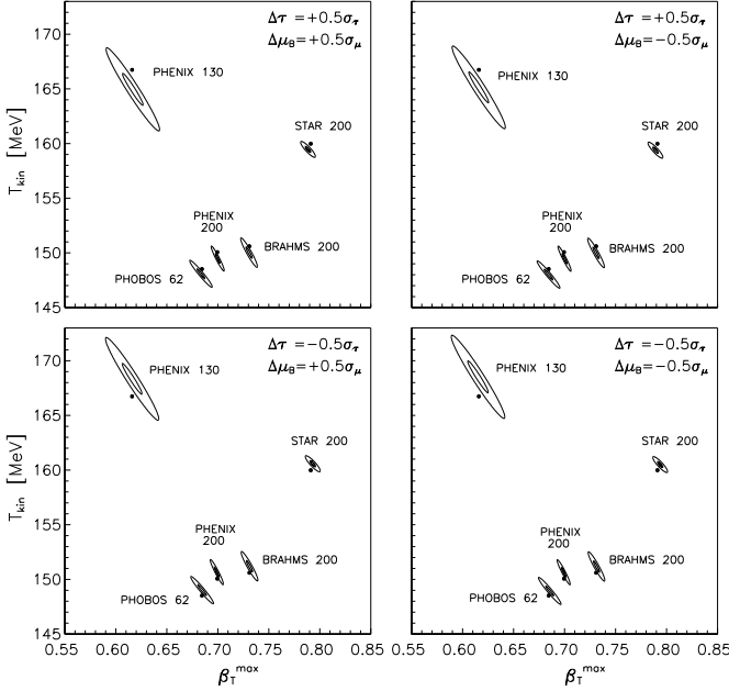
Fig. 3. The \chi^2 contours ( 1\sigma and 2\sigma ) in the parameter planes T_{\text{kin}} and \beta_{\perp}^{\text{max}} fixed by taking \mu_{\text{B}} and \tau at \pm 0.5\sigma from their optimum values, \Delta\tau = \tau - \tau_{\text{opt}} , \Delta\mu_{\text{B}} = \mu_{\text{B}} - \mu_{\text{B,opt}} . All cases represent the most central classes. Dots denote the projections of the points of optimum values of all parameters onto the appropriate plane T_{\text{kin}} - \beta_{\perp}^{\text{max}} .
