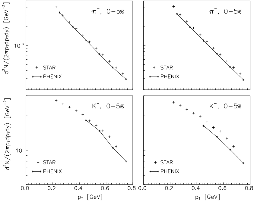
Fig. 11. Comparison of \pi^+ , \pi^- , K^+ and K^- spectra measured by STAR and PHENIX for the 0–5 % centrality bin at \sqrt{s_{\text{NN}}} = 200 GeV. All STAR data points are depicted, whereas PHENIX data ranges are cut from the right-hand side (in fact they extend to p_T = 2.95 GeV for pions and p_T = 1.95 GeV for kaons).
