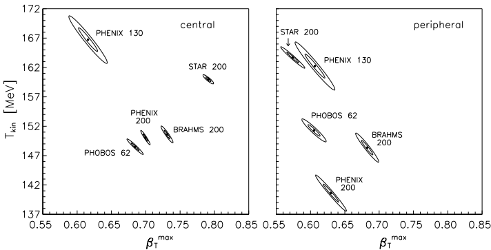
Fig. 2. The \chi^2 contours ( 1\sigma and 2\sigma ) in the parameter plane T_{\text{kin}} and \beta_{\perp}^{\text{max}} fixed by taking \mu_{\text{B}} and \tau at their optimum values. In the right panel the PHENIX case at \sqrt{s_{\text{NN}}} = 130 GeV is represented by the second from the most peripheral bin, see text for explanations. Dots denote the optimum values of T_{\text{kin}} and \beta_{\perp}^{\text{max}} .
