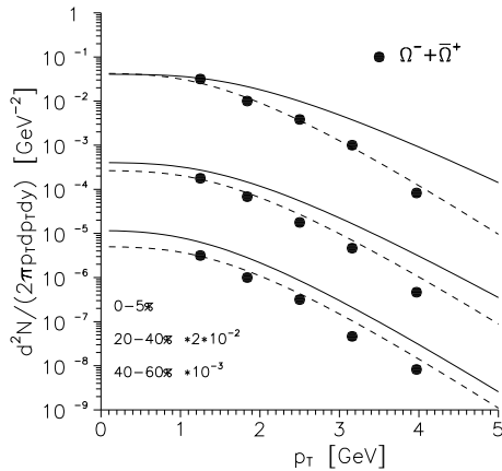
Fig. 10. Transverse momentum distributions of \Omega^- + \bar{\Omega}^+ for |y| < 0.75 in Au–Au collisions at \sqrt{s_{\text{NN}}} = 200 GeV. Data are from [31] (STAR) scaled for clarity, (statistical) errors are of the size of symbols. Lines denote model predictions: solid based on fits to the STAR spectra, dashed based on fits to the PHENIX spectra.
