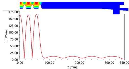
Figure 3: Magnitude of the longitudinal field on axis and gun geometry simulated by ANSYS-HFSS.
