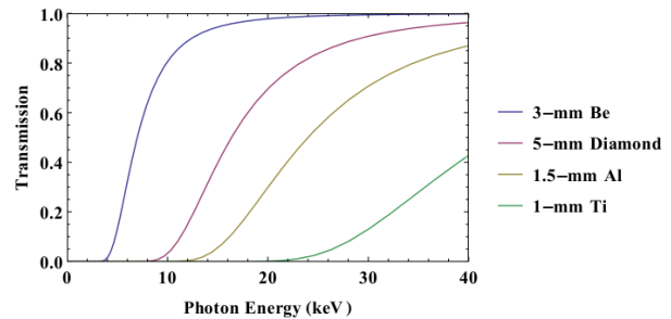
Figure 3: Transmission through different material considered for the radiation-extraction window as a function of photon energy.
