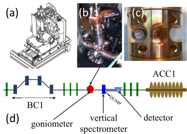
Figure 2: Sketch (a) and photograph (b) of the goniometer assembly on loan from HZDR. Diagram (d) shows the proposed location of the CR experiment in ASTA. Photograph (c) shows the water-cooled crystal holder.
