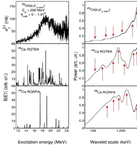
Fig. 4. Power spectra showing energy scales in experimental and theoretical spectra for the ^{48}\text{Ca} IVGDR.
