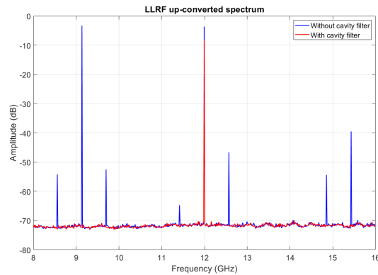
Figure 6: Up-converted measured vector modulator spectrum without (blue) and with (red) the cavity filter.
