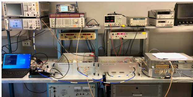
Figure 7: LLRF system under test at LNF RF laboratory.
