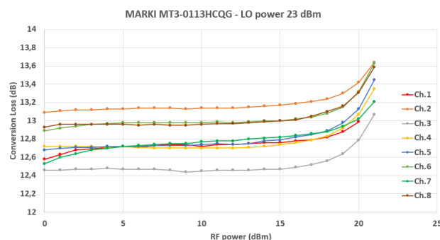
Figure 4: Calibration of Marki Microwave front-end mixers. The quoted conversion loss also accounts for the insertion loss of the 2.856 GHz band-pass filter and cable attenuation.
