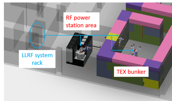
Figure 1: Drawing of the TEX facility area.
