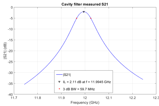
Figure 5: Measured S_{21} (absolute value) for the 11.994 GHz cavity filter.
