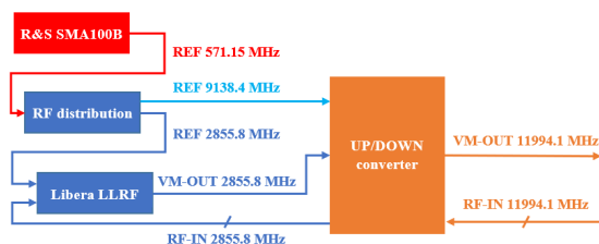
Figure 3: Block diagram of TEX LLRF system.
