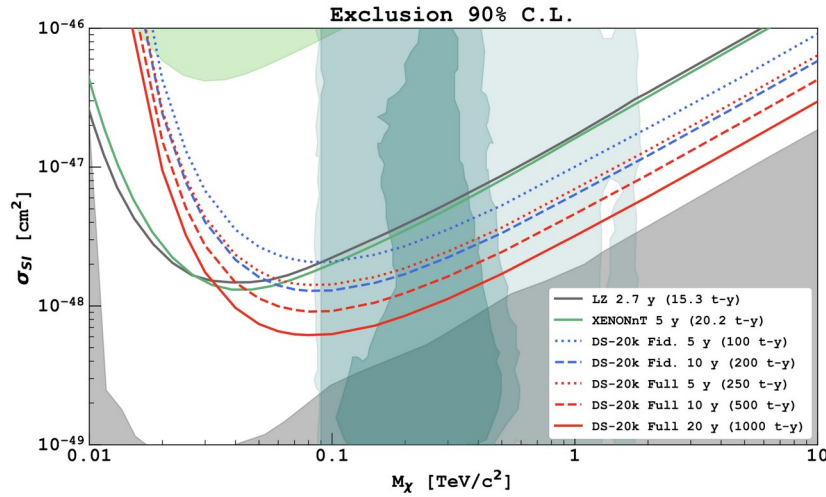
Fig. 6: The DarkSide-20k sensitivity projections to spin-independent WIMPs for different exposures compared to the nominal sensitivity current xenon based experiments that are expected to lead the field for WIMP searches in the next years [7, 8].
