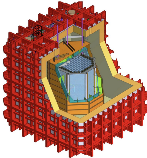
Fig. 3: From the outside: DarkSide-20k detector is contained in a ProtoDUNE-like cryostat (red) and inside is outer veto with atmospheric argon. The copper vessel (orange) separates it from the inner neutron veto. The TPC is supported by purple structure, hanging from the top of the cryostat. Gadolinium-loaded acrylic shell (green) separates the neutron veto from the TPC (transparent blue).
