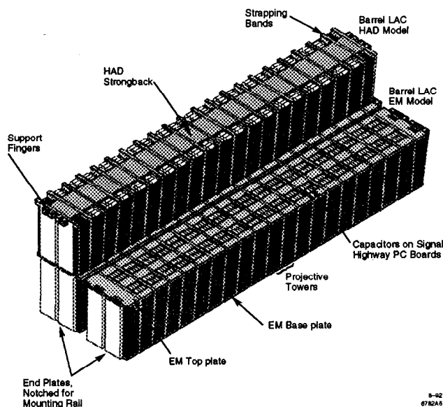
Figure 3.21: A LAC barrel module.
