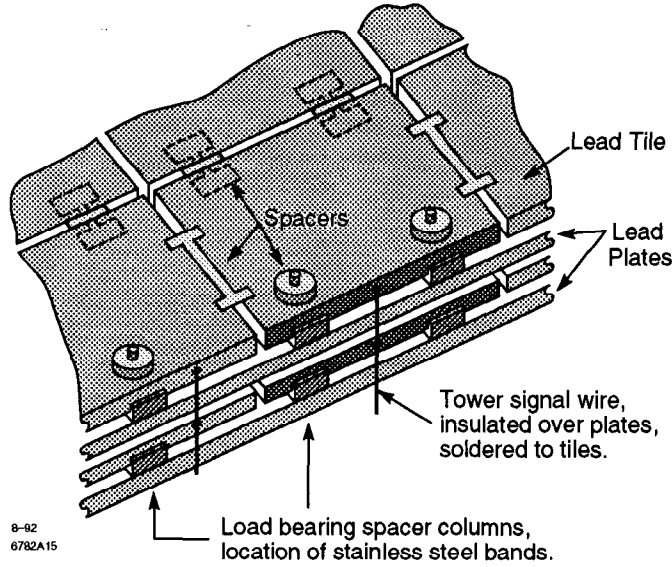
Figure 3.23: A LAC cell.
