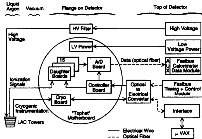
Figure 3.24: LAC electronics showing one tower, one “Tophat” and scheme for getting the signal to the FASTBUS.
