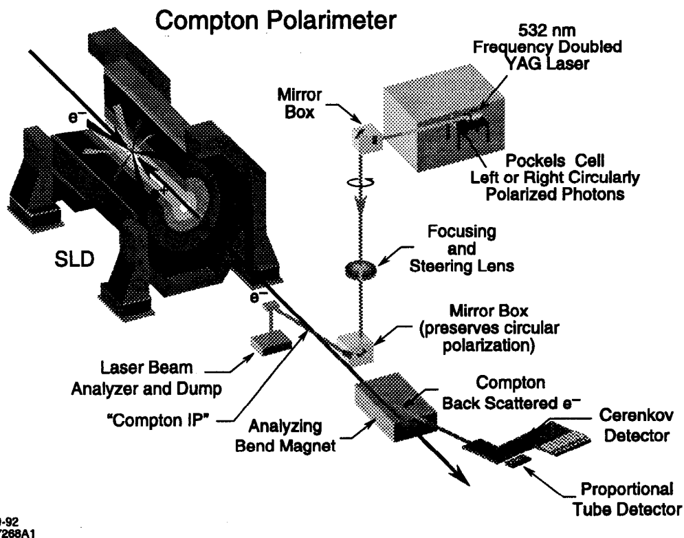
Figure 3.8: The Compton Polarimeter.
