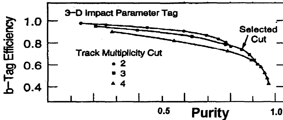
Figure 4.5: The generically-used 3-d impact parameter significance cut for tagging B hadrons [83]. The arrow shows typical required values of the minimum number of tracks and the minimum displacement from the IP of those tracks (in units of the error on that displacement, \frac{\sigma}{\delta\sigma} > d ).
