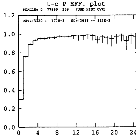
Figure 4.12: MC: Efficiency plot for association of a track to a cluster, binned in track |\vec{p}| (GeV/c), showing the problem of tracks not getting matched to clusters at low |\vec{p}| .
