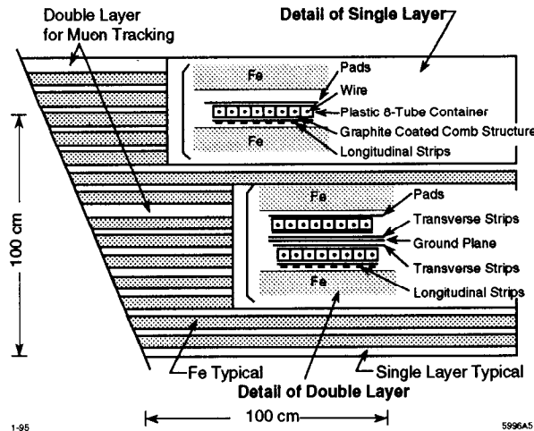
Figure 3.17: An r\phi(xz) view of the barrel(endcap) WIC. Inlaid are the two types of WIC layers.
