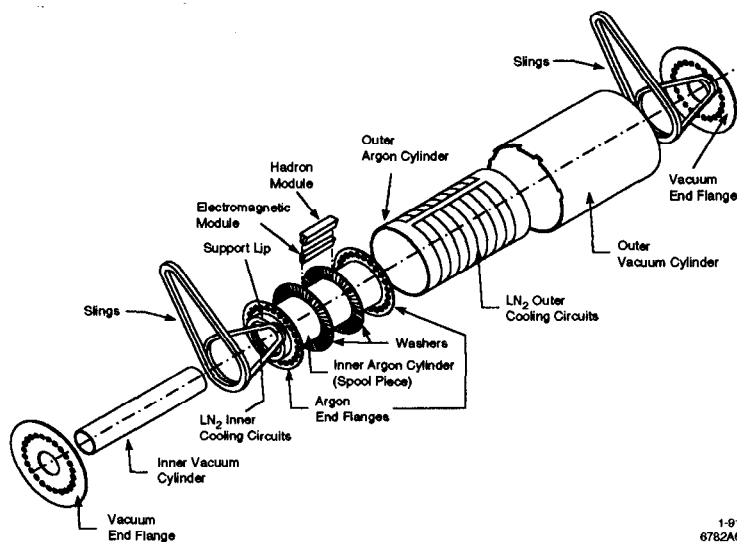
Figure 3.19: LAC barrel, showing the placement of one barrel module.
