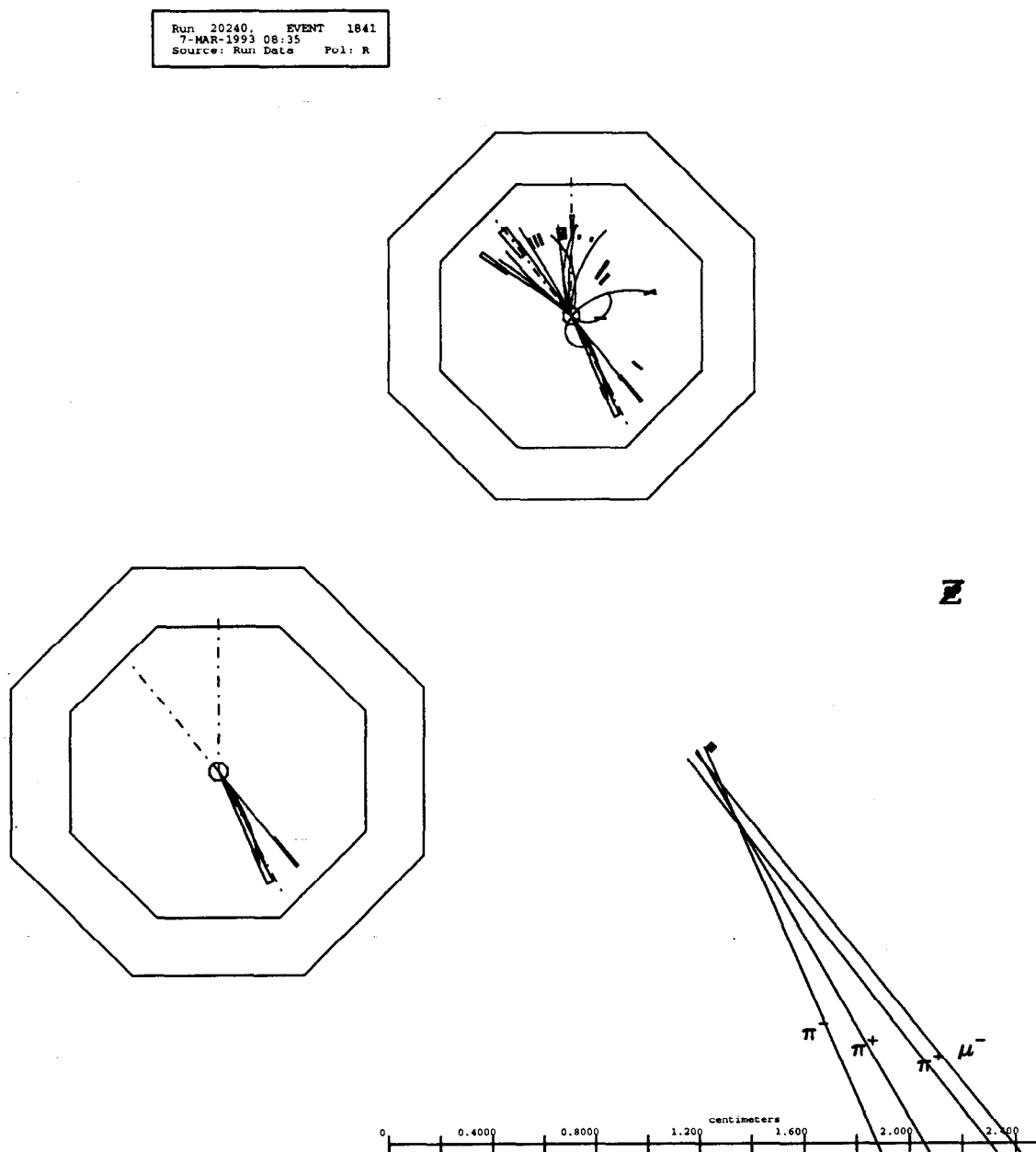
Figure 4.21: Three views of a B \rightarrow D\mu\bar{\nu}_\mu data event: the whole event, the isolated four B decay tracks and two clusters, and the four B tracks zoomed well inside the VXD2, showing the separate B and D vertices. Detector elements shown are the WIC and VXD2 only. The IP is shown in the zoomed-in display. Dashed lines are the (three, in this case) jet axes. The label \pi^\pm means \pi^\pm , K^\pm , etc. Note also that the tracks are extrapolated back far enough to determine their would-be crossing point with the IP, and are not terminated at the secondary vertex.
