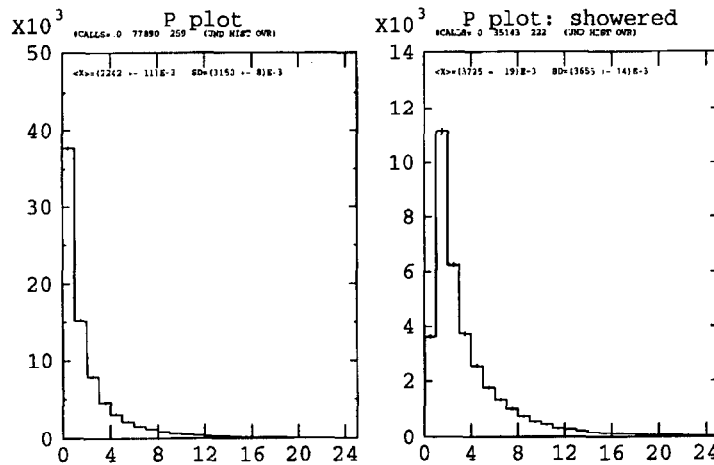
Figure 4.14: MC: |\vec{p}| (GeV/c) of all tracks, before and after the requirement that the particle showers in the LAC. This shows that particles of |\vec{p}| \lesssim 1 (GeV/c) rarely make it out to the LAC and shower.
