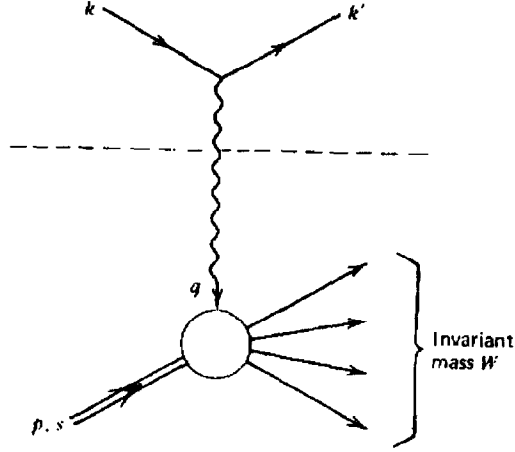
Figure 2.2: Deep Inelastic Scattering.
