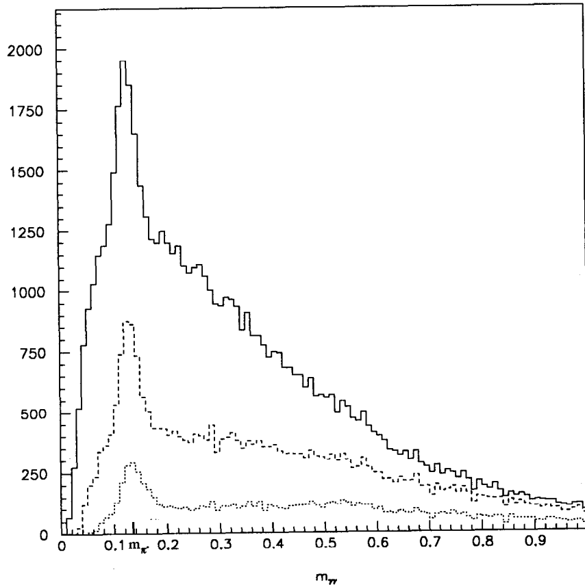
Figure 4.19: The invariant mass of pairs of photons, found and combined as explained in the text. This is 1993 data. The scale is in \text{GeV}/c^2 , and the mass of the \pi^0 is indicated. \frac{\epsilon}{\mu} = 0.67 to get the peaks to fall at m_{\pi^0} . The solid line requires that the energy ( mip scale) of each photon, E_{cl,2} , is greater than 100 MeV, the dashed line requires E_{cl,2} > 400 MeV and the dotted line requires E_{cl,2} > 700 MeV.
