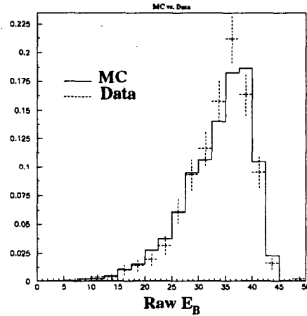
Figure 5.7: MC/Data: Reconstructed E_B for MC and Data. No background, unfolding or acceptance correction has been made. There's no reason these should necessarily agree.
