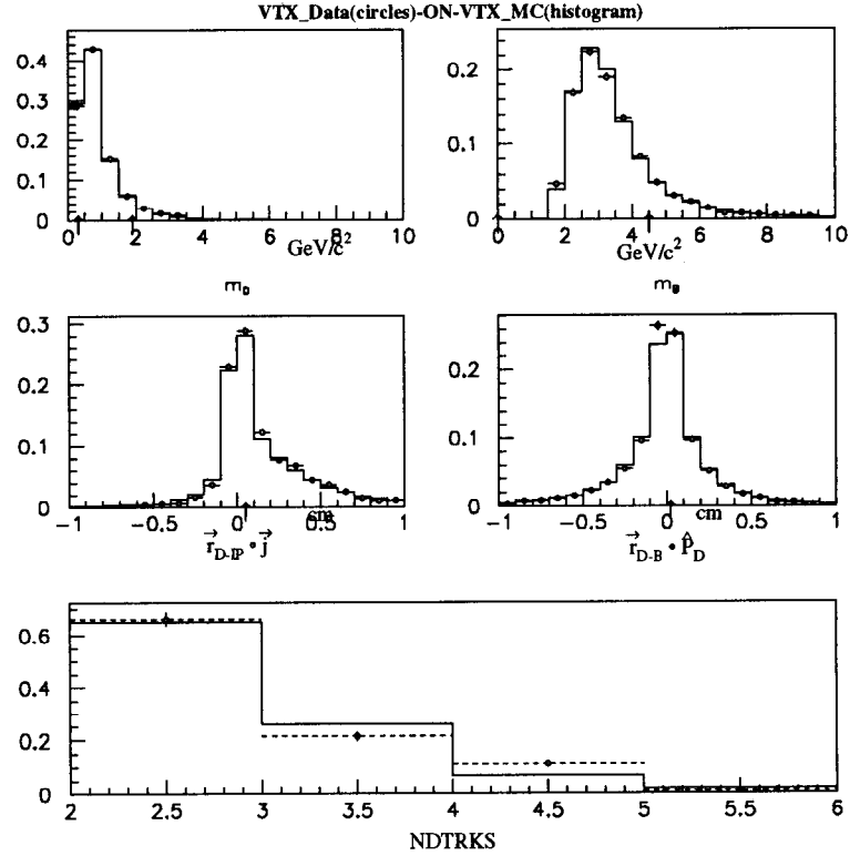
Figure 4.4: Data-MC comparison of four of the vertexing quantities – before cuts – in figure 4.3. At the bottom is the post-cuts number of prongs, NDTRKS.
