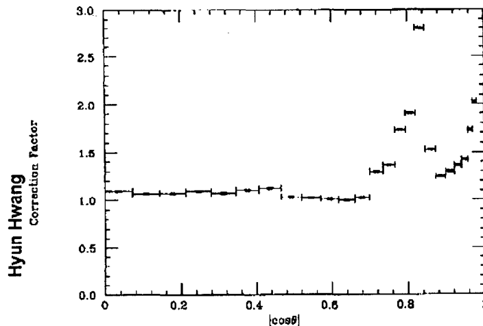
Figure 4.18: The amount by which we multiply the cluster energy as a function of its |\cos \theta| for hadronic clusters. The bin sizes are chosen to match LAC tower boundaries.
