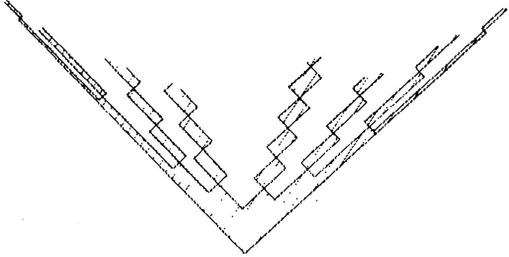
Figure 2.12: String model fragmentation showing production of q\bar{q} pairs. Shaded areas are regions of non-zero color force.
