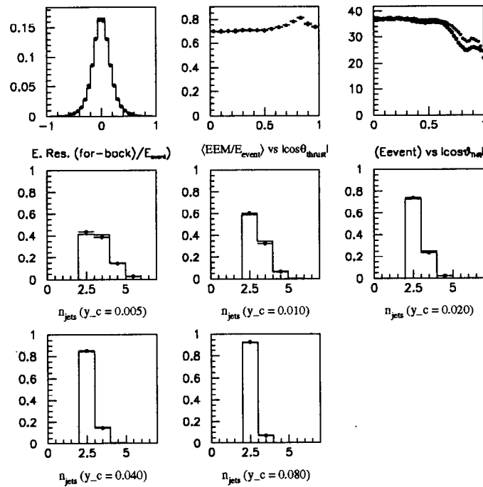
Figure 3.30: MC/data: Calorimeter event quantities II. Shown are the event Forward-Backward energy asymmetry, EM energy fraction vs. \cos \theta_{thrust} (note the peak where the hadron calorimeter is largely absent), E_{event} vs. \cos \theta_{thrust} , and the number of jets in the event for the Durham algorithm and y_c as labeled. All plots normalized to 1 entry, except \langle EEM/E_{Event} \rangle vs. \cos \theta_{thrust} and E_{event} vs. \cos \theta_{thrust} .
