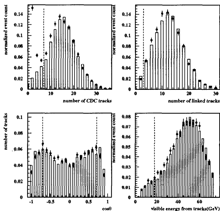
Figure 3.28: MC/data: Track multiplicity [83]. There is a 3% difference between data and MC in the mean in the upper left plot. "Linked tracks" means number of tracks in the CDC that are linked to tracks in VXD2. MC is the histogram; data are the points.
