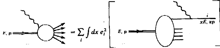
Figure 2.3: Deep Inelastic Scattering: the parton view.
