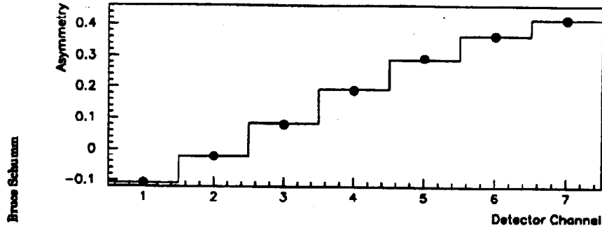
Figure 3.9: The measured energy-dependent Compton asymmetry function (see text) vs. the predicted shape.
