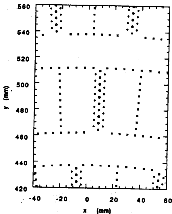
Figure 3.16: The points where the CDC wires attach to the ends of the CDC. One can see the structure of the super-layers and cells within them. The wires are of four types: high voltage field-shaping wires (crosses), guard wires (diamonds), signal, or sense wires (open circles) and dummy sense wires (squares).
