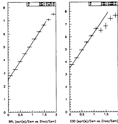
Figure 4.20: Extraction of \frac{\epsilon}{\pi} . BRL(EDC) means the thrust angle is well-contained in the barrel(endcap) LAC. Notice that the last 2(4) points are omitted from the fit. One can check that it is extremely rare ( \approx 2\% of good clusters) that the ratio of hadronic energy to electromagnetic energy in a given cluster is as large as 1.5.
