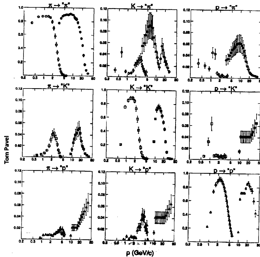
Figure 3.14: \pi^+ , p , K^+ (and their anti-particles) Monte Carlo (mis-)identification efficiency. Note that the plots on the diagonal are the correctly ID'd particles, and the maximum value on their y-axes (1.0) is an order of magnitude larger than that on the off-diagonal plots – the incorrectly identified particles. Also note the interruption in each plot in the two curves: in the lower (higher) momentum range the liquid (gas) radiator is used.
