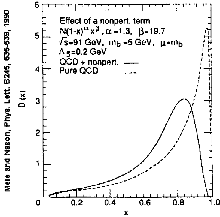
Figure 2.9: Pure pQCD calculation of the fragmentation function accurate to NNLO (dashed curve) and calculation with ad-hoc non-perturbative convolution (solid curve).
