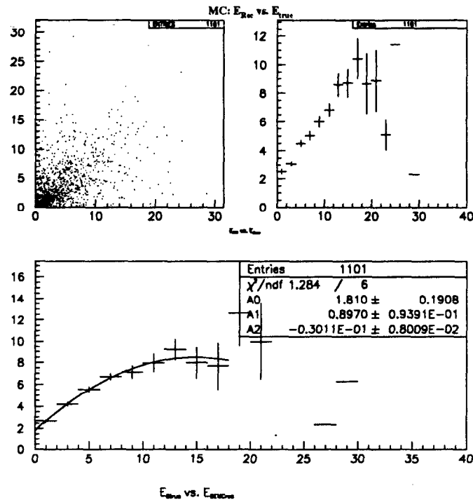
Figure 5.4: MC: The top row is reconstructed vs. true total neutral fragmentation energy, defined as in the text. The plot in the second column is the binned version of the scatter plot in the first column, as before. The bottom plot just has the x- and y-axes switched with respect to the top plot, and is fit with a 2 nd order polynomial. This, finally, is what is used to get the neutral contribution to the fragmentation energy. The systematic error on finding the neutral fragmentation energy comes from varying the parameters of the fit by the errors on them coming from MINUIT [96].
