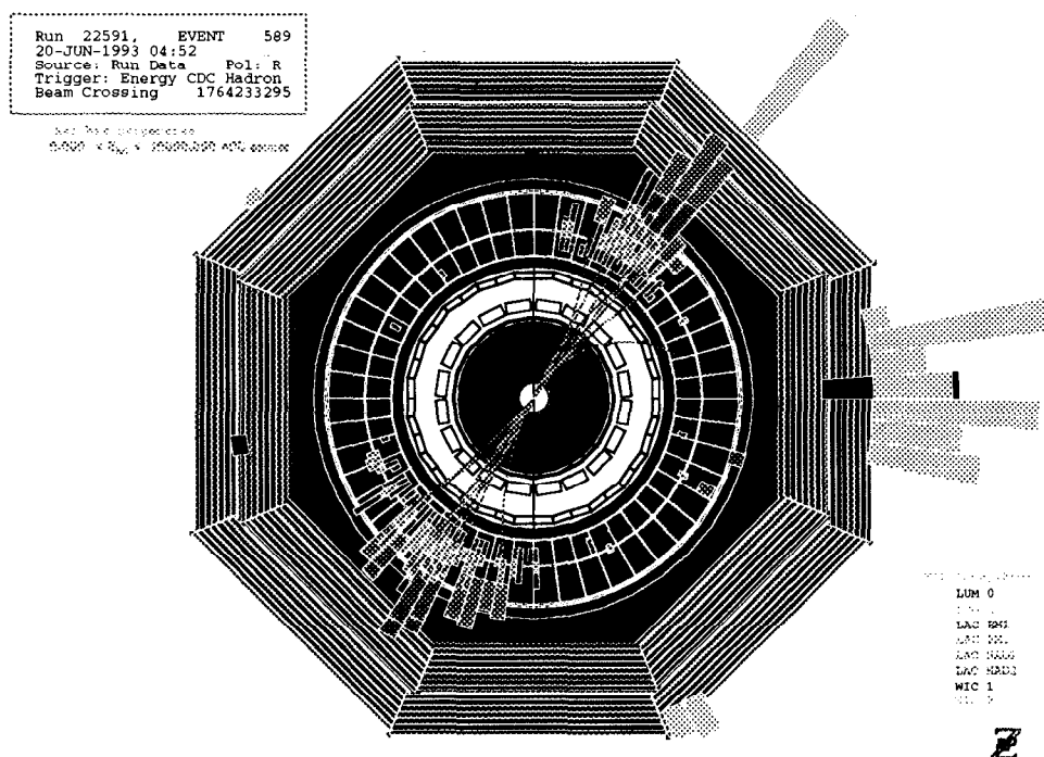
Figure 4.10: A typical 2-jet event, showing tracks and clusters and all detector sub-systems. Cluster sizes are in logarithmic proportion to the energy in them.
