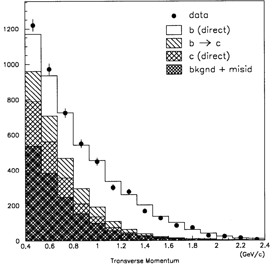
Figure 4.6: Plot [89] of underlying event flavor as a function of a lepton's p_{\perp} with respect to the closest jet – for |\vec{p}| > 4.0 GeV/c. One sees from this that at large p_{\perp} the leptons are mainly “direct,” i.e. b \rightarrow c l \nu_l .
