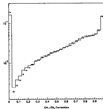
Figure 3.32: MC/data: Kal cluster quantity G_c .
