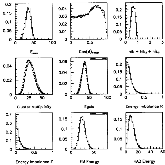
Figure 3.29: MC/data: Calorimeter event quantities I. Shown are E_{event} , |\cos \theta_{thrust}| , hiE + hiE_2 + hiE_3 (the sum of the 3 highest scaled cluster energies in each event), n_{clus} , E_{gcls} (energy sum in “good” clusters in an event), Energy Imbalance (the scaled missing momentum vector for both R and Z components) and the event energy in the EM and HAD sections. MC is the histogram; data are the points. All plots normalized to 1 entry.
