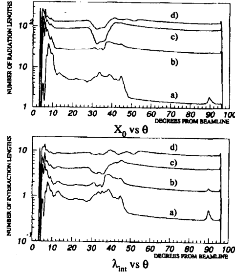
Figure 3.18: Material thicknesses (measured in units of radiation lengths, X_0 , and strong interaction lengths, \lambda ) in front of various sections of the Calorimeter. a), b), c), d) is just inside EM1, EM2, HAD1, HAD2, respectively.]
