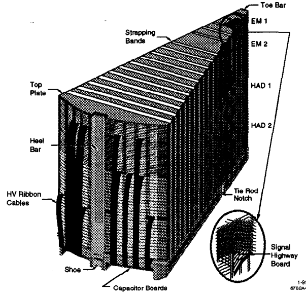
Figure 3.20: A LAC endcap module.
