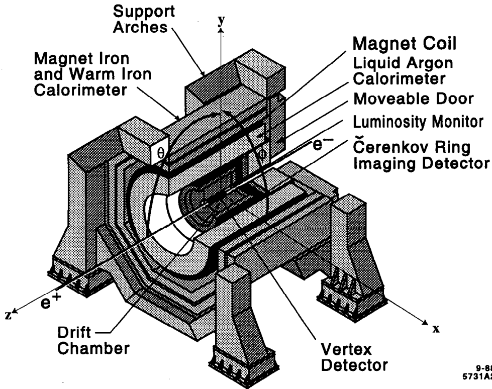
Figure 3.6: The Stanford Linear Collider Large Detector – Cut-away view.
