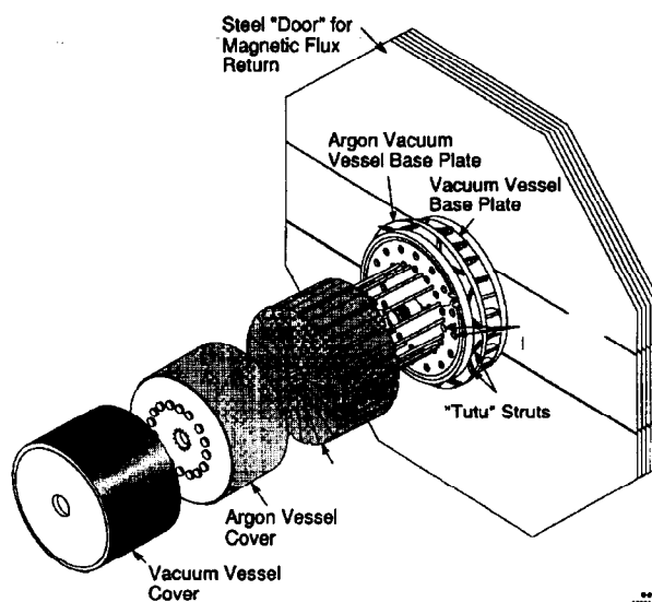
Figure 3.22: LAC endcap, showing the placement of one endcap module.
