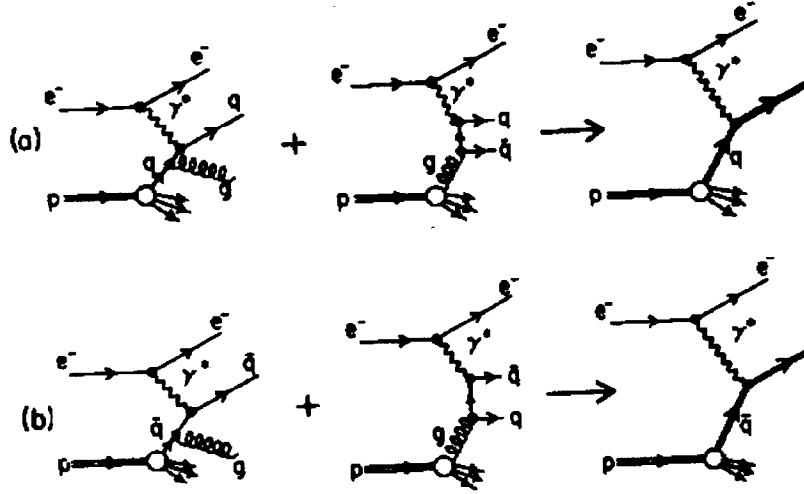
Figure 2.4: Deep Inelastic Scattering: QCD effects. The “Compton” gluon diagrams are the second in each of the lines (a) and (b) above.
