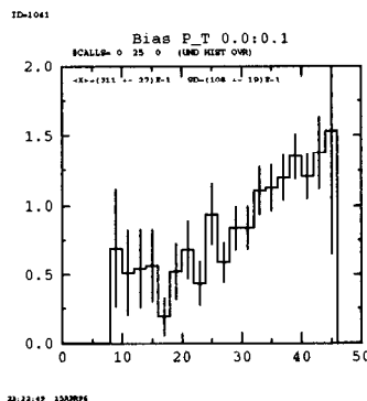
Figure 4.8: This is the normalized, binned MC E_B before vertex cuts divided by the same quantity bin-by-bin post-vertex cuts. There is no minimum lepton p_\perp cut. (The ratty statistics here are due to the fact that this plot comes from an analysis of only about \frac{1}{5} of the MC. The trend remains when the plot includes all the MC.) This shows the vertexing by itself selects preferentially high energy B hadrons. This will be accounted for with an acceptance correction.
