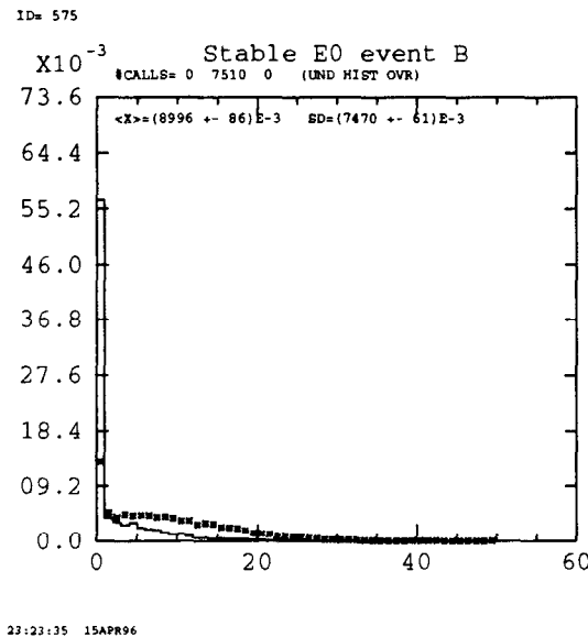
Figure 5.1: MC: E_0 in s.l. B hadrons and all B hadrons. The stars are the all-B sample, and the histogram is the s.l. B hadrons, showing the relative lack of neutral energy in s.l. B decays. The histograms are normalized to the same area.
