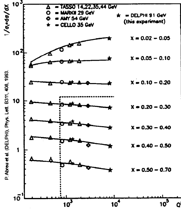
Figure 2.7: GLAP scaling violation in fragmentation. Compare to figure 2.5. 1/\sigma_t \cdot d\sigma/dX is the total, normalized, charged, hadronic cross-section. It contains all the quark fragmentation functions. See equation 2.11 for the lowest order in \alpha_s expression for this quantity. The higher-order-in- \alpha_s terms cause these curves to bend, in the way shown here, with Q^2 .
