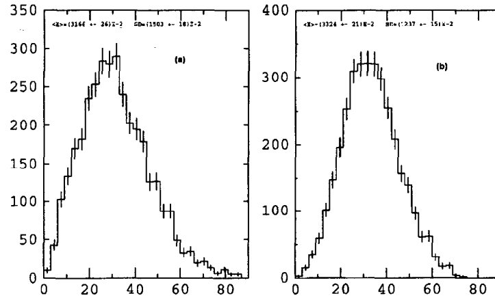
Figure 4.17: MC: (a) The Monte Carlo true E_{Neu} and (b) the reconstructed E_{Neu} , according to the algorithm described.
