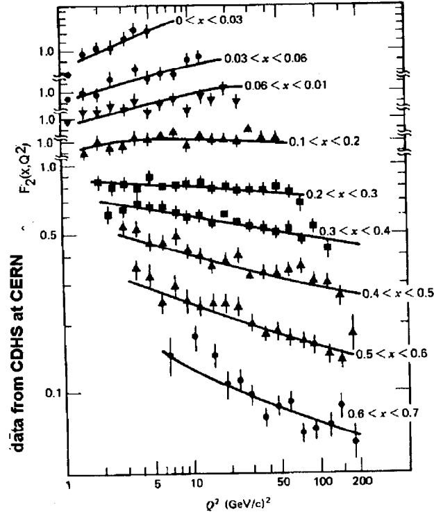
Figure 2.5: GLAP scaling violation in DIS, as reprinted from reference [33].
