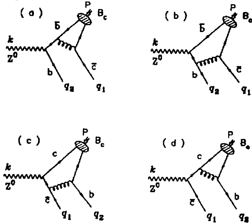
Figure 2.10: Braaten/Cheung/Yiu fragmentation model. Shown are the leading order-in- \alpha_s diagrams to produce a heavy-heavy meson, here a B_c . This model is proposed to be used also in the production of light-heavy mesons – the type commonly created in e^+e^- annihilation.
