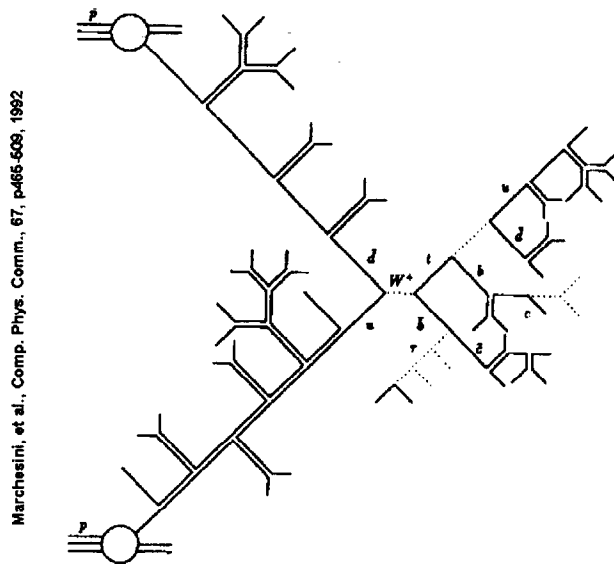
Figure 3.25: HERWIG color connection in a p\bar{p} event.
