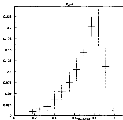
Figure 5.8: Data: Final E_B spectrum. The solid lines are statistical errors, the dashed includes systematic errors as well.
