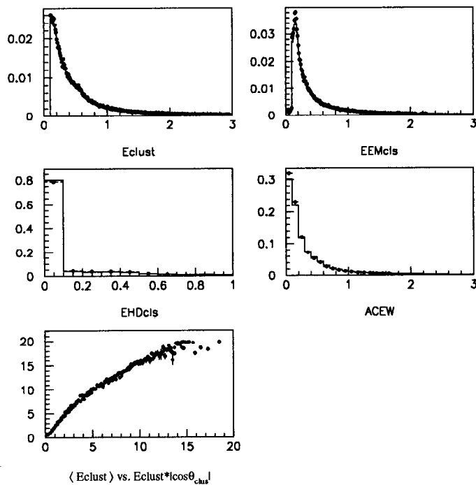
Figure 3.31: MC/data: Calorimeter clusters. Shown are E_{clus} , E_{clus_{EM}} , E_{clus_{HAD}} , E_{clus} \cdot |\cos \theta_{clus}| , and E_{clus} vs. E_{clus} \cdot |\cos \theta_{clus}| . MC is the histogram; data are the points. Top four plots normalized to 1 entry.
