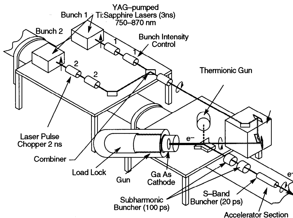
Figure 3.4: The SLC electron source.
