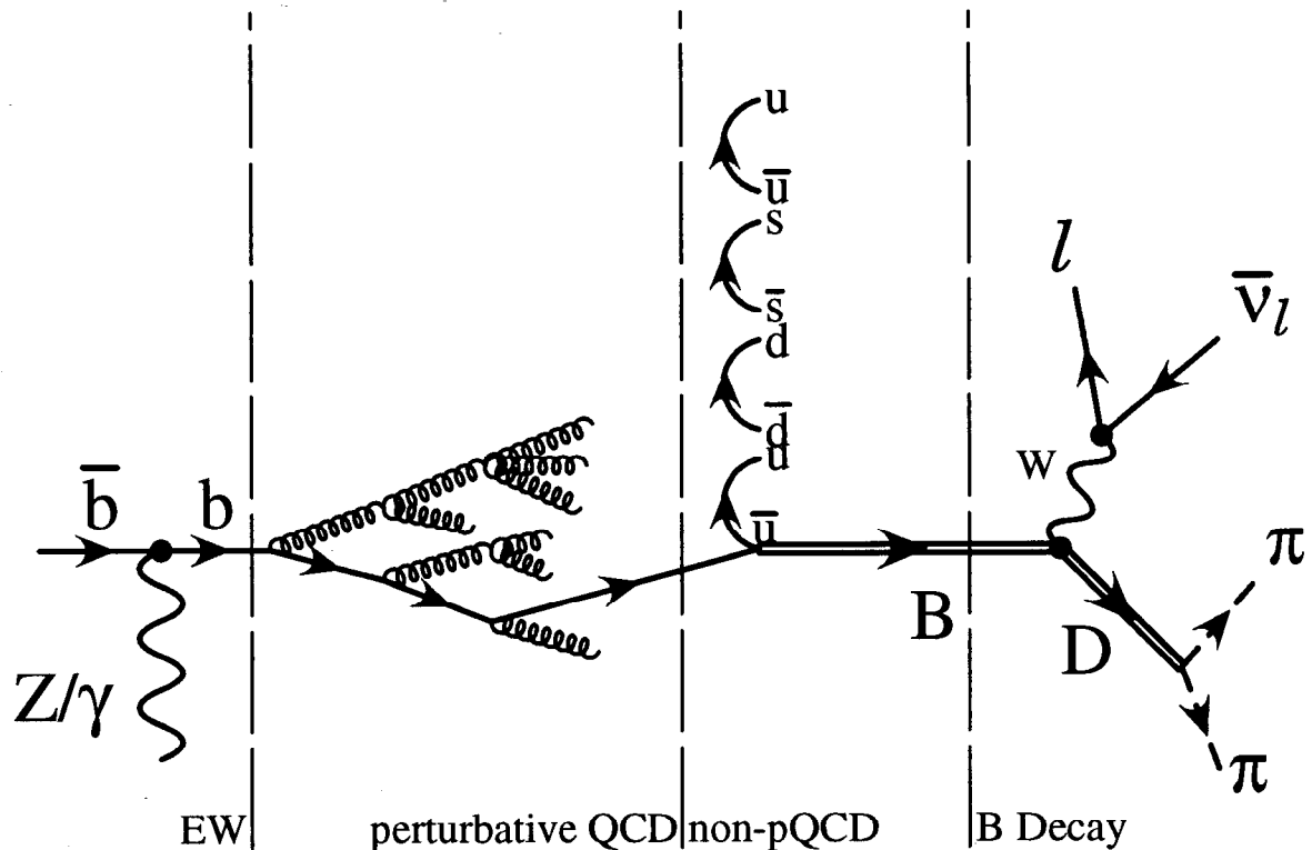
Figure 4.1: The topology under study, showing the various stages of the process. The D \rightarrow \pi\pi is symbolic of any 2-prong seed vertex. Extra tracks may be added to the vertex in the way described in the text. The \pi may in fact be a K ; for the energies of the tracks which form a vertex ( \gtrsim 1.5 GeV) the error made by assuming m_{\pi^\pm} is negligible.
