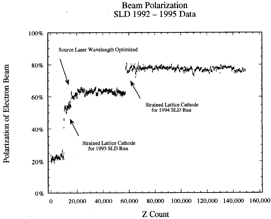
Figure 3.3: The time history of the e^- polarization from 1992 through 1995.
