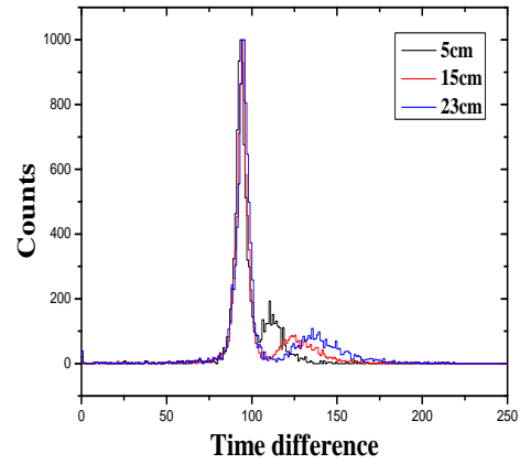
FIG. 1: The TOF spectrum with ^{252}\text{Cf} source with 3PB detector at distances 5 cm (black color), 15 cm (red color) and 23 cm (blue color) respectively from the source position. Here, we do not use any energy gate. The prompt gamma and delayed neutron bunches are separated nicely with the digitizer set up. As the distance of the stop detector increases, the neutron bunch is separated more clearly in TOF spectrum.
