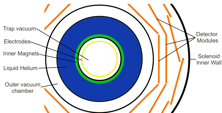
Figure 2.8: A schematic cross-section of the apparatus core showing the two vacuum chambers and the liquid helium volume.
