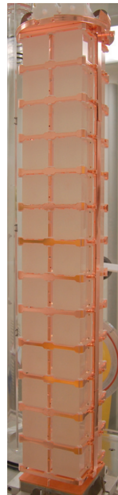
Fig. 1. The CUORE-0 detector.
