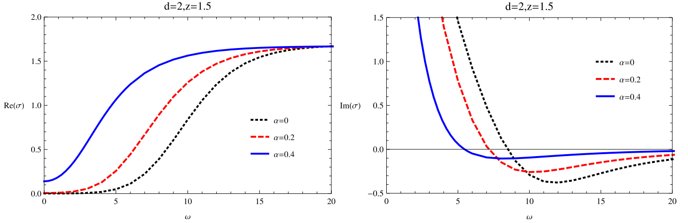
Fig. 5. The conductivity at T/T_c = 0.25 with d = 2 and z = 1.5 for \alpha = 0, 0.2 and 0.4 .
