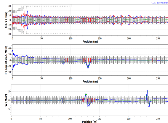
Figure 2: Beam envelopes (4σ, multiparticle tracking) with several failures compensations.
