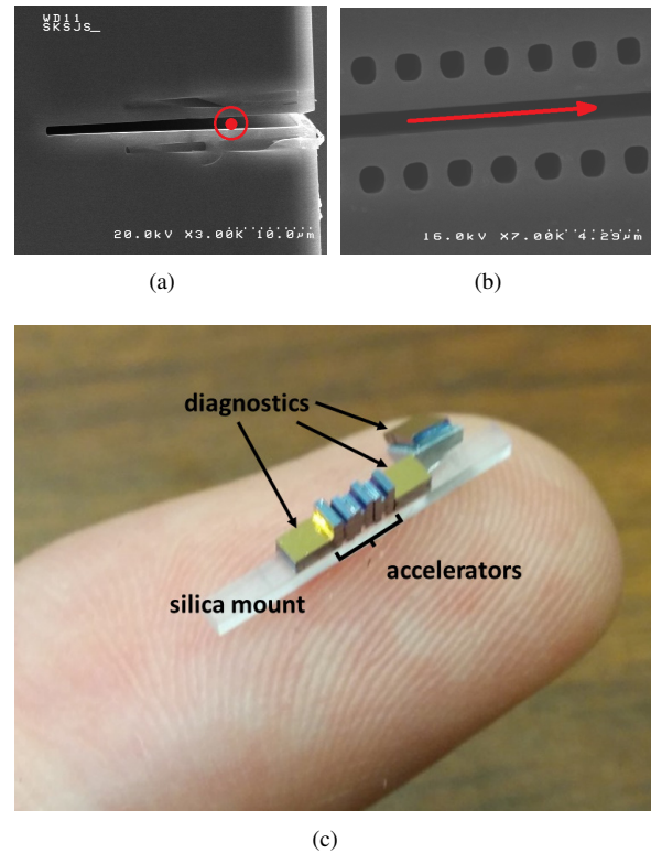
Figure 2: Views of fabricated accelerator structures before hydrogen annealing, red markers indicates axis of electron travel: (a) view from upstream, electrons travel through the vacuum gap in the center (b) top view onto the surface of a etched buried grating (c) three accelerator samples mounted on glass substrate for testing with diagnostic structures for alignment and timing.
