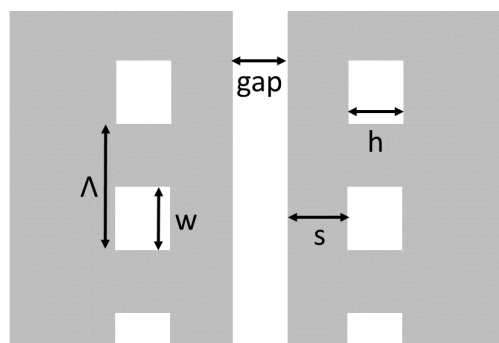
Figure 1: Illustration of parameters used in the design and simulation of buried grating structures.
