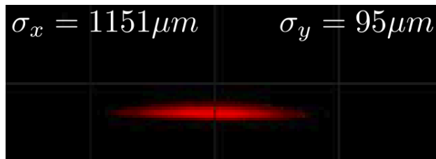
Figure 1: Electron beam profile as measured at the SLM, for a current of 500 mA stored in 100 bunches, after setting the Crab-Waist Sextupoles at 1/3 of the nominal strength. The beam vertical size is at the level of the diagnostics resolution.
