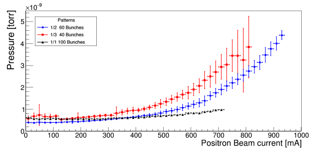
Figure 2: Positron ring vacuum rise as a function of the stored current for different bunch patterns. Each series represent the average (markers) and RMS (bars) over several hours of running.
