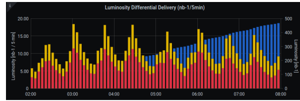
Figure 5: Luminosity (differential and integrated) during 6hr of SIDDHARTA-2 pilot run.
