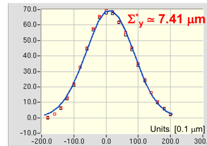
Figure 6: Vertical beam-beam luminosity scan.
