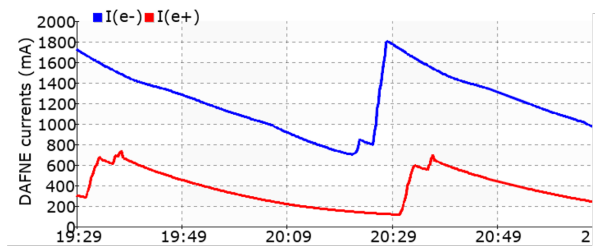
Figure 3: Maximum electron (blue) and positron (red) beam currents stored so far in the DAΦNE main rings.
