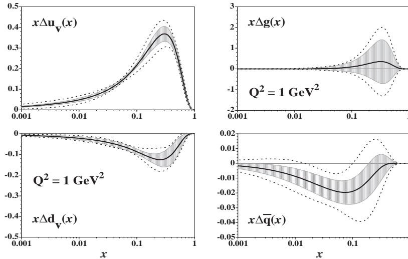
Figure 1. Polarized PDFs and their uncertainties are shown at Q^2=1 \text{ GeV}^2 . The solid curves and shaded areas indicate the AAC03 distributions and uncertainties. The dashed curves indicate the uncertainties of the previous version AAC00.
