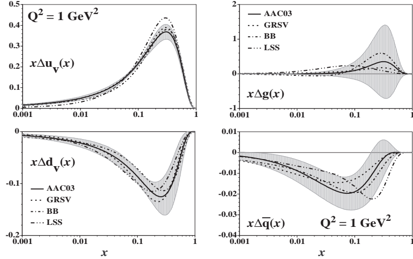
Figure 2. The polarized PDFs are compared with other parametrizations at Q^2=1 \text{ GeV}^2 .
