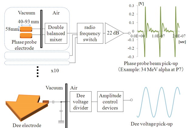
Figure 3: The block diagram of the phase probe and dee voltage pickup.
