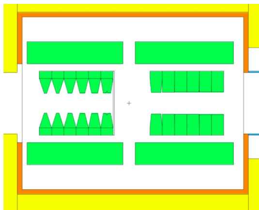
Figure 2: Cross section in the XZ-plane (top view) of the KHE2 (left) and KHE3 collimators. The beam enters from the left. The complex teeth structure of KHE2 is clearly visible.
