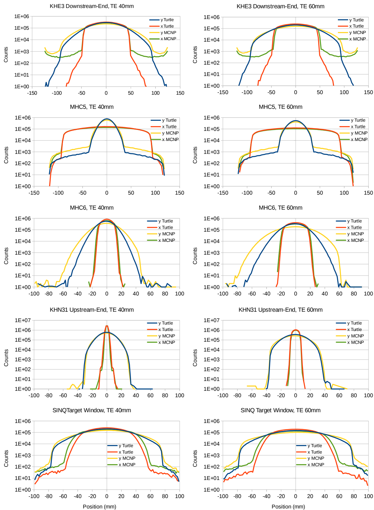
Figure 3: Proton beam distributions for TE40 and TE60 along the SINQ beam line obtained with pure Turtle as well as combined Turtle/MCNPX (MCNP in the legend) simulations.
