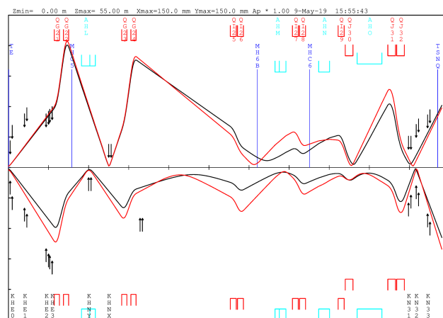
Figure 1: Beam envelope fit between TE and SINQ.
