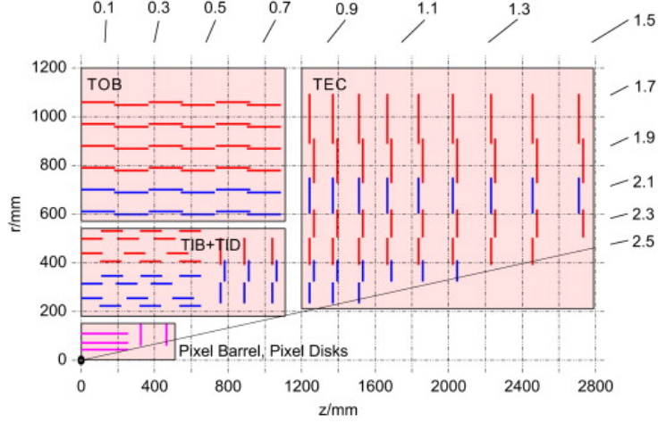
Figure 1.14 – Structure of the CMS tracker system. View in one quadrant of the z-r plane. From inside to outside, the pixel detector (barrel and end-cap), the TIB and TID the the TOB in the barrel region while the TEC compose the endcap region.
