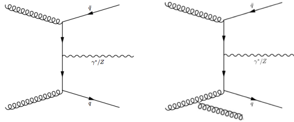
Figure 3.29 – Representation on one of the production modes of Zb\bar{b} events with or without extra-radiations. Left: Production diagram for the selected Zb\bar{b} final state without extra jets. Right: Production diagram for the selected Zb\bar{b} final state with extra jets, Zbx and Zbx+\text{jets} final states.
