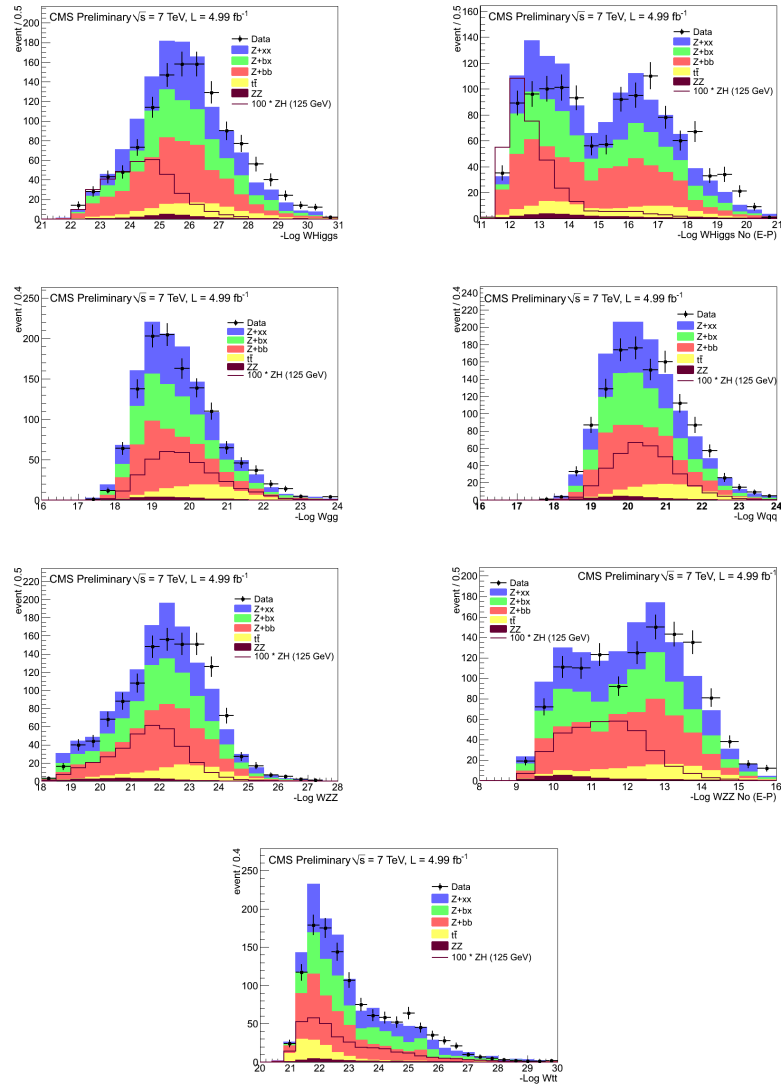
Figure B.4 – Comparison of Data-MC at 5.0 \text{ fb}^{-1} of the Matrix Element weights distribution for the seven hypothesis of the ZH analysis. Dielectron channel at Z(\ell\ell)H(b\bar{b}) Medium-Loose working point.
