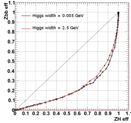
Figure 3.20 – Comparison between the Zbb vs ZH efficiency curves for the Matrix Element Higgs weight estimated assuming the E-P conservation and two different Higgs width. Similar performances are observed.
