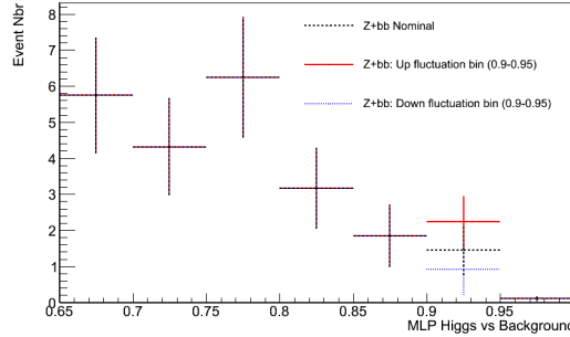
Figure 3.33 – Illustration of a the shape fluctuation considered to take into account the statistic uncertainty due to the available number of simulated event. It shows the asymmetric up and down fluctuation for the bin (0.9 - 0.95) for the Z+bb processes. The distribution stay un-changed for the other bin.
