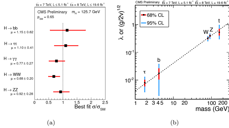
Figure 1.9 – (a): Values of production cross section times the relevant branching fractions \sigma/\sigma_{SM} for the combination (solid vertical line). The vertical band shows the overall uncertainty. The horizontal bars indicate the \pm 1 standard deviation uncertainties for the individual modes. [39]. – (b) Fits for the deviation to the Standard Model prediction of the coupling between Higgs boson and fermions/vector bosons. For the fermions it is the values of the fitted Yukawa couplings while for vector bosons it is the square-root of the coupling divided by twice the vacuum expectation value [39].
