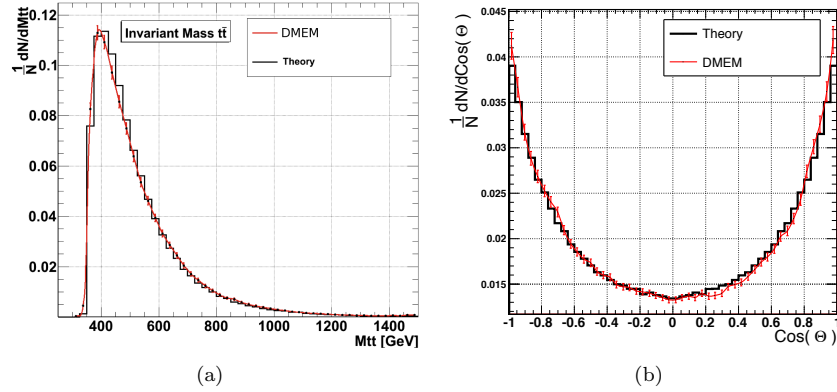
Figure 2.20 – -a) M_{t\bar{t}} normalized differential cross section.-b) \cos\theta^* normalized differential cross section. Both are produced with 10000 top quark pair events decaying in fully leptonic channel. The theoretical curve are the expected one at tree-level when neither ISR and UE are taken into account. The DMEM is used on fully simulated events.
