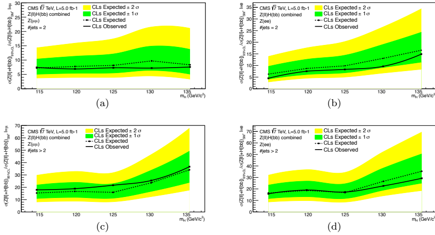
Figure 3.34 – Expected and observed 95% upper limits on the ratio of Standard Model production of Z(l\bar{l})Hb\bar{b} for the Matrix Element method analysis. (a) Z(\mu\mu) in the two jet category. (b) Z(ee) in the two jet category. (c) Z(\mu\mu) in the more than two jet category. (d) Z(ee) in the more than two jet category.
