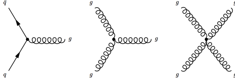
Figure 1.2 – Representation of the different QCD coupling, between quarks and gluons and between gluons themselves.
