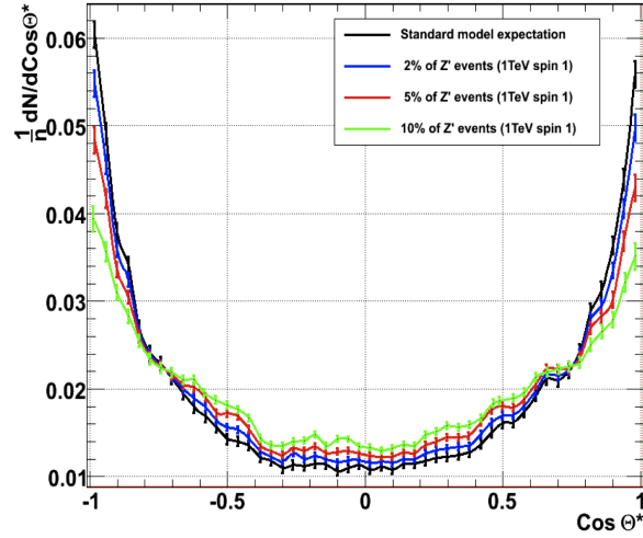
Figure 2.22 – Distribution of the diffusion angle of the top quark, \cos \theta^* emission reconstructed by the Differential Matrix Element method. Variable represented for events with DMEM reconstructed M_{t\bar{t}} that peak above 700 GeV for several sample containing different fraction of new physics event ( Z' \rightarrow t\bar{t} ).
