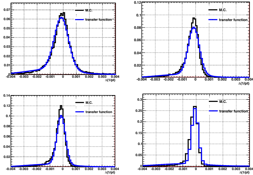
Figure 3.8 – Projection of \delta \frac{1}{P_t} = \frac{1}{P_t} - \frac{1}{P_{t^{vis}}} for different range in P_t for muons. The black curve shows the distribution obtained from the difference between the generated and the reconstructed inverse transverse momenta. The blue (continuous) curve corresponds to the transfer function. The curves are normalized to unity.
