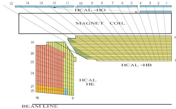
Figure 1.16 – Representative view of a quadrant of the hadronic calorimeter [59]. in the z - y plan.
