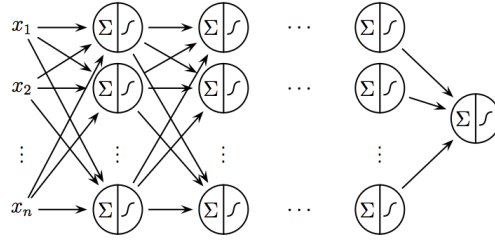
Figure 3.11 – Schematic representaion of the structure of a multilayer perceptron. There are n input variables ( x_i ), several layer composed of various number of nodes characterized by a sigmoid function applied on its input. Each of the node is linked to all the node of the previous and the following layer and each link is characterized by a weight. Finally that converge to the output variable.
