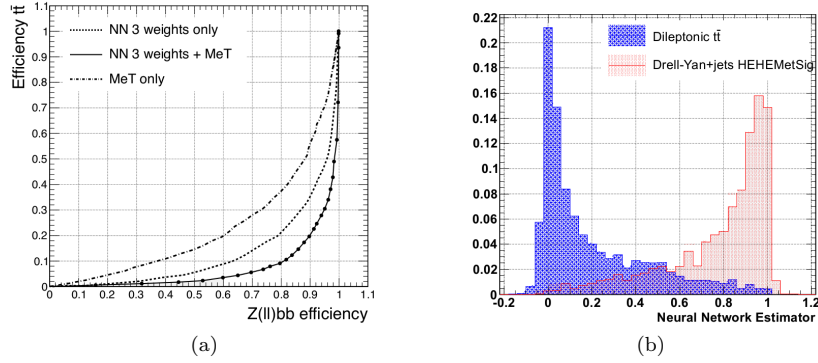
Figure 3.13 – Left: Z(l\bar{l})b\bar{b} versus t\bar{t} selection efficiencies estimated according to three quantities which are: the E_T^{miss} distribution, a neural network that uses the matrix element weights and the E_T^{miss} and one NN based on the matrix element weights only. - Right: Neural network discriminant, using the matrix element weight, for t\bar{t} and D-Y sample. Both sample are normalized to 1.
