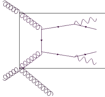
Figure 2.16 – Example of a t\bar{t} process with one initial state radiation. The reduced event is represented by the diagram inside the box. The ISR boost correction is equal to the P_t of the extra radiation or can be deduced from the reduced event.
