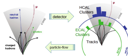
Figure 1.18 – Schematic representaion of the Particle flow object by comparison to the detector level. Particle flow particle candidates are constructed using information of several subdetector systems. [66]
