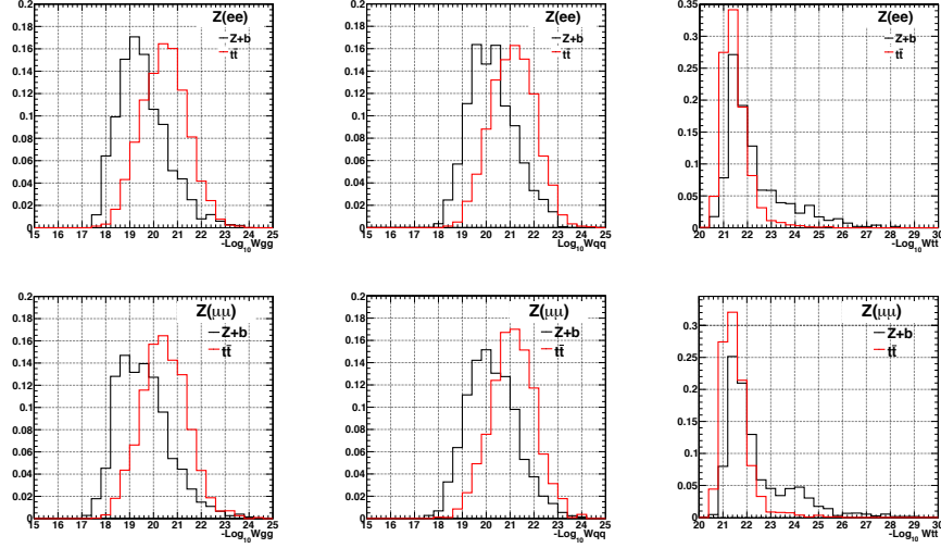
Figure 3.9 – Distribution of the -\text{Log}_{10} of the weights for Drell-Yan and t\bar{t} events in the dielectron channel. - Top Left: gq \rightarrow Z(e^+e^-)b\bar{b} hypothesis. - Middle top: qq \rightarrow Z(e^+e^-)b\bar{b} hypothesis. For these two matrix elements the correction for the transverse boost is evaluated only with the visible particles. - Top Right : t\bar{t} hypothesis, the boost correction uses the missing transverse energy information. Bottom plots represent the same discrimination in the dimuon channel.
