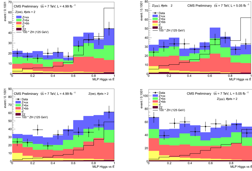
Figure B.2 – Comparison of Data-MC at 5.0 \text{ fb}^{-1} of the neural network discriminant between Z(\text{ll})H(b\bar{b}) and t\bar{t} . Top: 2 jets category, Bottom: More than 2 jets category. Left: Dielectron channel, Right: Dimuon channel.
