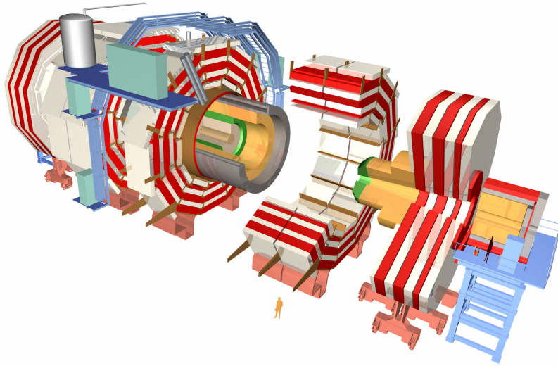
Figure 1.13 – Schematic representation of the CMS detector [1]. Starting from the interaction point, the detector is composed of; the pixel tracker system, the silicon strip tracker, the electromagnetic calorimeter, the hadronic calorimeter, the magnet solenoid and then in the magnet yoke structure, the muon chamber.
