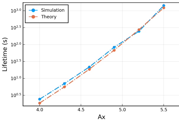
Figure 3: Comparison of the 1-d quantum lifetime between simulation and Piwinski's formula.
