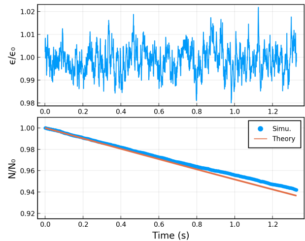
Figure 1: Evolution of beam emittance and particle number in the 1-d tracking ( A = 4.6 , \lambda = 100 \text{ s}^{-1} , \tau_{\text{theory}} = 18.6 \text{ s} ).
