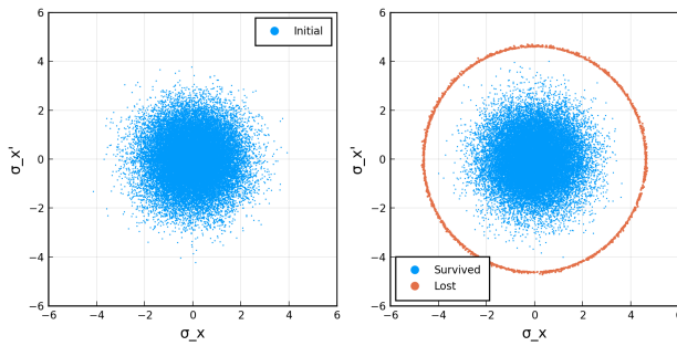
Figure 2: Beam distribution at the start (left) and the end (right) of simulation. The lost particles illustrate the aperture which is 4.6\sigma .
