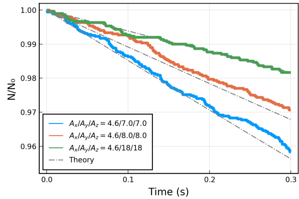
Figure 4: Simulation result of the particle loss with 3-d aperture, the dashed line is calculated by Eq.(10). The theoretical lifetime is 16.3 s, 9.2 s and 6.7 s, respectively ( \lambda_x = \lambda_y = \lambda_z = 100 \text{ s}^{-1} ).
